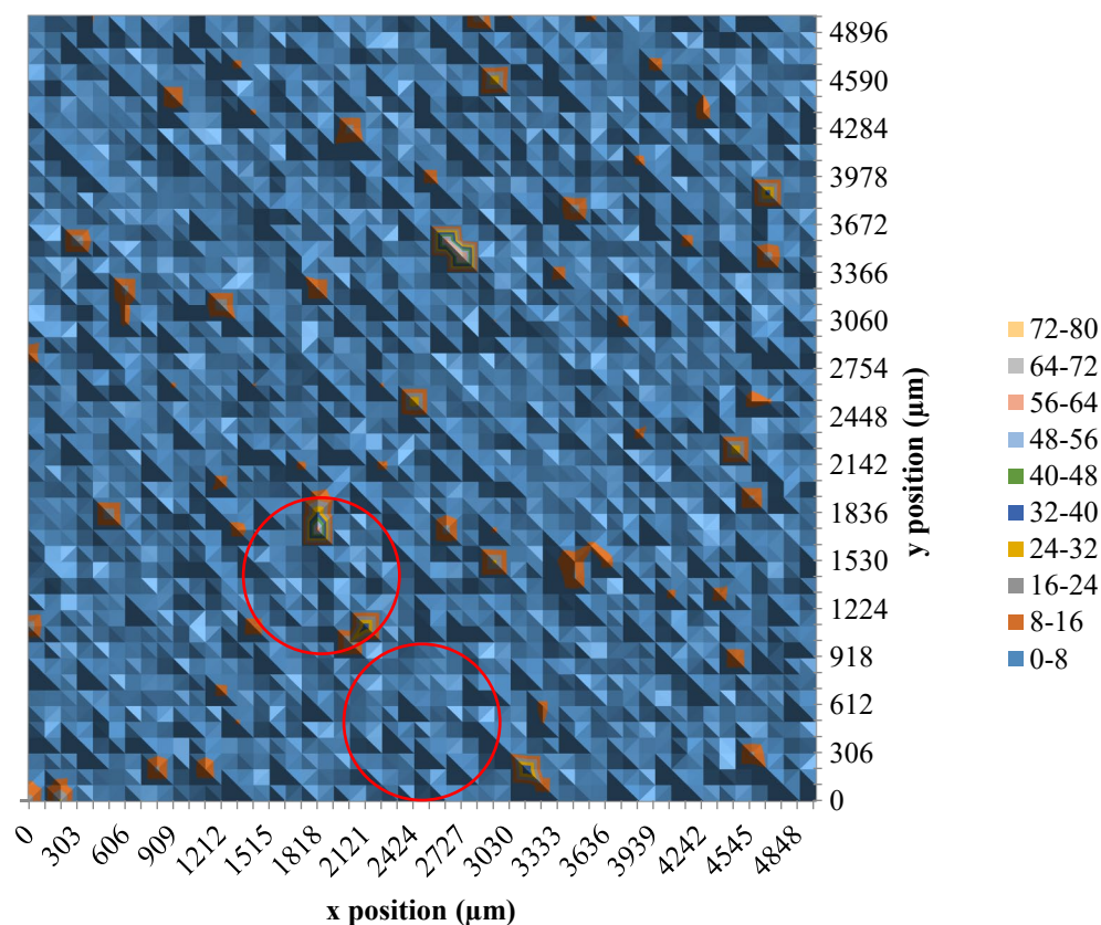
Fig. 10. Map of Ba L_3 - M_{4,5} count rates in the surface of a melt-pressed disk of SRM 2861 after cryogenic grinding to a fine powder. The red circles represent an X-ray beam from a 1 mm aperture aimed at two locations. Data were collected using a 0.05 mm spot size.
