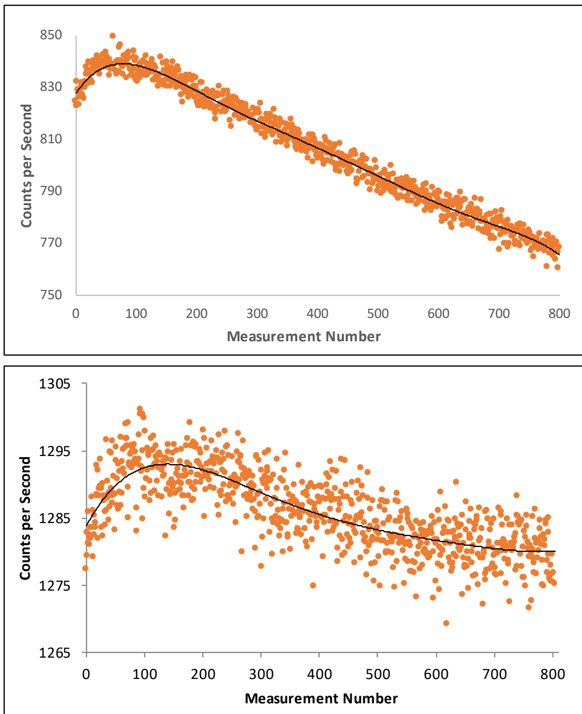
Fig. 15. Chlorine count rates as a function of exposure of a single location in the microXRF spectrometer. Top is SRM 2859; bottom is CRM 8123-a
