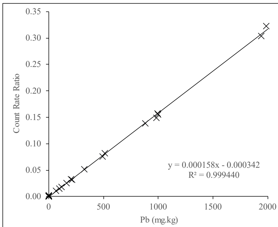
Fig. 11. Calibration graph for Pb L 3 -M 4,5 by WDXRF. The value R^2 is the correlation coefficient, used as a simple measure of goodness of fit.
