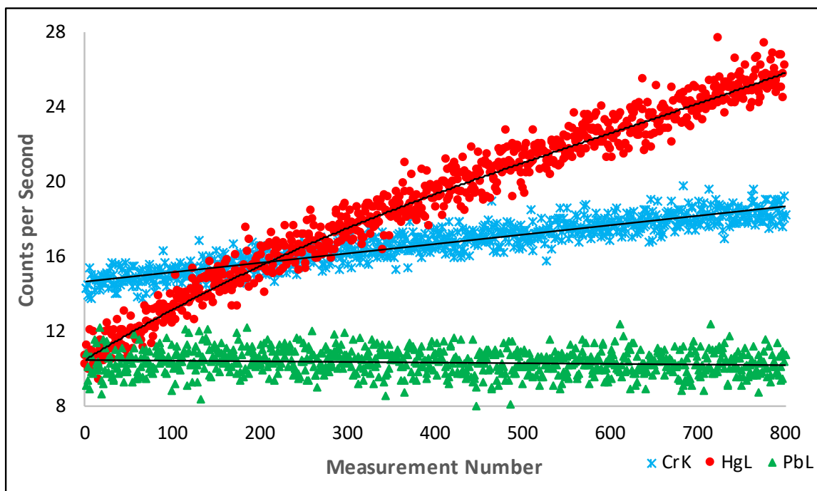
Fig. 14. Measured count rates for Cr, Hg and Pb from a single location (nominally 50 \mu\text{m} diameter) on one extruded pellet of SRM 2859. The measurements were acquired in 30 h. Black curves are meant only to show trends.
