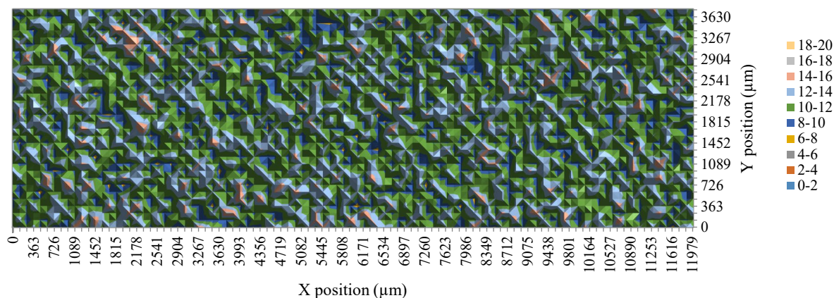
Fig. 9. Map of Hg L_3 - M_{4,5} count rates in the surface of a melt-pressed disk of SRM 2861. Data were collected using a 0.05 mm spot size.
