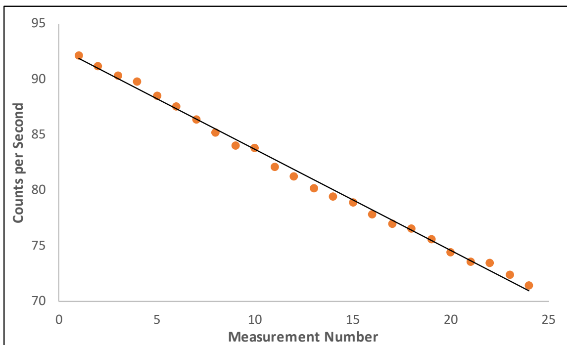
Fig. 17. Measured count rates for Cl in a melt-pressed disk of SRM 2859 at 1200 W generator power for 10 min per measurement.
