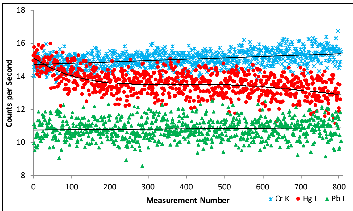
Fig. 13. Measured count rates for Cr, Hg and Pb from a single location (nominally 50 \mu\text{m} diameter) on a single extruded pellet of CRM 8123a. The measurements were acquired in 30 h.
