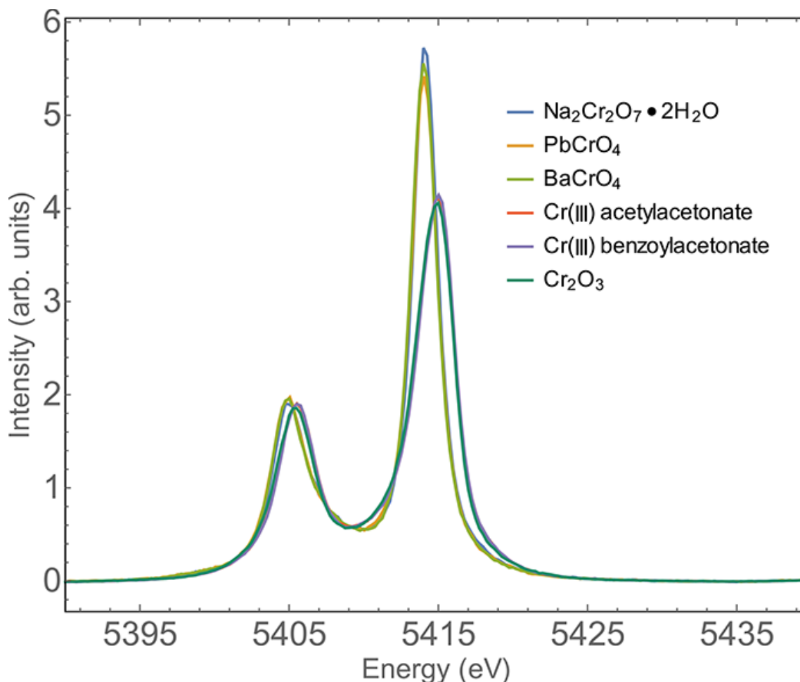
Fig. 21. Cr K-L 2,3 XES of selected trivalent and hexavalent reference Cr compounds after background correction and integral normalization. Note, the spectrum of Cr(III) acetylacetonate is nearly identical to that of Cr(III) benzoylacetonate and is hidden from view.
