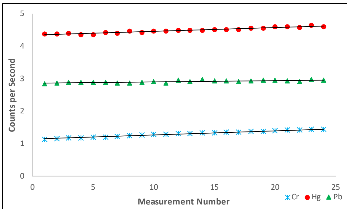
Fig. 16. Measured count rates for Cr, Hg and Pb from a single, melt-pressed disk of SRM 2859. The measurements were acquired in 4 h.
