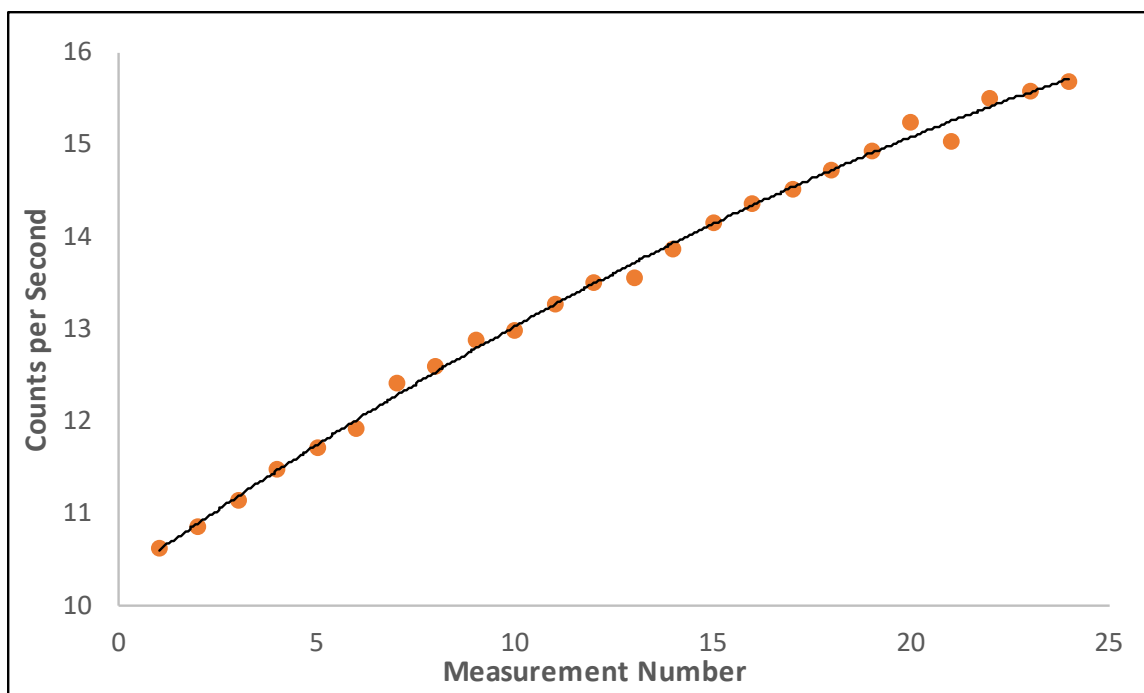
Fig. 18. Measured count rates for Ca in a melt-pressed disk of SRM 2859 at 1200 W generator power for 10 min per measurement.
