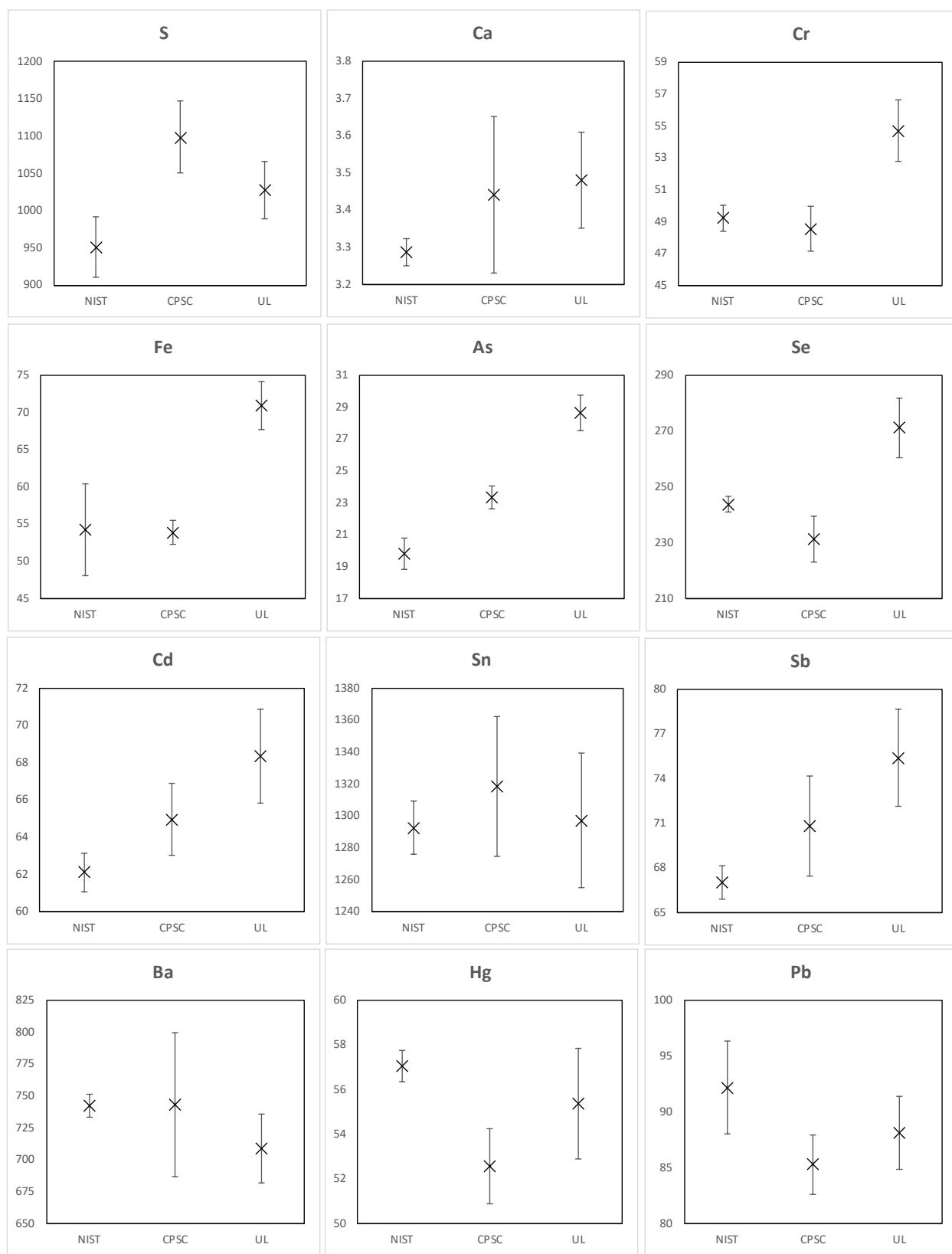
Fig. 20. Comparisons of mean results and expanded uncertainty estimates for elements found by collaborating labs in SRM 2861.
