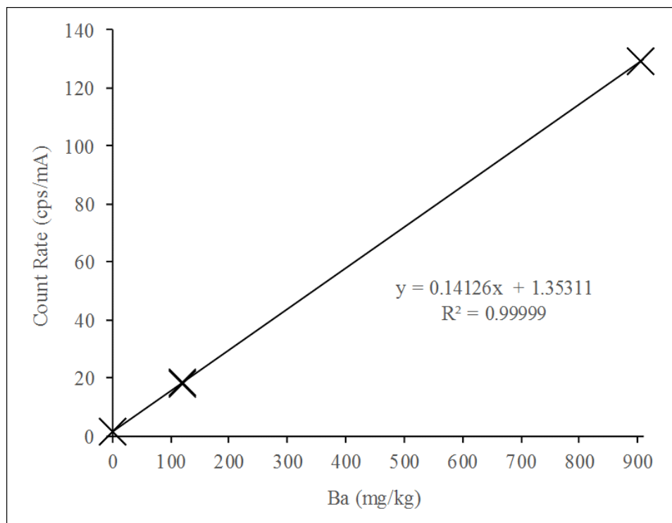
Fig. 12. Calibration graph for Ba K-L 2,3 by EDXRF. At each mass fraction, there are two measured points corresponding to the two faces of each calibrant disk in Table 29. The value R^2 is the correlation coefficient, used as a measure of goodness of fit.
