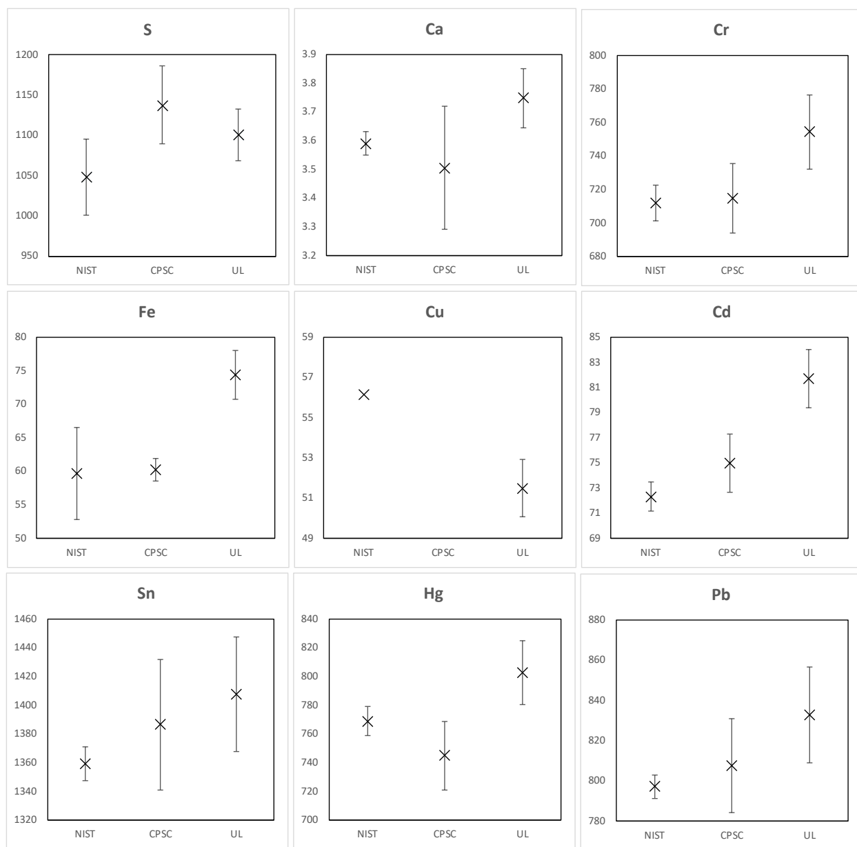
Fig. 19. Comparisons of mean results and expanded uncertainty estimates for elements found by collaborating labs in SRM 2859. Note, Cu by NIST is for information only, i.e. no uncertainty estimate was provided.
