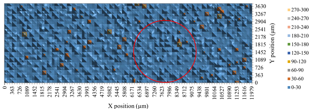
Fig. 7. Map of Ba L 3 -M 4,5 count rates in the surface of a melt-pressed disk of candidate SRM 2861. The red circle represents a 3 mm X-ray aperture of a handheld spectrometer.
