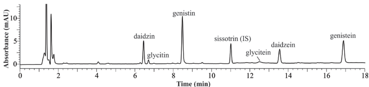
Figure 2. Chromatogram showing separation and detection of isoflavones in SRM 3238 using LC/absorbance. For this method, an Ascentis Express RP-Amide column (150 mm × 4.6 mm, 2.7 μm particle size; Supelco, Bellefonte, PA) was held at 35 °C. The separation was performed using a gradient consisting of 5 mmol/L ammonium acetate in water and acetonitrile. Absorbance detection was utilized at 254 nm.
