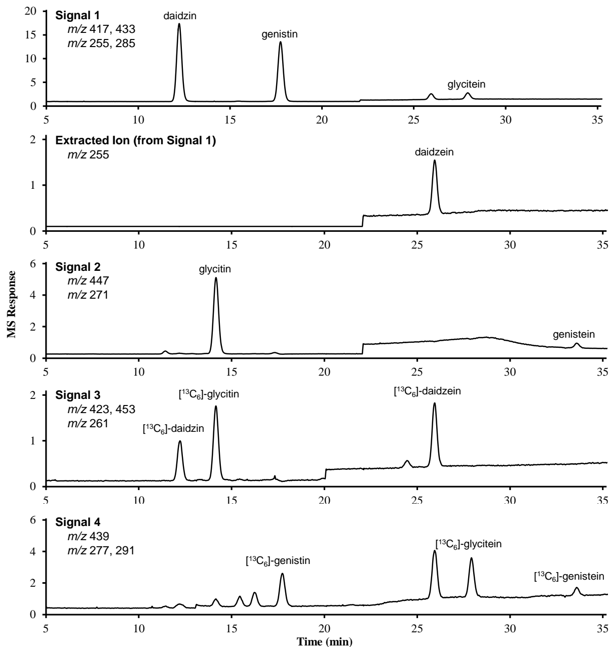
Figure 1. Chromatograms showing separation and detection of isoflavones in SRM 3238 using ID-LC/MS. For this method, a Zorbax SB-CN column (250 mm × 4.6 mm, 5 μm particle size; Agilent Technologies, Wilmington, DE) was held at 23 °C. The separation was performed using a gradient consisting of water and methanol, each containing 0.1 % formic acid (volume fraction). Mass spectrometric detection with electrospray ionization was utilized in the positive ion mode with selected ion monitoring as described in the text and within the figure.
