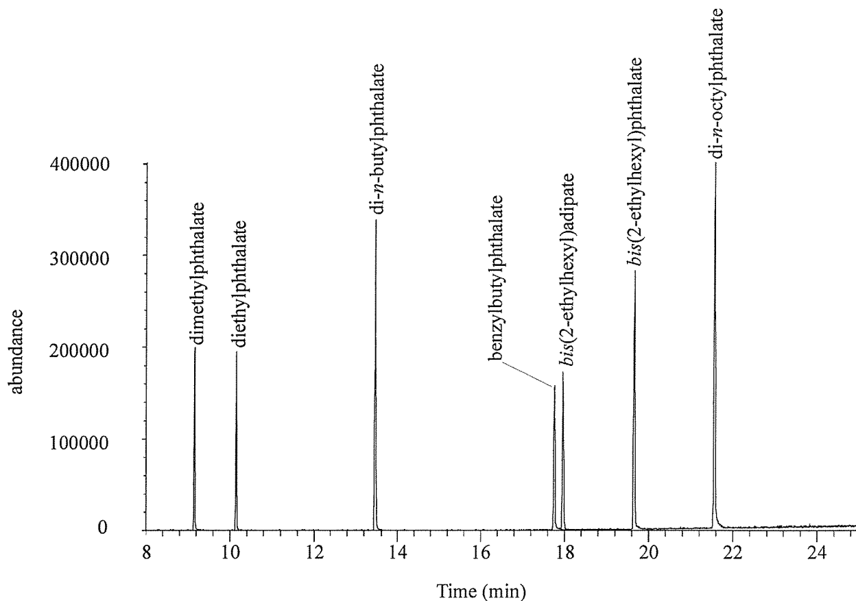
Figure 1. Chromatogram from GC/MS analysis of NIST SRM 3074 using a 0.25 mm i.d. × 60 m (length) fused-silica capillary column with a 5% phenylmethylpolysiloxane phase (0.25 μm film thickness). Temperature Program: 100 °C (1 min) then 30 °C/min to 200 °C, then 7.5 °C/min to 320 °C; MS scan from 50 m/z to 300 m/z (2.4 scans/s), electron multiplier voltage = 2000 V.
