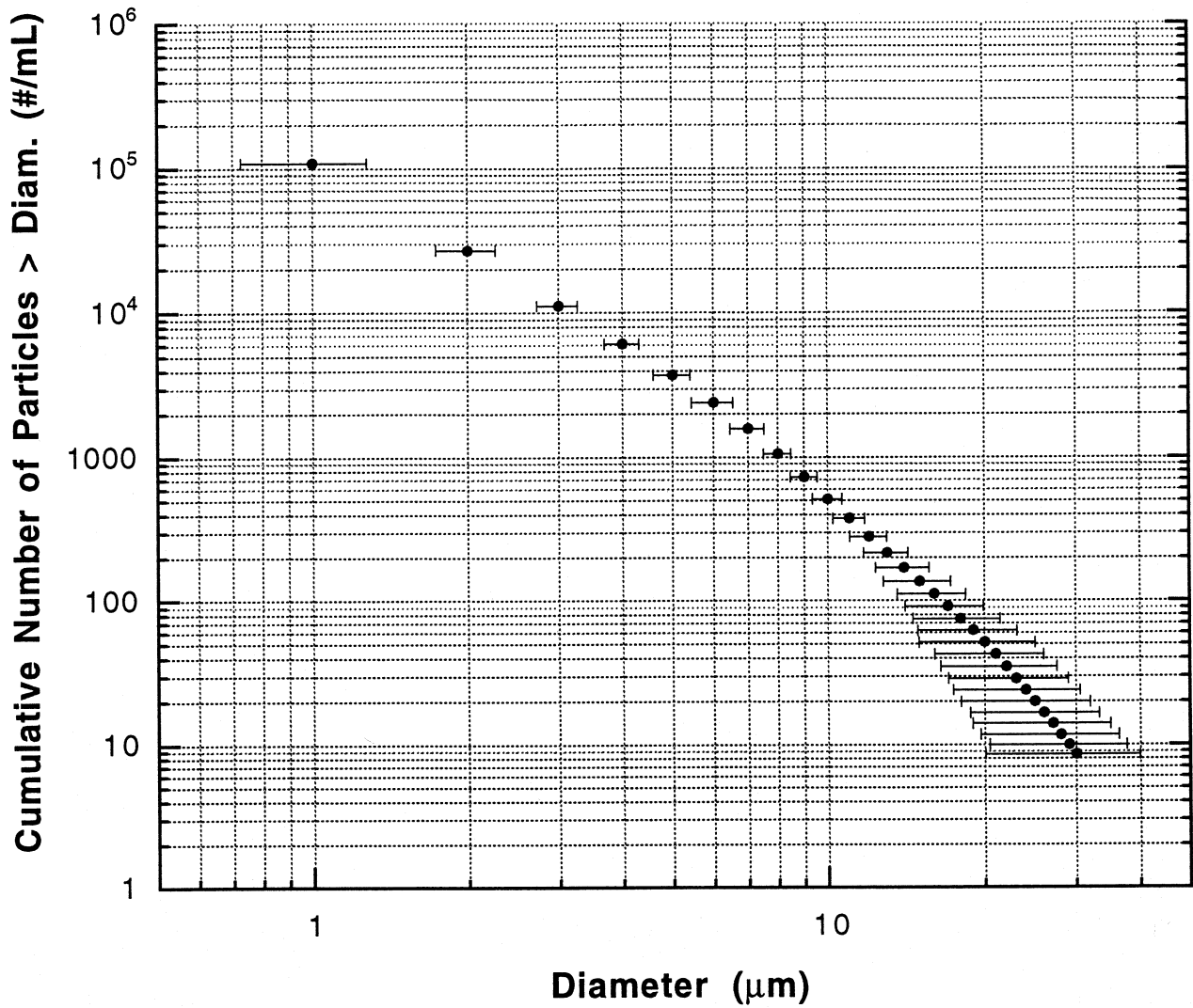
Figure 1. Plot of cumulative number of particles per milliliter of hydraulic oil greater than the specified projected area diameter. The uncertainty bars are the expanded uncertainties with k = 2 .
