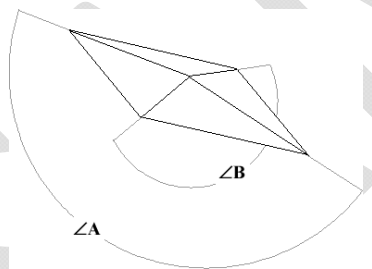
Figure 2. Knoop indenter geometry showing \angle A , the included longitudinal edge angle, and \angle B , the included transverse angle
