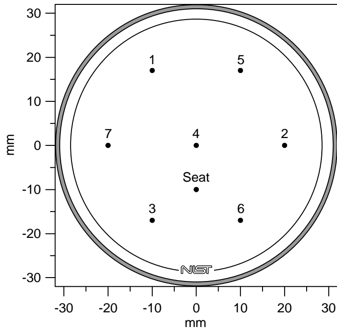
Figure 1. Test surface of SRM indicating the location and sequence of certification indentations (shown as black dots), and illustrating the appearance of the engraved circle and NIST logo. The first indentation, labeled “Seat”, was made to ensure that the new test block was adequately seated on the anvil. The indentations labeled 1 through 7 indicate the indentation sequence used in certification.
