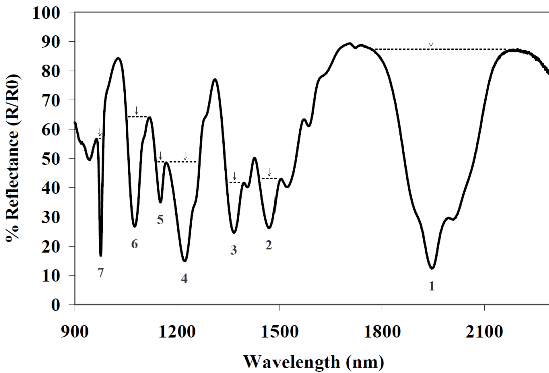
Figure A1. SRM 2036 Diffuse Reflectance Spectrum. Specular-excluded spectrum acquired at 5 nm spectral slit width. The dashed lines and arrows indicate the base of the band from which the 10 % band fractions were calculated for band location certification. They do not represent the 10 % band fractions. See values of potential interest to users for additional information pertaining to Band 1 centroid location.
