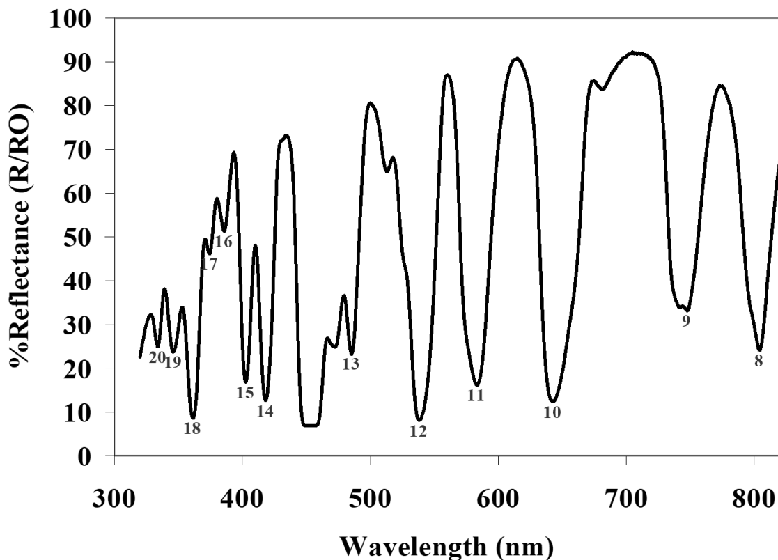
Figure A2. SRM 2036 Diffuse Reflectance Spectrum. Specular-included spectrum acquired at 5 nm spectral slit width.
