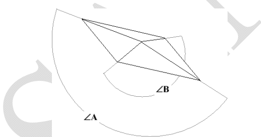
Figure 2. Knoop indenter geometry showing ∠A, the included longitudinal edge angle, and ∠B, the included transverse angle
