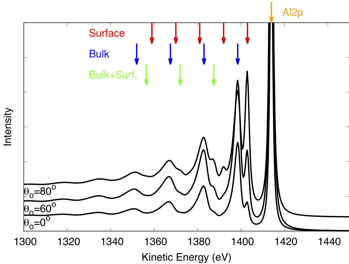
Figure 5.1: Simulation results for the Al- K\alpha excited Al 2 p photoelectron peak taking into account surface excitations using the database "SEP03" for different photoelectron emission angles \theta_0 with respect to the surface normal. Red arrows indicate surface plasmons, blue arrows indicate bulk plasmons, and green arrows indicate combination bulk and surface plasmons (see text).
