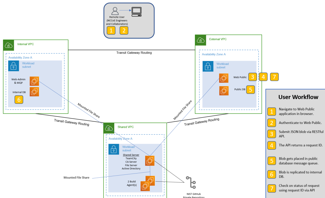
Fig. 2. Legacy System End User Workflow
