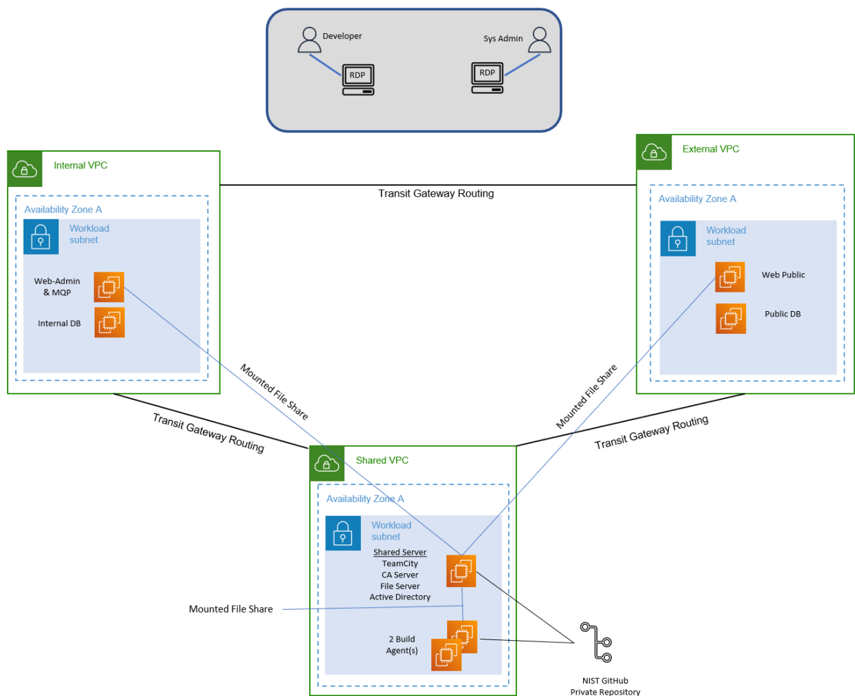
Fig. 1. Legacy System Architecture Diagram
