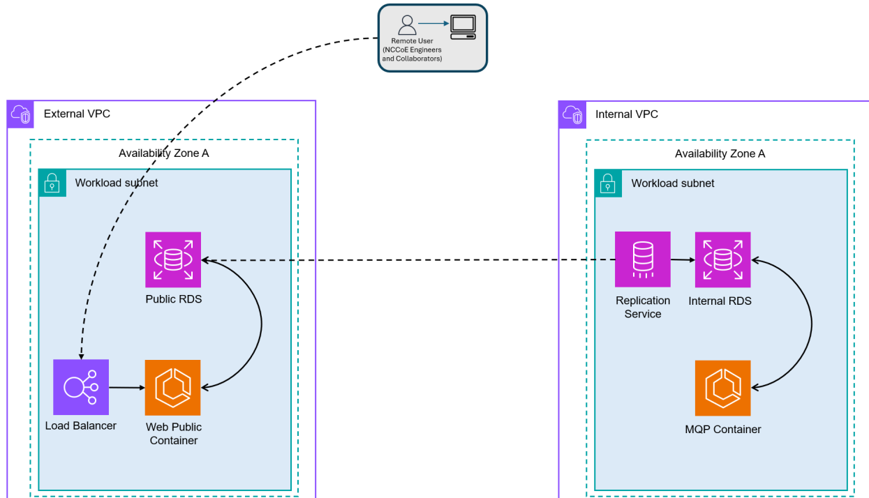
Fig. 7. Modernized Client Workflow
