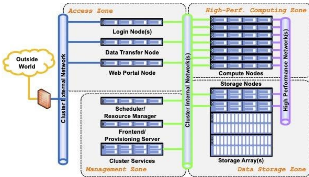
Fig. 1. HPC system reference architecture
