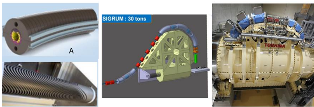
Figure 7. Right, SC gantry capable of 360° rotations at NIRS/HIMAC [25]. Left, Curved SC magnets combining dipole & quadrupole, and Center, SC rotating gantry designed for NIMMS [26].
