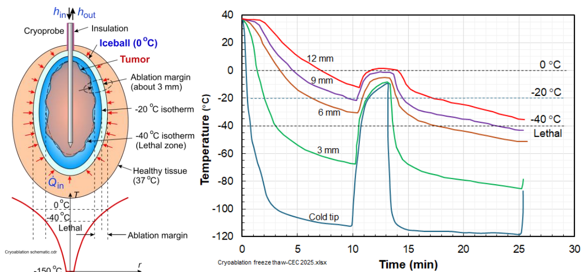
Figure 1. Left: Schematic of cryoablation isotherms showing tumor, ice ball, and ablation margins. Right: Example of freeze/thaw ablation in the first cycle [4].
