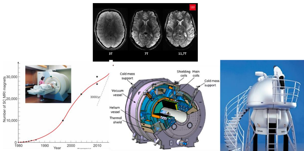
Figure 3. Left, Superconducting MRI systems in use around the world. Inset: Modern MRI system with a 1.5 T SC magnet and cryocooler, photo: Siemens. Center, 11.7 T Whole Body MRI [11]. Right, 900 MHz (21.1 T) NMR system, Photo: Varian. Upper, MRI images with different magnetic field, the higher fields the higher resolutions.
