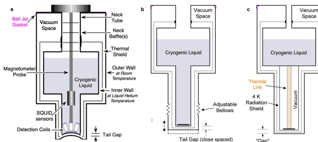
Figure 4. Different methods of achieving close dewar tail spacing. MLI is omitted for clarity.
