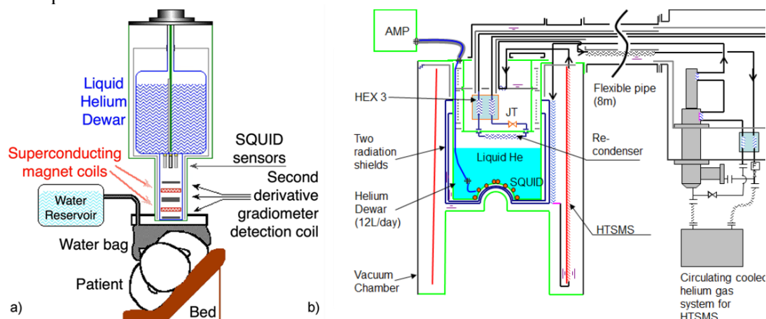
Figure 5 Left, coil-in-vacuum system for combining SQUID sensors and superconducting magnetic to measure magnetic susceptibility of internal organs [16]. Right, diagram of a MEG system utilizing a remote liquefier/recondenser to achieve zero boiloff [20].
