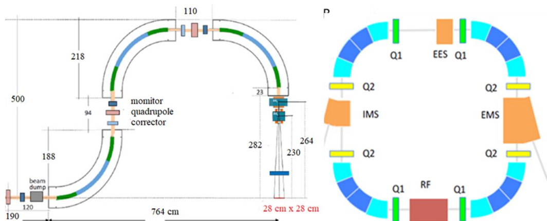
Figure 6. Right, Lay out of the synchrotron. Left, Layout of the 4-T gantry, the quadrupole coils inside the main CCT magnets. [24]
