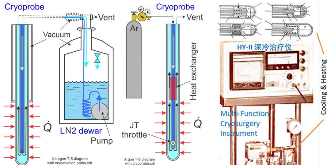
Figure 2. Left, Structure of a liquid nitrogen cryoprobe (Not to scale). Center, Structure of a JT cryoprobe (Not to scale). Right, Photo of a multifunction cryosurgery instrument with optional tips [6].
