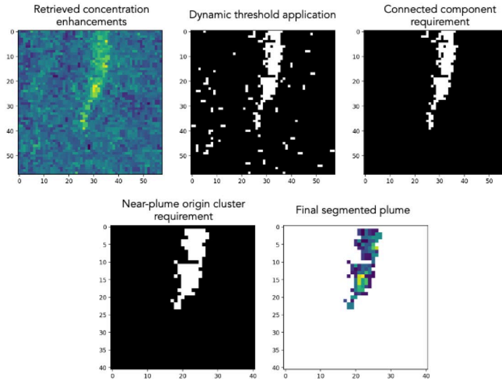
Figure 6. Steps Showing the Process of Finding the Methane Enhancement and Then the Plume. Credit: Dan Cusworth, Carbon Mapper, used with permission.
