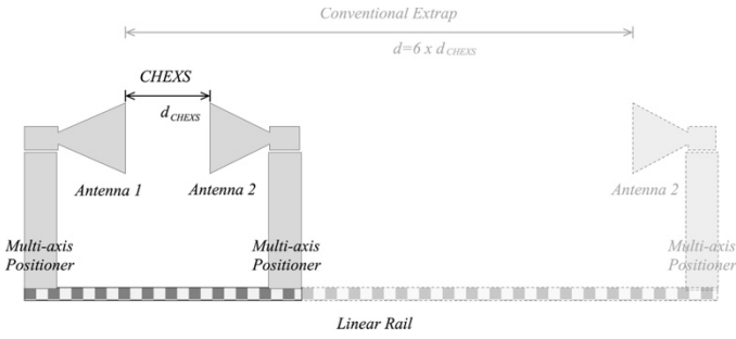
Figure 2. Length comparison (to-scale) of CHEXS vs a conventional gain extrap range. The antenna separation, d , for the conventional extrap range is up to six times greater than for the CHEXS.
