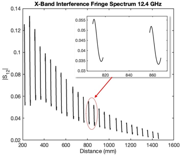
Figure 1. Example of interference fringes obtained with a CHEXS at 12.4 GHz for X-band standard gain horn antennas that result from direct-wave and third order scatter waves. Inset shows a close up of the fringes centered at 813 mm and 861 mm.
