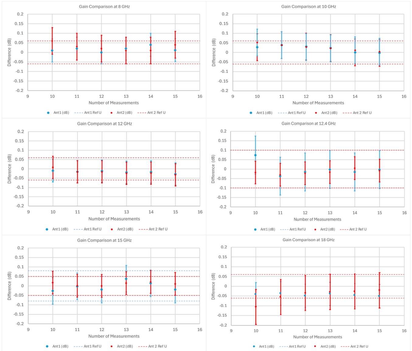
Figure 3. For each frequency, shown in each plot are the difference between the reference gain values and the measured gain from the CHEXS as a function of the number of data points used. Antennas 1 and 2 are denoted as Ant1 and Ant2 respectively in the legends. The uncertainty (taken from Table II) for each gain value is given by the error bars. Dotted lines for upper and lower bounds for the reference gain uncertainty (taken from [13] and [14]) for antennas 1 and 2 are denoted in the legends as “Ant1 Ref U” in blue and “Ant2 Ref U” in red respectively. These bounds are equal for Ant1 and Ant2 for all frequencies, except 15 GHz, where there are then two sets (blue and red) of upper and lower bound dotted lines.
