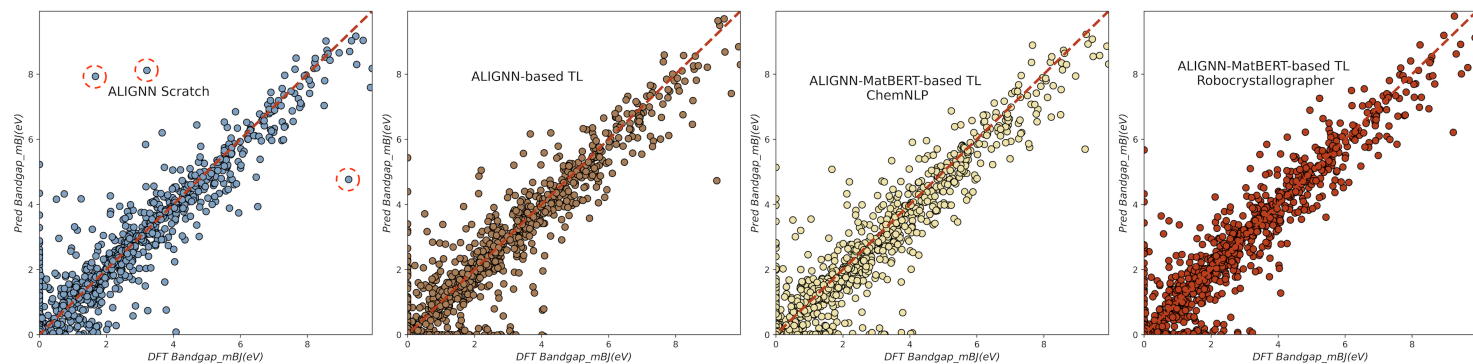
Fig. 2 Parity plot of the original ALIGNN model (1st), ALIGNN-based feature extraction transfer learning (2nd), and the proposed hybrid transfer learning approach based on ChemNLP (3rd) and Robocrystallographer (4th) for predicting bandgap computed by mBJ. The successful elimination of extreme prediction errors circled in ALIGNN Scratch model plot contributes to the Mean Absolute Error performance gain.
