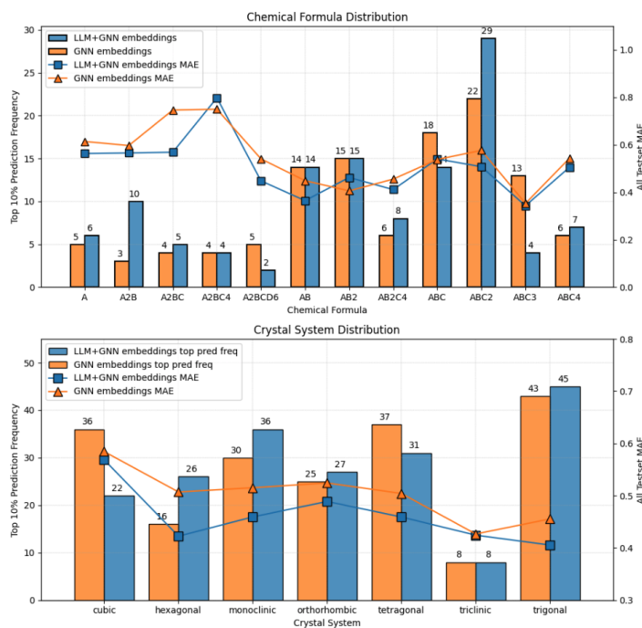
Fig. 6 Test set performance categorized by composition prototype (top) and crystal system (bottom) for bandgap property with metal samples excluded. The predictions using ALIGNN-MatBERT-based embeddings (blue) are compared with those using only ALIGNN embeddings (orange). All results are based on Robocystallographer text.
