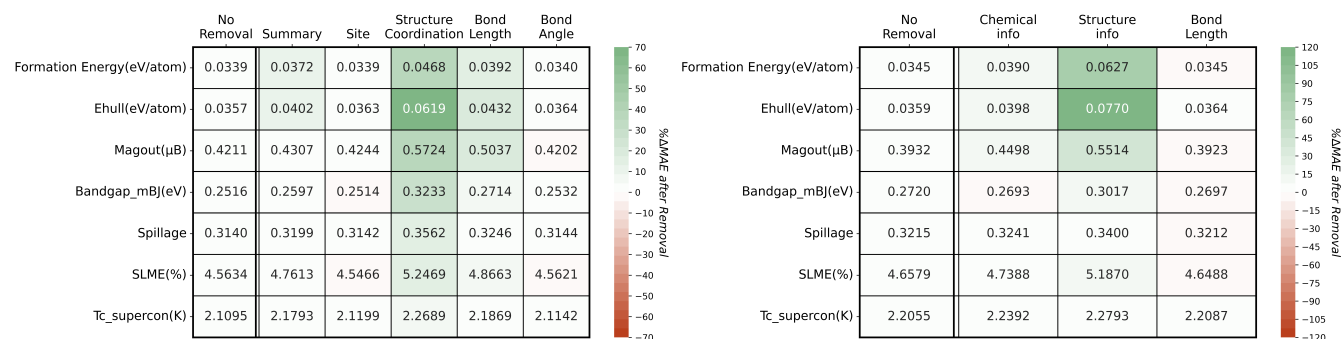
Fig. 5 Heatmap for comprehensiveness for ALIGNN-MatBERT-based TL results (left: Robocrystallographer; right: ChemNLP). The values in each cell present the MAE values with the removal of each tag and the color indicates the magnitude of MAE change with more significant tags shaded by darker color.
