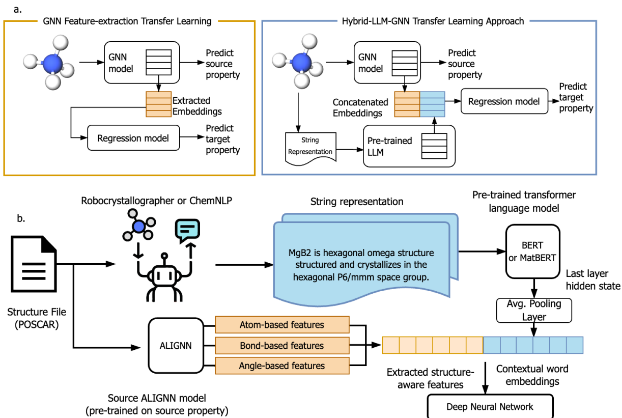
Fig. 1 a.(top) Workflow comparison of feature-extraction-based transfer learning approaches. Left: original GNN-only embedding feature extraction; Right: proposed hybrid transfer learning. b.(bottom) Detailed workflow of proposed Hybrid-LLM-GNN feature extractor. First, the input structure file is fed to an NLP-based text generator to produce domain knowledge descriptions. Next, the pre-trained LLM, serving as a knowledge model, is employed to extract contextual word embeddings, which are further concatenated with ALIGNN embeddings to leverage textual learnings to improve the predictive ability of the forward model.
