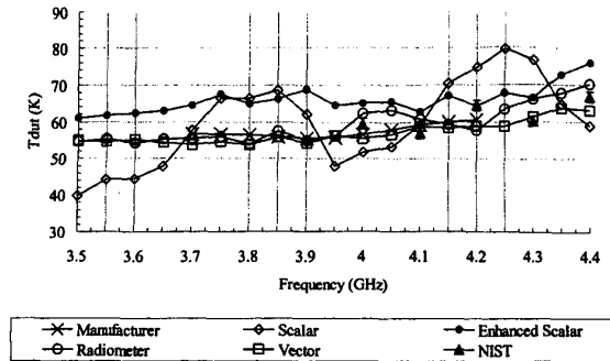
Fig. 4 Synthetic cold source data with scalar, enhanced scalar and NFM radiometer measurements performed at Raytheon Andover, vector measurements performed at Agilent Technologies North Billerica, and NIST measurements performed in Boulder, CO using NIST's NFRAD. Error bars are for a \pm 1.4 K NIST measurement uncertainty.
