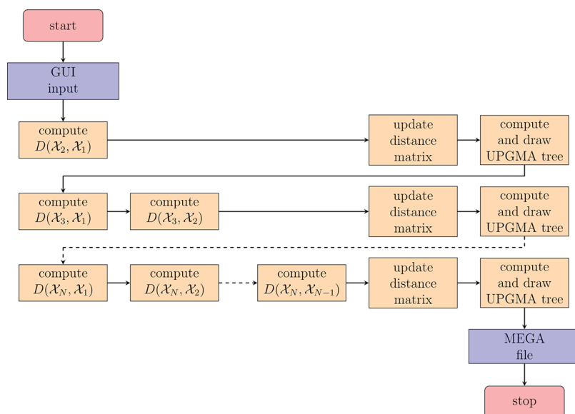
Figure 1. CompareMS2 2.0 workflow, orchestrated by the graphical user interface. After parsing and checking the input parameters, ensuring all files are present and in the correct format, compareMS2 performs (N^2 - N)/2 pairwise comparisons of N datasets using the symmetric distance measure described below, or N^2 - N comparisons if the original measure is used. After each row is completed, compareMS2 updates the (strictly triangular) distance matrix and generates a new tree. This allows the user to monitor progress and terminate and restart the run if necessary. If the original measure is used, compareMS2 by default creates both the strictly upper and lower triangular distance matrices (these can be averaged in phylogenetics software such as MEGA).
