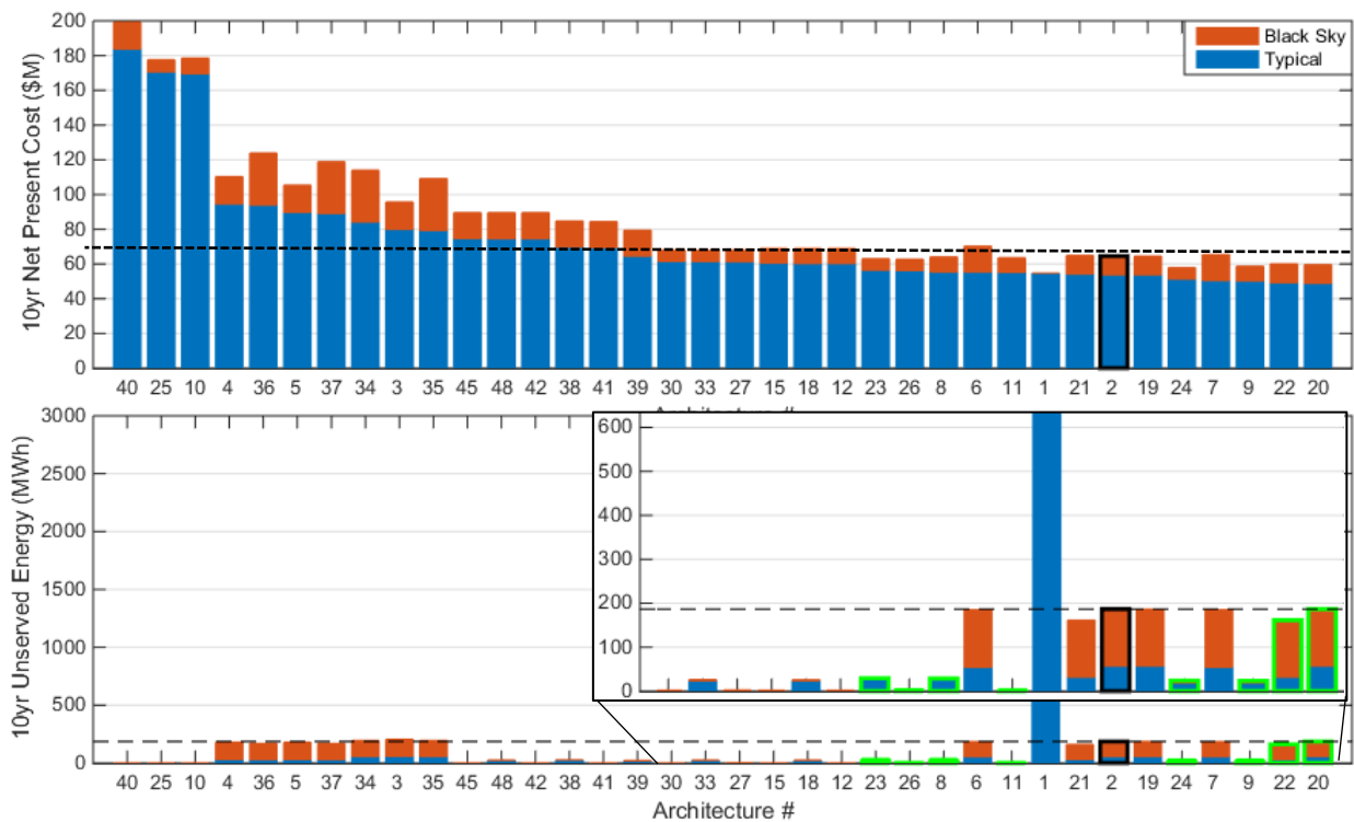
Figure 13-4 LCC versus Unserved Energy (2-Week Outage) [133]
