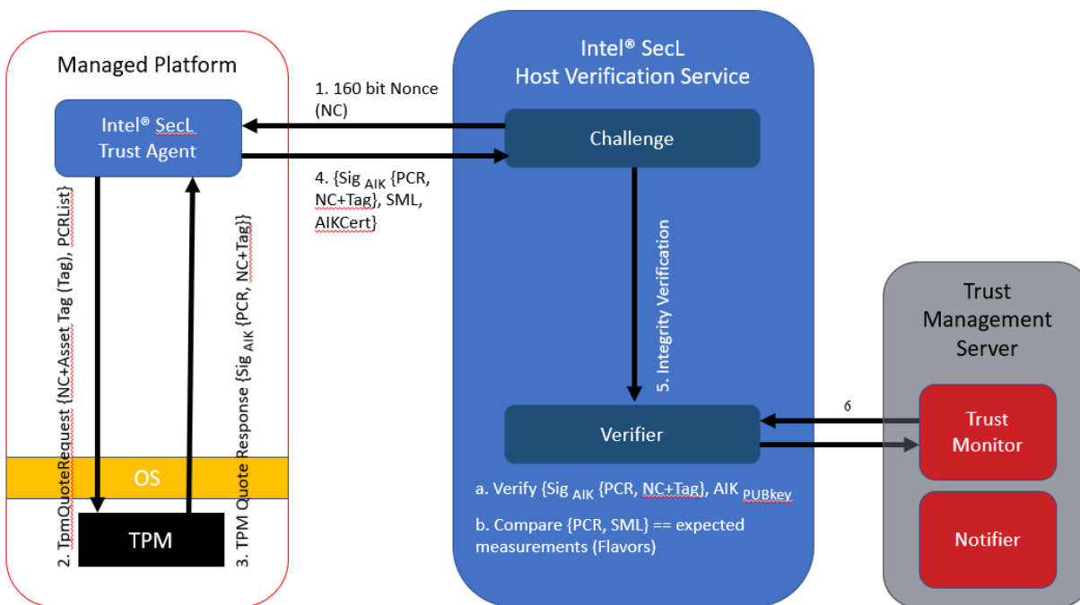
Figure 6: Remote Attestation Protocol
