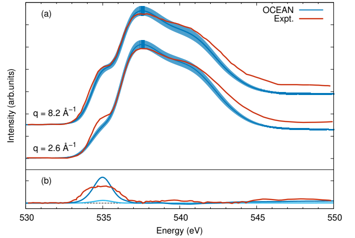
Fig. 10 a) The O K edge of liquid water as seen with NRIXS at momenta of 2.6 \text{ \AA}^{-1} and 8.2 \text{ \AA}^{-1} . Other than the value of the momentum transfer the details of the calculation are the same as for Fig 9, and the experimental data is from Ref 75. b) The difference between the high and low momentum spectra for OCEAN in blue and the measured data in red. For reference, the difference between q = 2.6 \text{ \AA}^{-1} and a dipole XAS calculation is shown in cyan, showing already a slight increase in the pre-edge feature at finite momentum. While the calculated pre-edge appears to be growing faster with increasing momentum in (a) than the measured pre-edge, in (b) it is clear that in the measured data the pre-edge is wider at higher q . The change in the area of the pre-edge is very similar between OCEAN and experiment.
