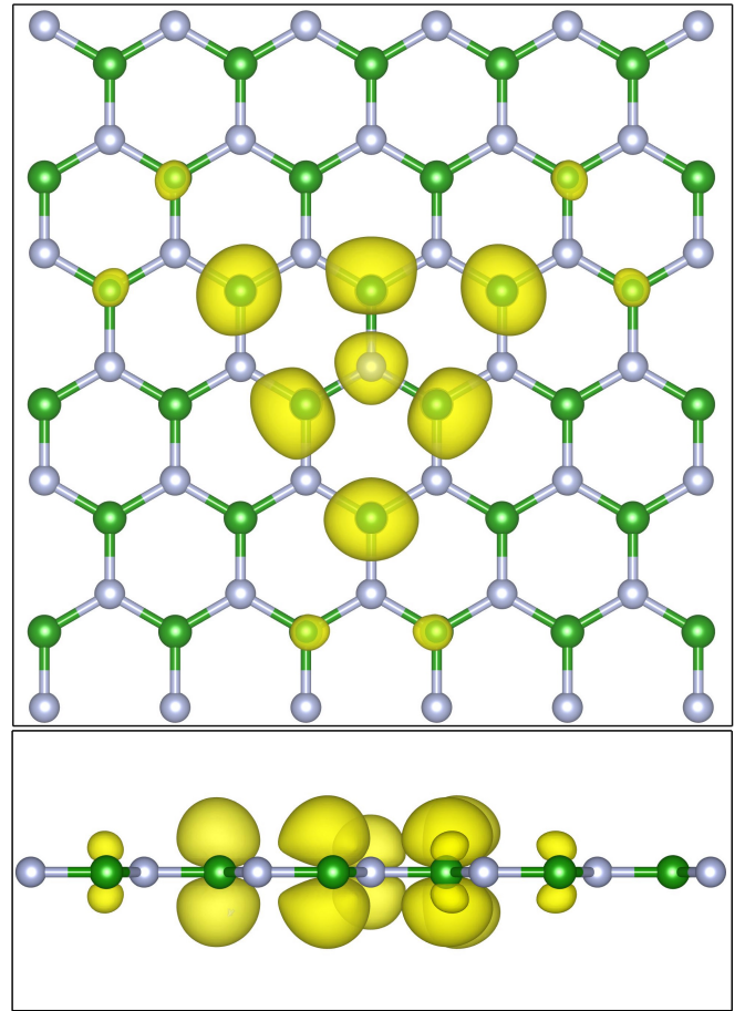
Fig. 4 Top) The excited electron density (yellow) of the lowest energy exciton of a single sheet of hexagonal boron nitride at the nitrogen K edge viewed looking down. Bottom) the same plot but viewed from the side. The absorbing site is the central nitrogen atom (grey). The majority of the electron density is sitting in p_z type states on the first and second nearest neighboring boron atoms (green). Plots generated using VESTA. 56
