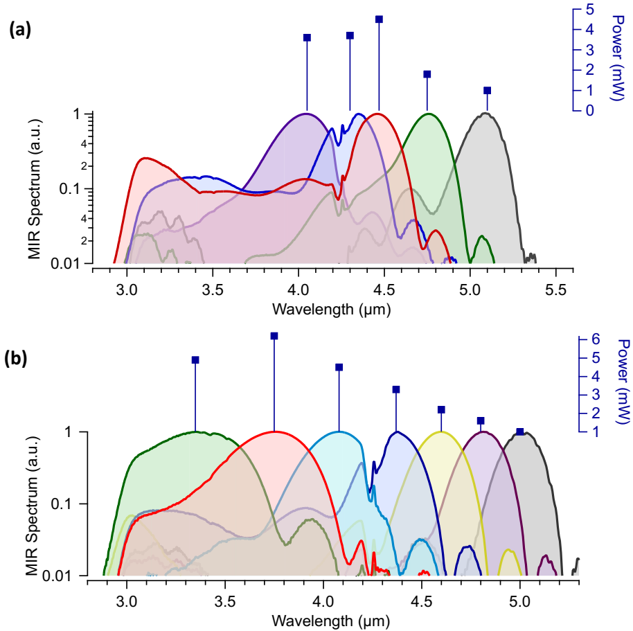
Figure 5. (a) MIR spectra generated by focusing 1.5 cycle pulse into a fanout PPLN crystal. Broadest spectrum covers 3 - 4.7 \mu\text{m} and 4.5 mW of power. (b) MIR spectra with a PPLN with 7 individual periodically poled gratings (out of 16 total). Maximum power is 6.2 mW and covers 3 - 4 \mu\text{m} .
