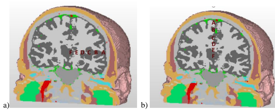
Fig. 6. Implant locations for which the power flow and channel attenuation have been evaluated a) on-body antenna at location 1 and b) on-body antenna at location 2
