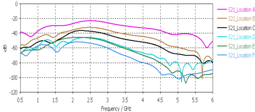
Fig. 9. Forward channel coefficient ( S_{21} ) for different implant locations and mini-horn antenna location 1
