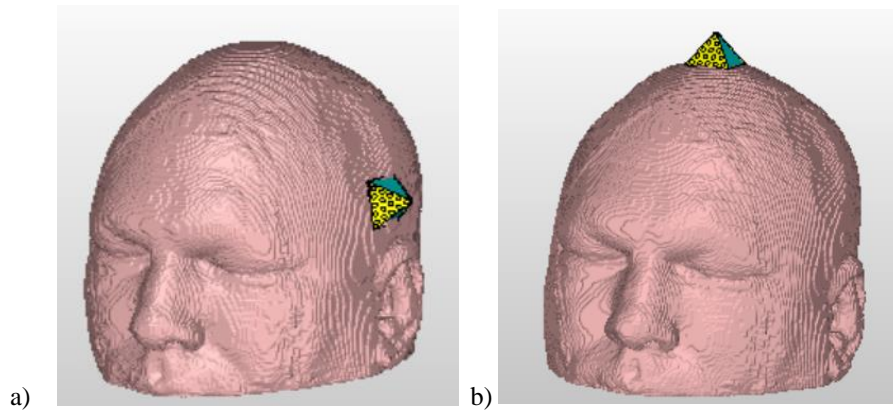
Fig. 3. On-body antenna locations: a) Location 1 (above the temporal bone on the left side), b) Location 2 (top of the head)
