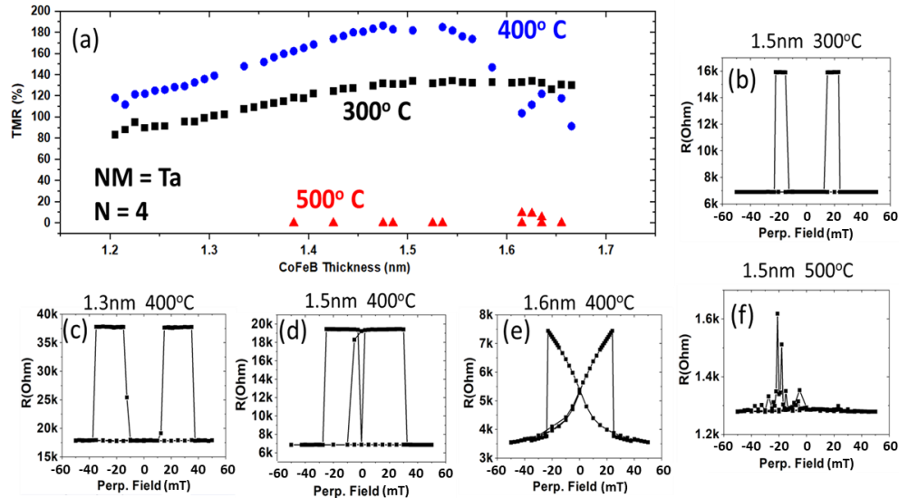
Figure 3. (a) CoFeB thickness dependence of the TMR in pMTJs with Ta-MIFLs. The samples were successive annealed at each temperature for 10 min. (b) TMR curve of the 1.5 nm sample after the 300°C annealing. (c-e) TMR curves of three pMTJs after the 400°C annealing. (f) TMR of the 1.5 nm sample after the 500°C annealing.
