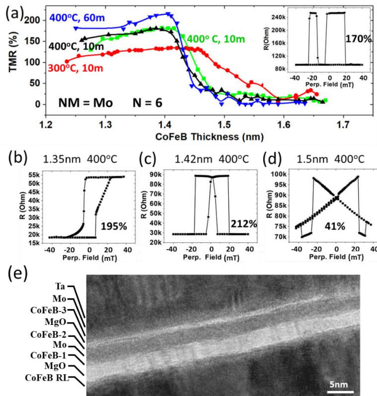
Figure 4. (a) CoFeB thickness dependence of the TMR in pMTJs with Mo-MIFLs. The samples with Mo-0.9nm coupling layer were successive annealed at 300°C for 10min (red dots), 400°C for 10min (black up-pointing triangles), then 400°C for another 50min (blue down-pointing triangles, where the total annealing time at 400°C is 60min). The green square data points are the TMR values of the samples with the Mo-1nm coupling layer, annealed at 400°C for 10min. The lines are for guiding eyes only. Inset shows the TMR curve of a pMTJ with the Mo-1nm coupling layer. (b-d) Representative TMR curves of three pMTJ after the 400°C annealing for 60min. (e) HRTEM image of the pMTJ with Mo-MIFL.
