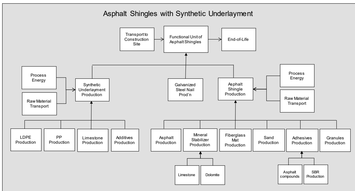
Figure 11-2 Asphalt Shingles with Synthetic Underlayment System Boundaries
