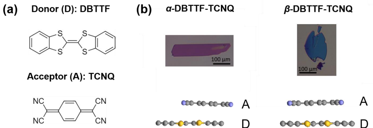
Figure 1: a) The donor (DBTTF) and acceptor (TCNQ) in the CT complex. b) Crystals of the \alpha - and \beta -polymorphs, with the donor-acceptor overlap displayed below. The scale bars are 100 \mu\text{m} long. The \alpha -polymorph is rectangular in habit, while the \beta -polymorph is elliptical and thin. The overlap is depicted from the crystal structure for the \alpha -polymorph measured by X-ray diffraction, while the \beta -polymorph overlap is predicted based on selected-area electron diffraction measurements. 23,43 The colors of the crystals are representative of their lamination onto a silicon wafer with 200 nm silicon dioxide.
