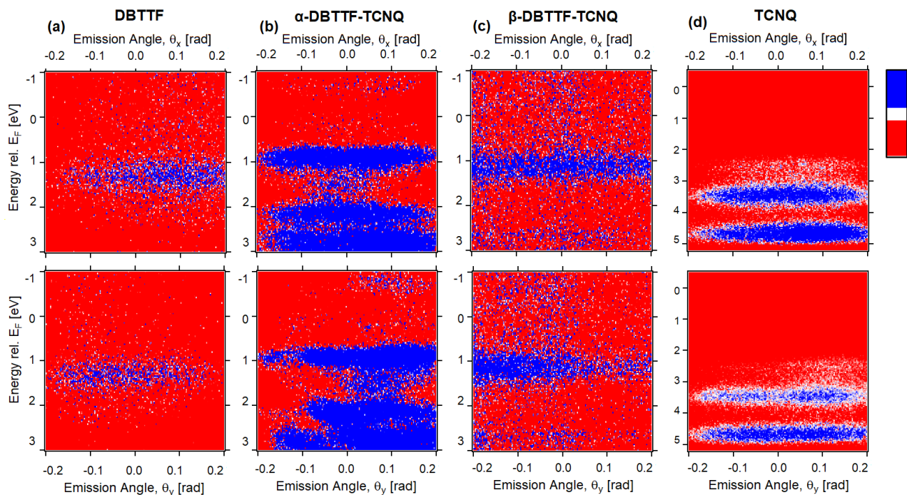
Figure 3. ARPES results of crystalline (a) DBTTF, (b) \alpha -DBTTF-TCNQ, (c) \beta -DBTTF-TCNQ, and (d) TCNQ. Top and bottom panel show the electron emission as a function of \theta_x and \theta_y , respectively, and high counts shown in blue and low counts in red. The data are shown within the angular emission range of \pm 0.2 rad (corresponding to \pm 0.8 \text{\AA}^{-1} ).
