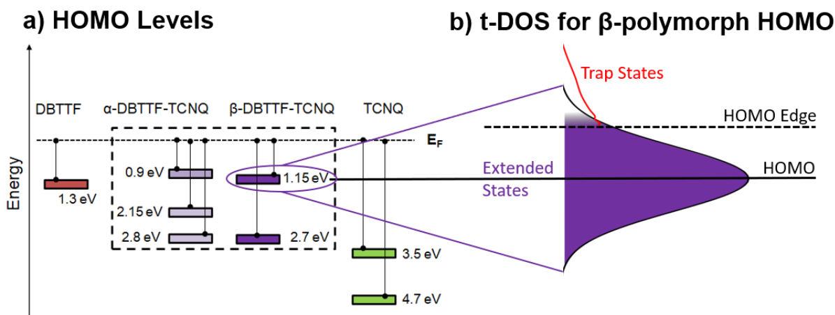
Figure 5: Electronic structure of \alpha - and \beta -DBTTF-TCNQ. a) A summary of the ARPES results shown in Fig. 3 of the identified HOMO levels of \alpha -DBTTF-TCNQ, \beta -DBTTF-TCNQ, and each parent compound. Energy referencing is to the Fermi level. The uncertainty is \pm 0.1 eV to account for contact potential differences between Au and Ag substrates. b) A schematic representation of the HOMO of \beta -DBTTF-TCNQ. The HOMO is represented by a gaussian distribution, and the t-DOS calculation for holes is shown in red at the mobility edge of the HOMO.
