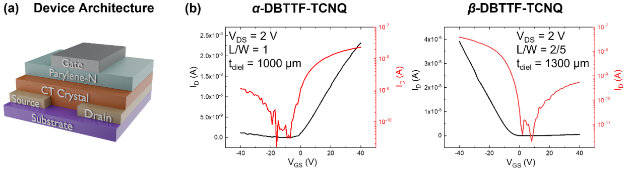
Figure 2: a) the bottom-contact, top-gate transistor architecture used to extract the trap-DOS for each polymorph. b) Examples of transfer characteristics in the linear regime for each polymorph. The V_{DS} , channel dimensions as a ratio of length to width ( L/W ), and thickness of the parylene-N gate dielectric ( t_{\text{Pary}} ) are given in the inset.
