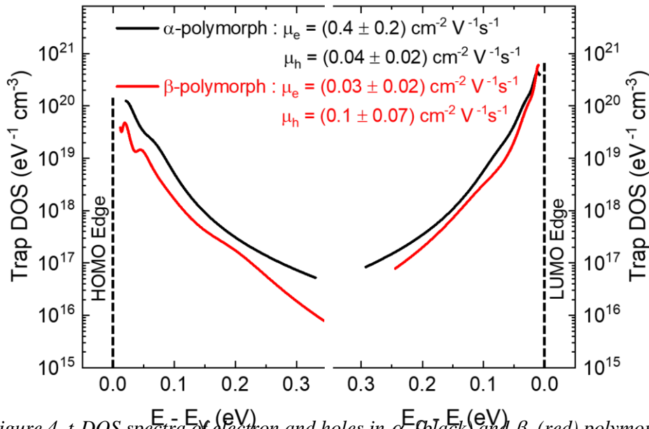
Figure 4. t -DOS spectra of electron and holes in \alpha - (black) and \beta - (red) polymorphs
