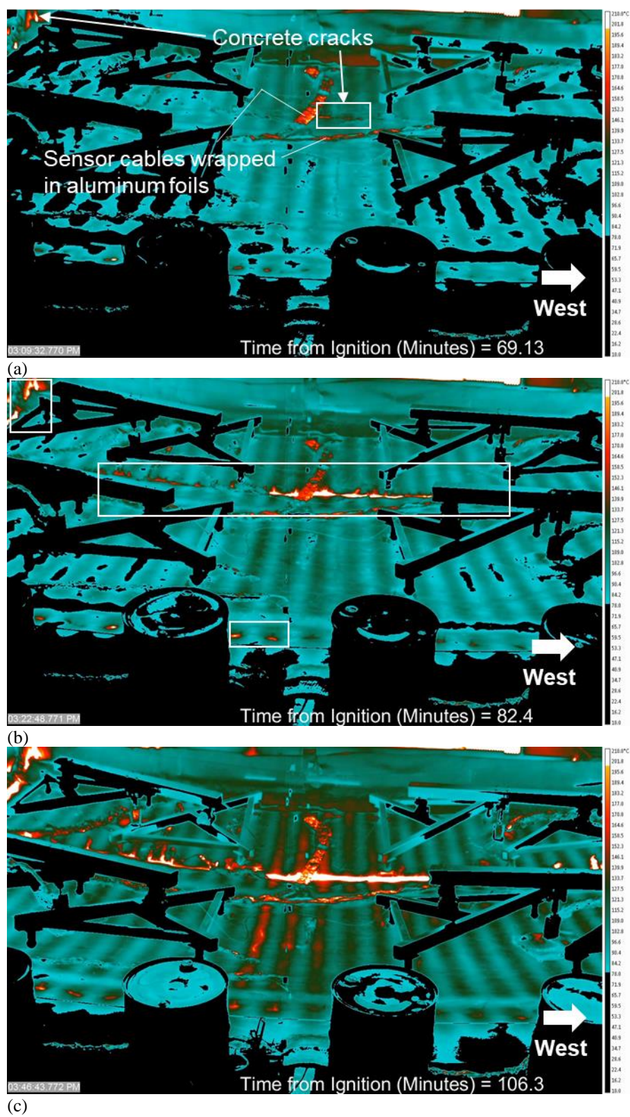
Fig. 4-29. Thermal images displaying top of the slab at (a) 69 min, (b) 82 min, and (c) 106 min.
