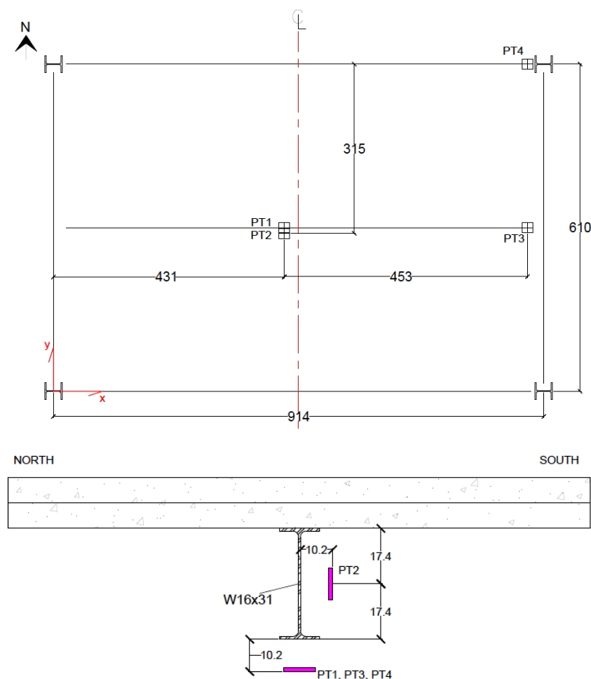
Fig. C-1. Locations of plate thermometers.
