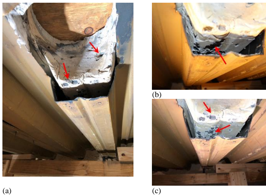
Fig. 4-40. Post-test photographs: (a) slab through-hole used for running a water-cooled loading tube; (b-c) deck delamination from concrete. Localized spalling is indicated by arrows.
