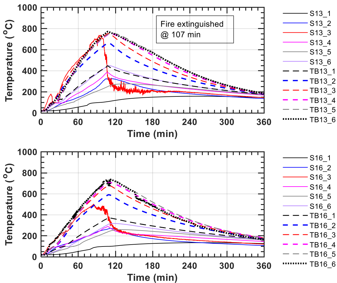
Fig. B-13. Composite section temperature at midspan of west girder (section 13) and east girder (section 16).
