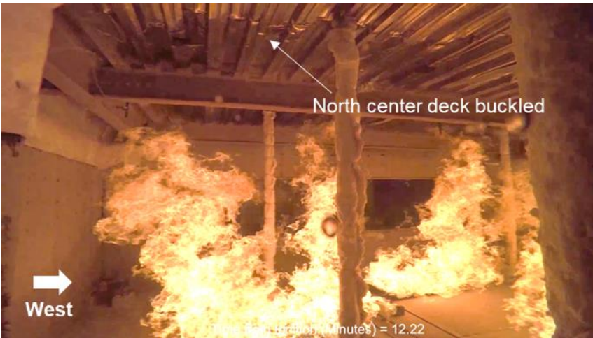
Fig. 4-25. A snapshot of the test video showing local buckling of the north steel deck at about 12 min.
