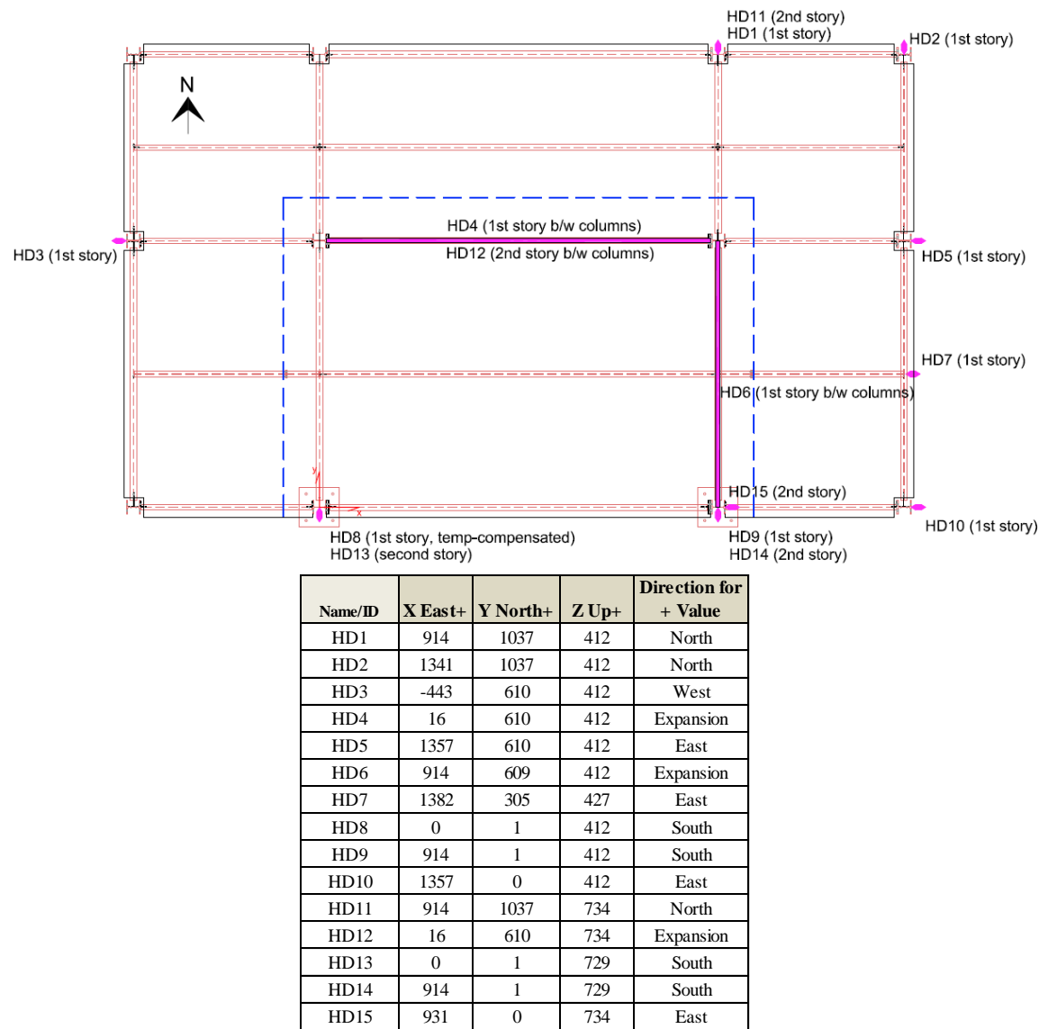
Fig. 4-34. Locations of horizontal displacement measurements, unit in cm. The XY origin is defined at the center of the southwest column of the test bay; The Z datum is defined at the laboratory strong floor.
