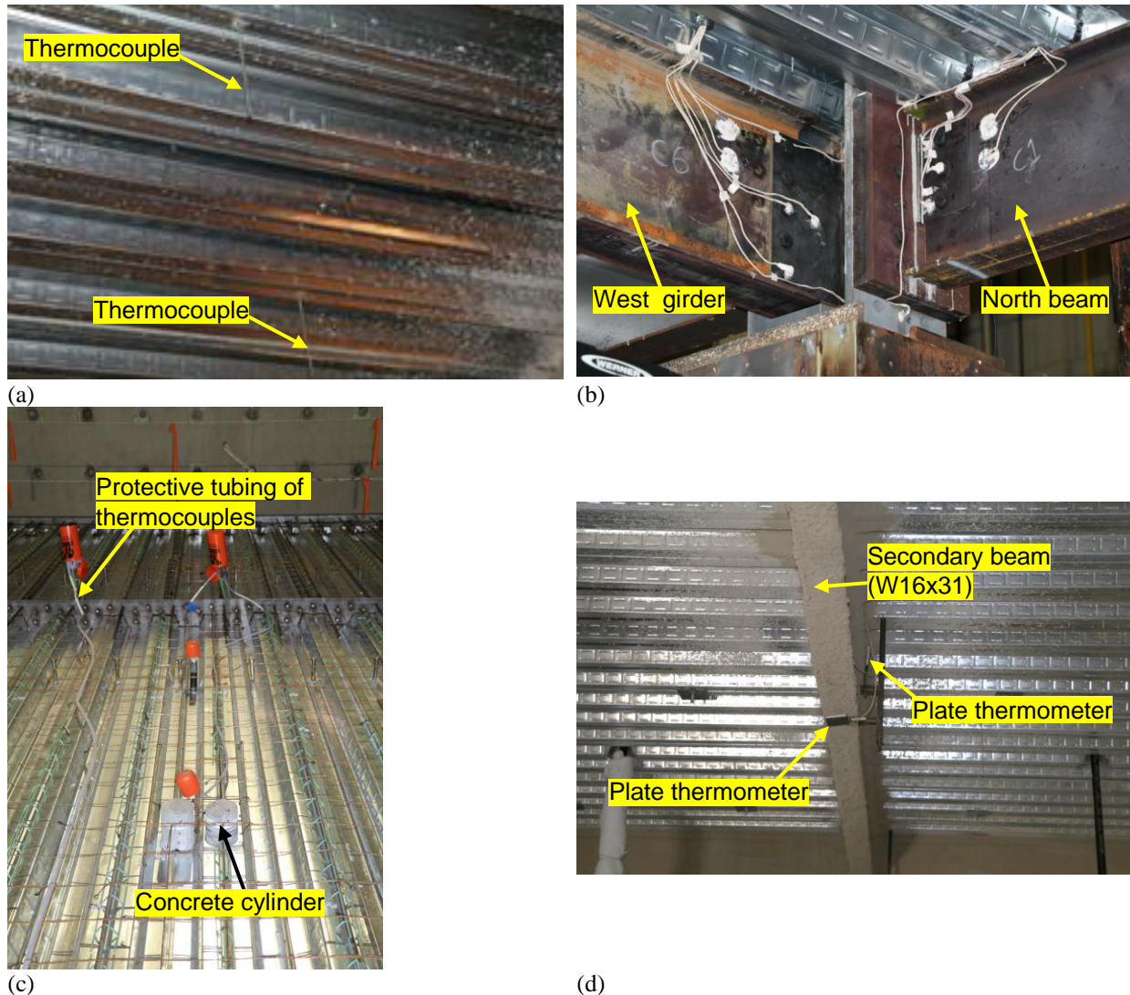
Fig. 3-4. Photographs of temperature sensors installed at (a) 305 mm below exposed steel deck; (b) ends of the west girder and the north beam prior to fireproofing; (c) top of the steel deck prior to concrete casting; (d) midspan of secondary beam.
