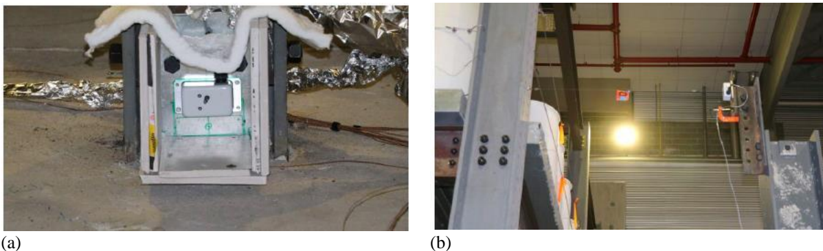
Fig. 3-3 String potentiometers installed at (a) the interior (B3) column and (b) the exterior (C4) column.
