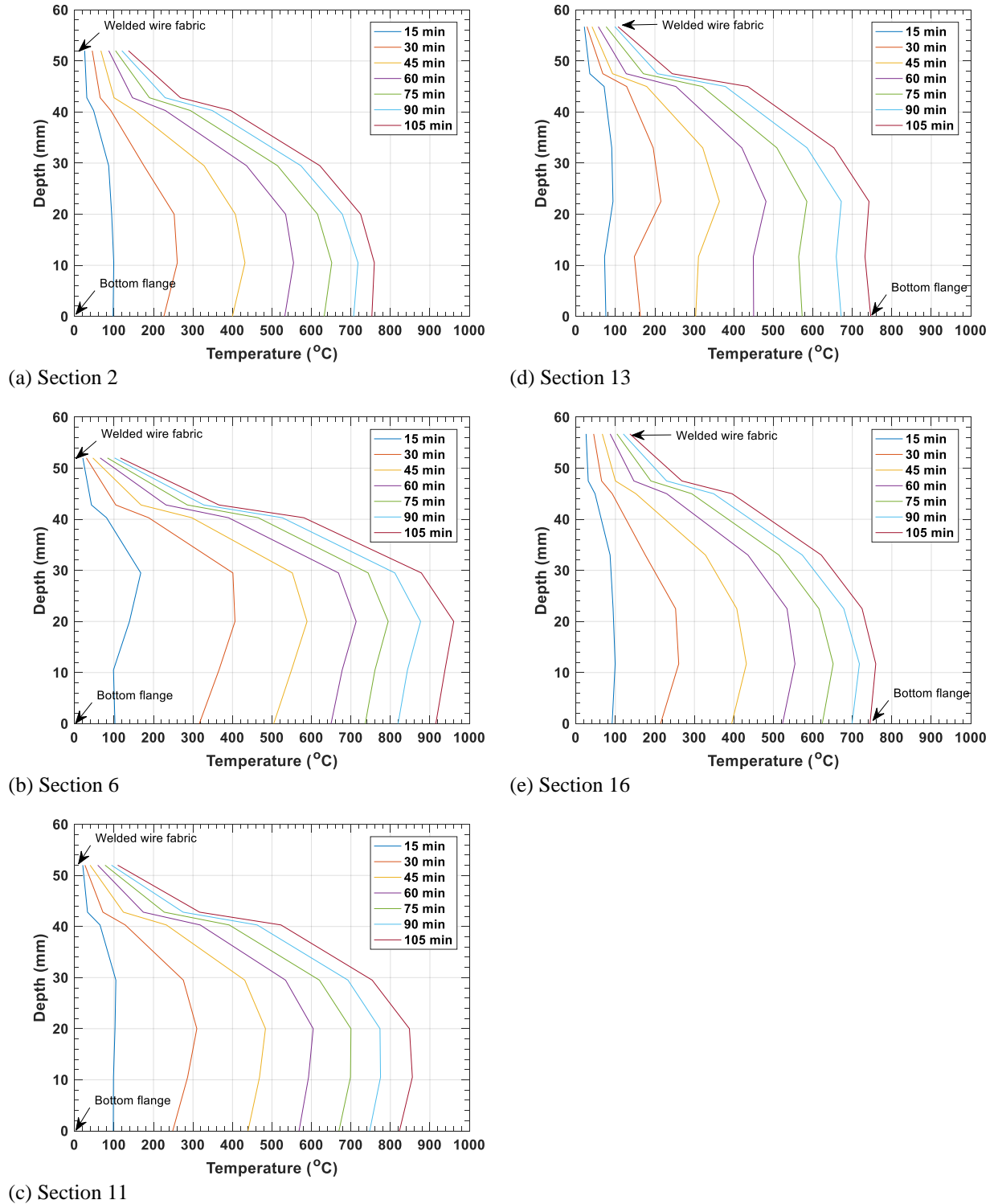
Fig. B-14. Change in thermal gradients through the depth of the midspan composite sections of (a) south primary beam, (b) secondary beam, (c) north primary beam, (d) west girder, and (e) east girder during heating.
