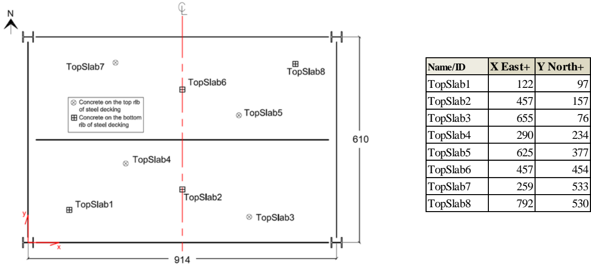
Fig. 4-17. Locations of thermocouple probes 3 mm below the top (unexposed) surface of the test floor slab, unit in cm.
