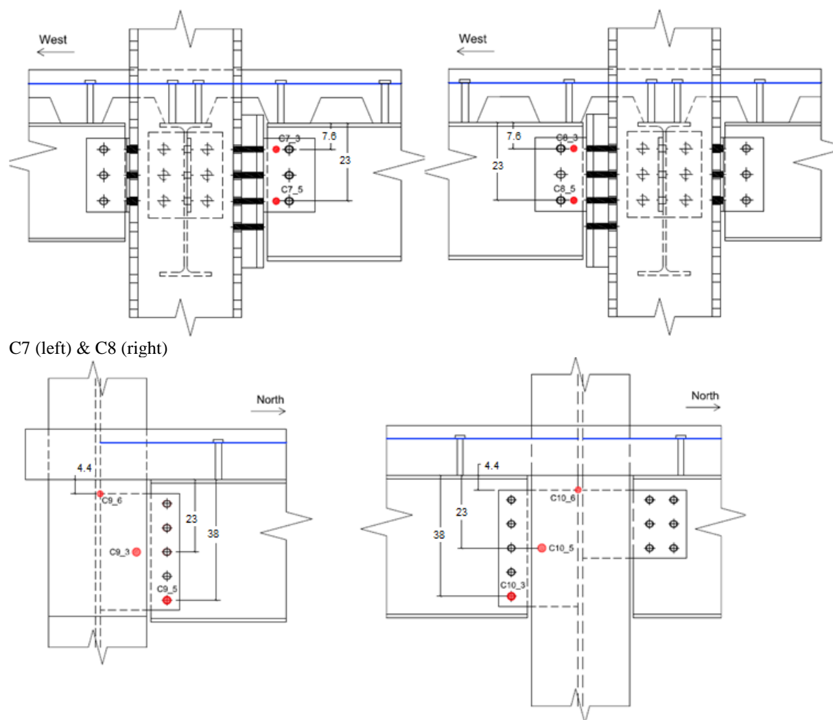
C9 (left) & C10 (right) Fig. B-17. Locations of thermocouples mounted at the ends of composite beams and girders in the test bay.
