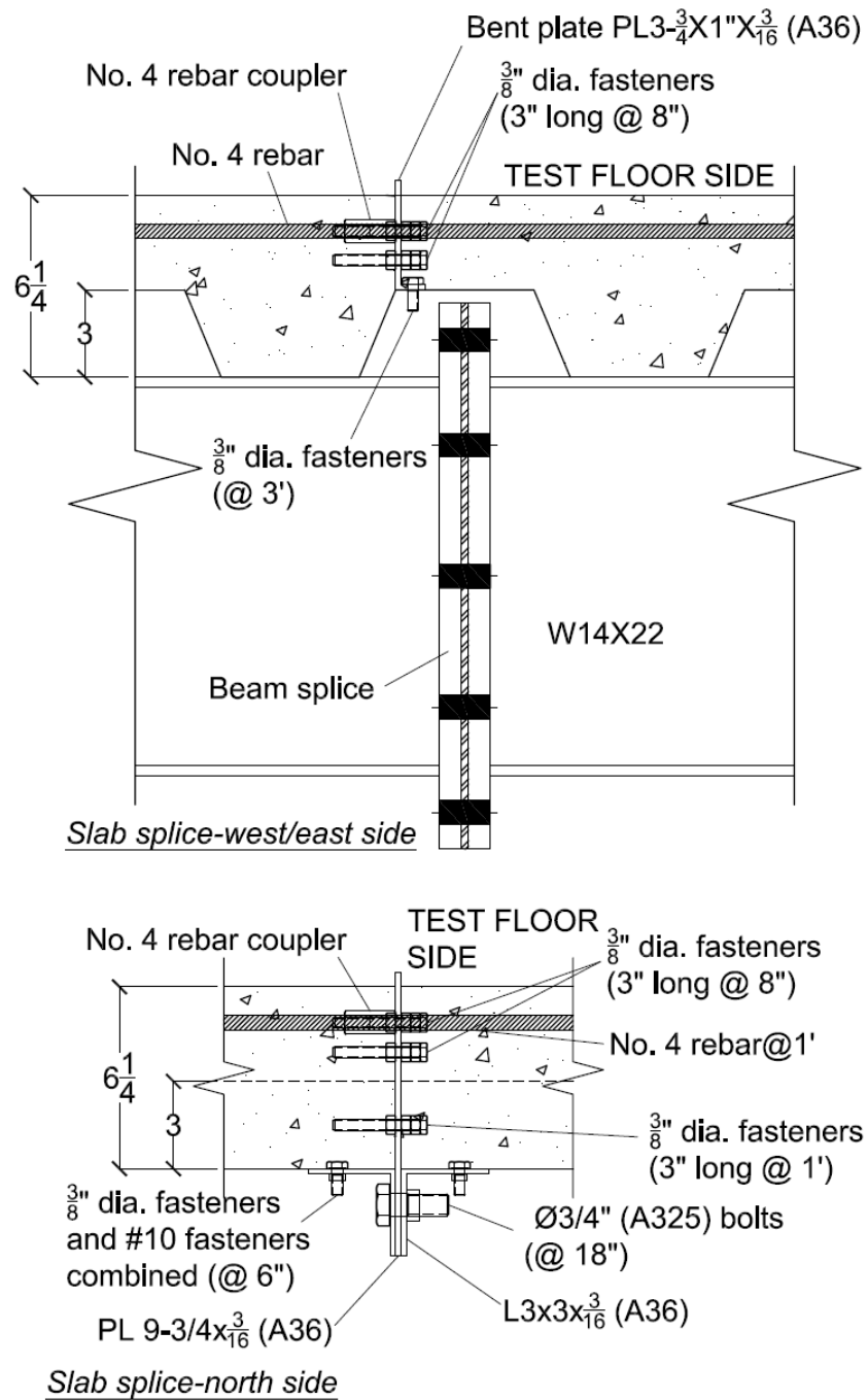
Fig. 2-20. Scale drawings of slab splices (unit = inch).
