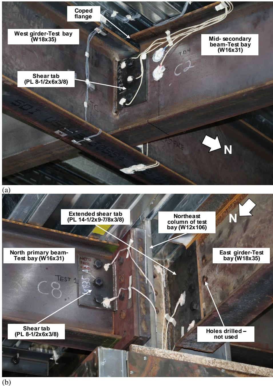
Fig. 2-11. Steel frame connections in the fire test bay: (a) beam-to-girder connection (b) beam-to-column flange and girder-to-column web connections.
