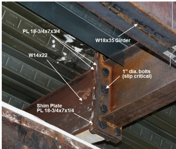
Fig. 2-16. Beam splice in the surrounding bay (unit = inch).
