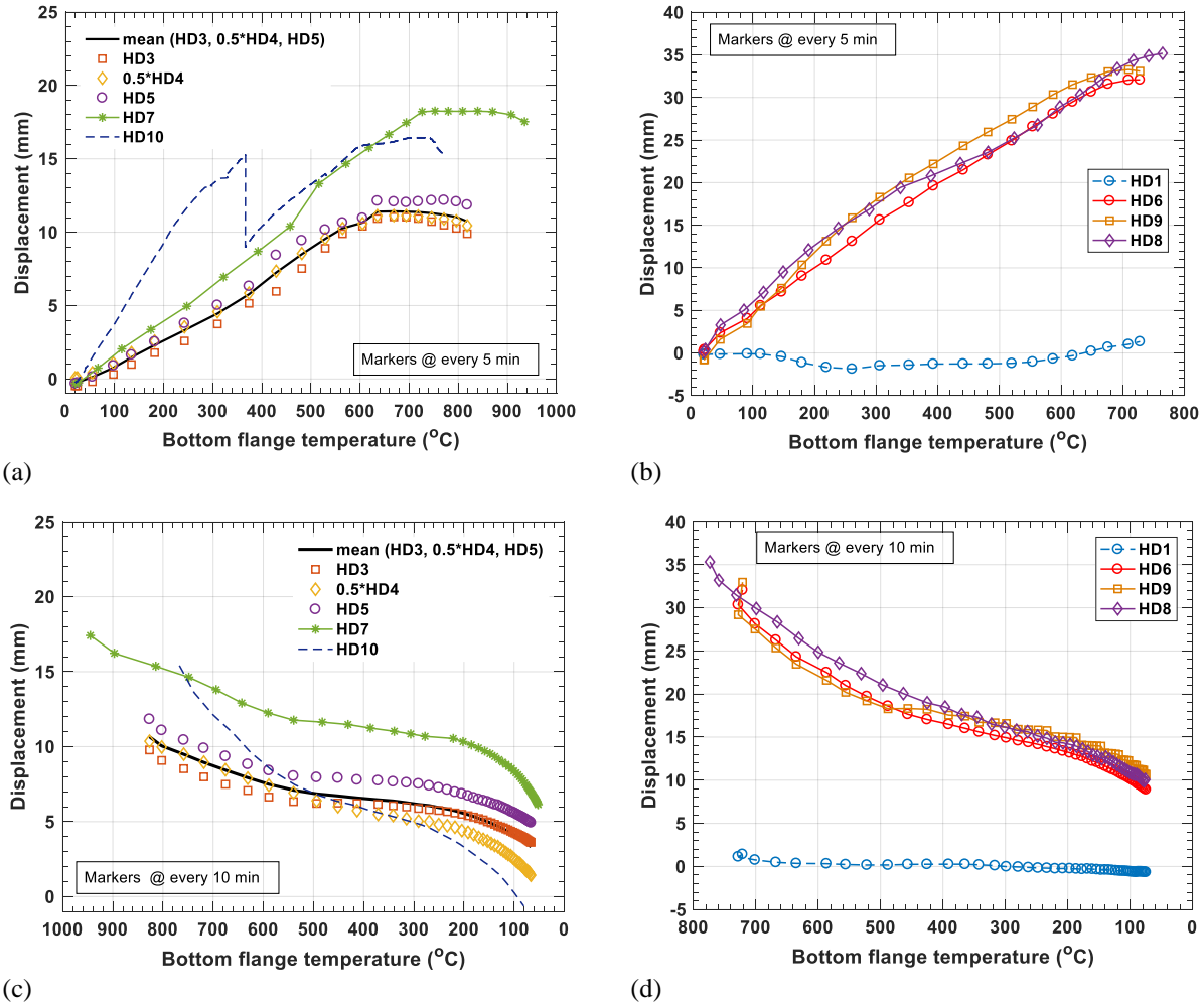
Fig. 4-36. Lateral displacements of the prototype building at the first-story level as a function of bottom flange temperatures in the test bay; (a) the east or west side during heating, (b) the north or south side during heating, (c) the east or west side during cooling, and (d) the north or south side during cooling.
