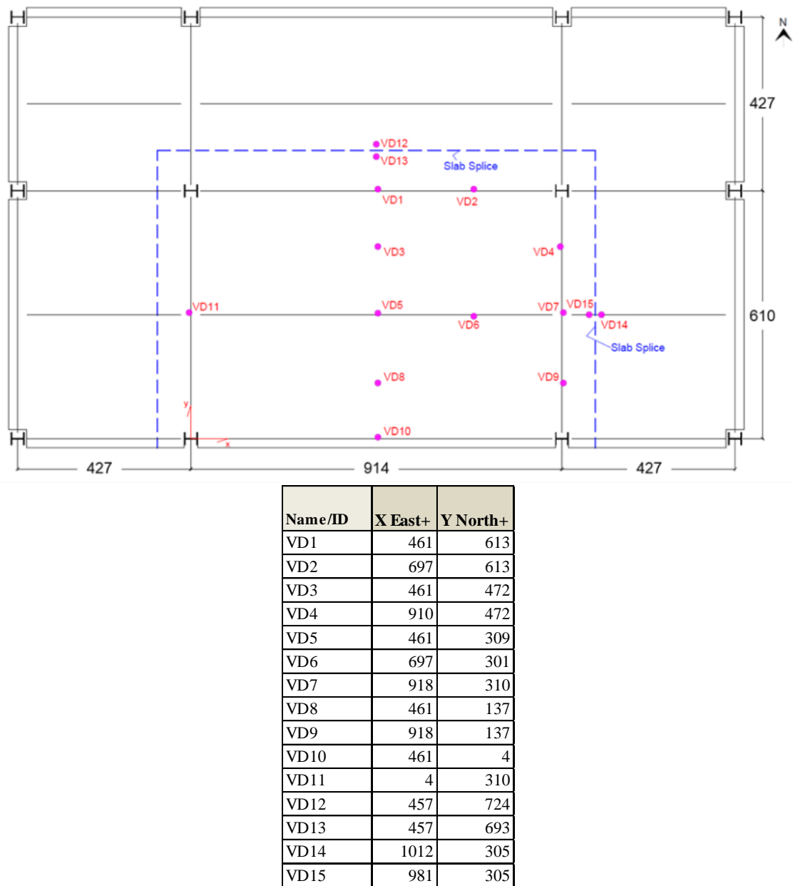
Fig. 4-30. Locations of vertical displacement measurement, unit in cm. Measuring strings were attached to the eye bars embedded in the test floor slab.
