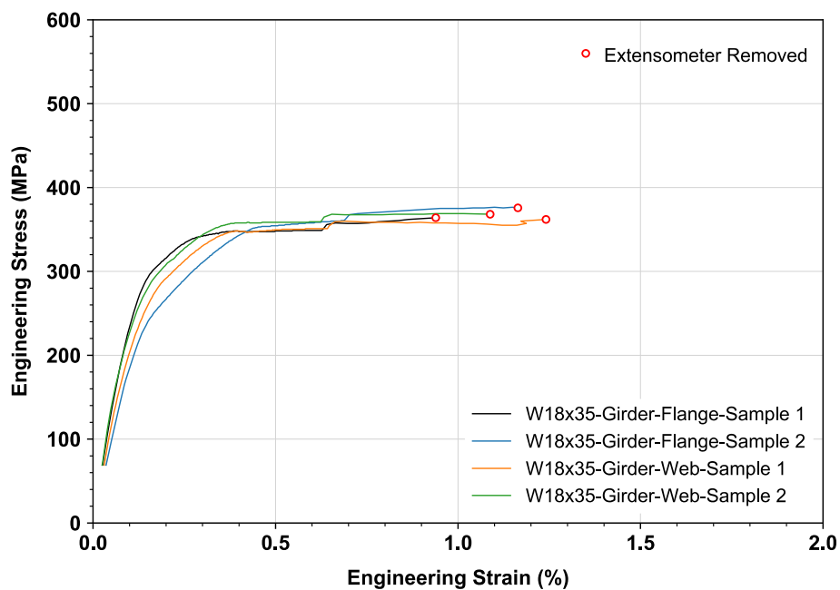
Fig. 2-28. Engineering stress-strain relationship for (a) W16x31 beam (b) W18x35 girder.
