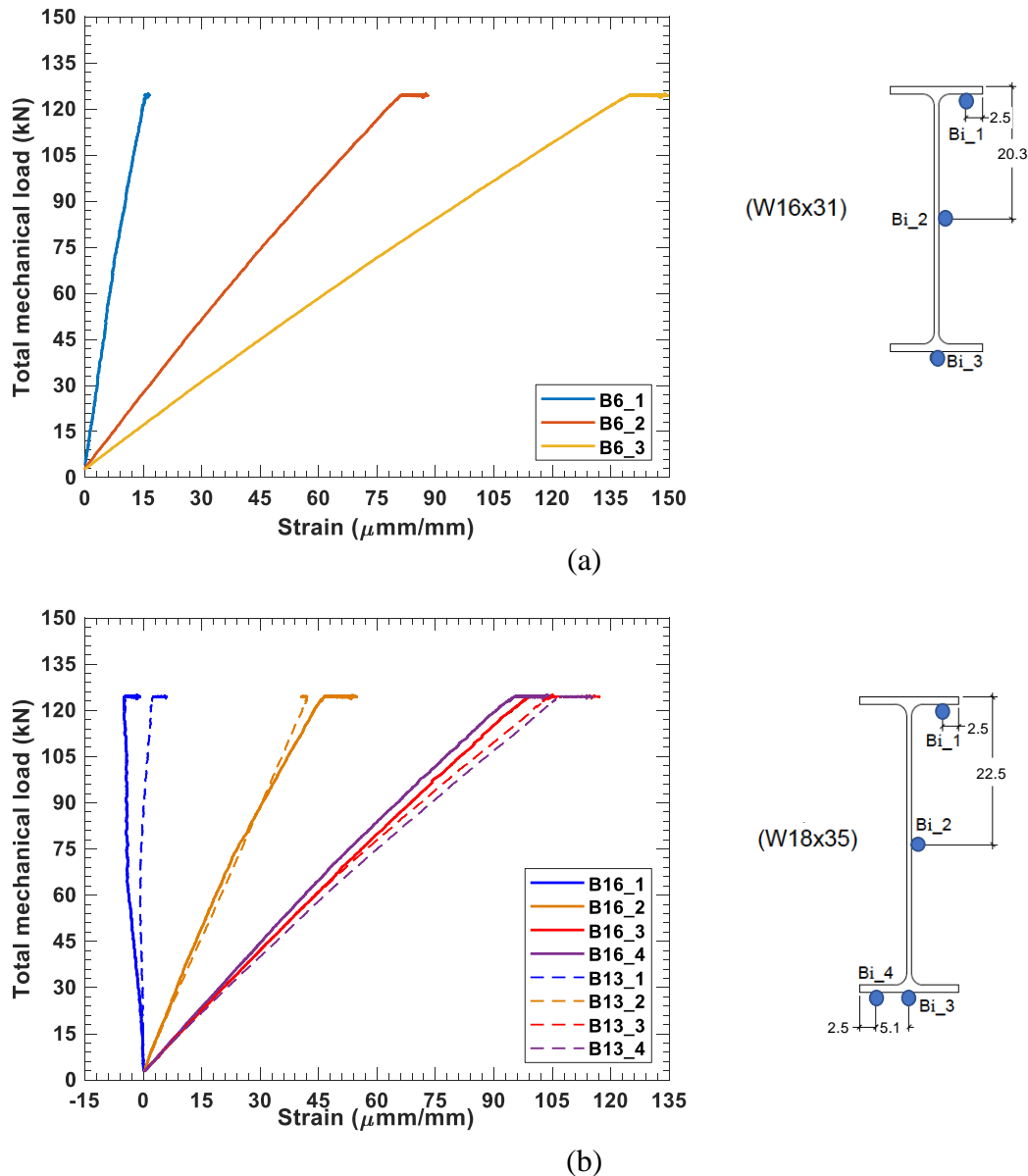
Fig. B-2. Measured beam strains during mechanical loading at ambient temperature: (a) secondary (W16x31) beam; east and west (W18x35) girders at midspan.
