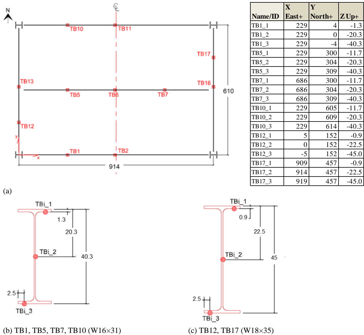
Fig. B-15. Locations of (a) steel temperature measurements where the Z datum is located at top of the steel members and thermocouples mounted to (b) W16×31 beams (TB1, TB5, TB7, and TB10 sections) and (c) W18×35 girders (TB12 and TB17 sections). i = section number shown in (a).
