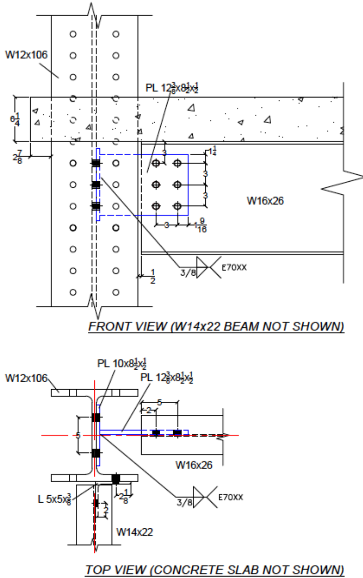
Fig. 2-7. Connection detail of column C1. Units are in inches.
