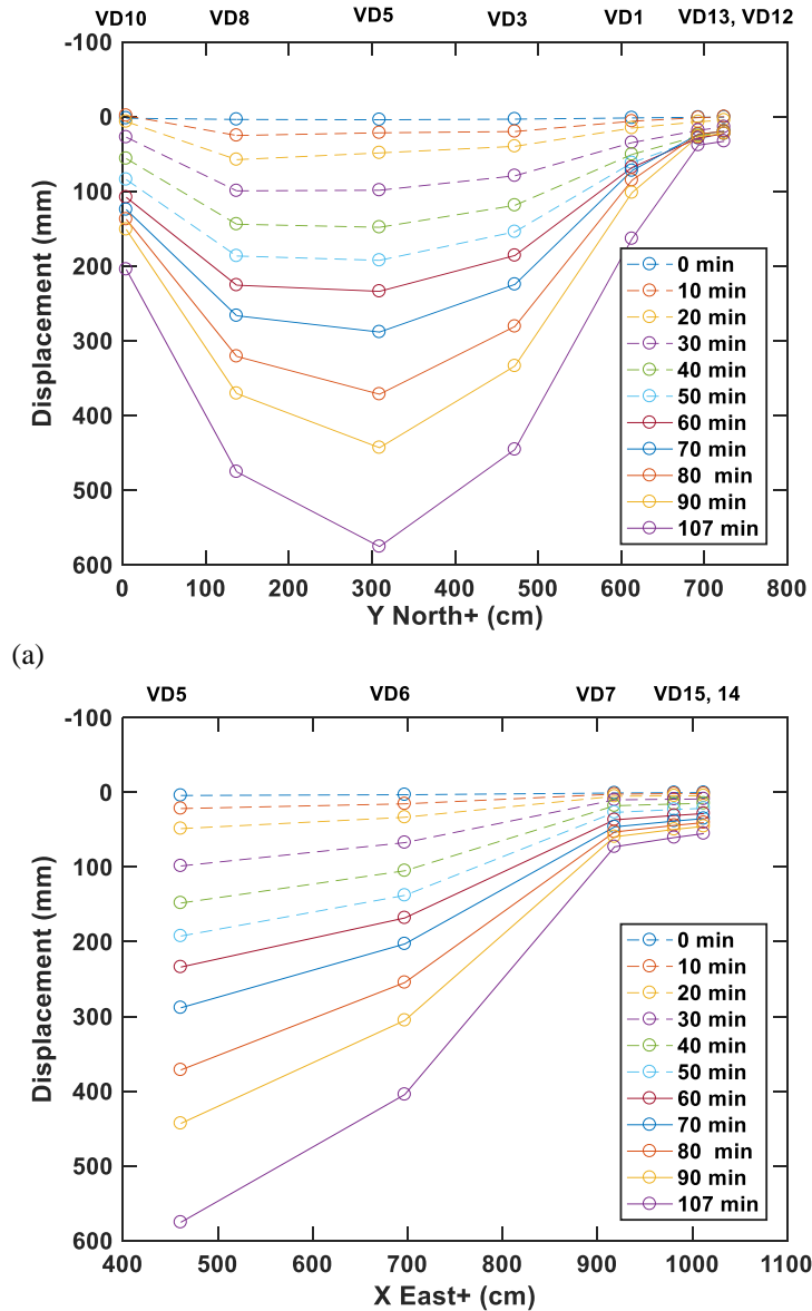
Fig. 4-33. Vertical displacement profile of the test floor assembly at (a) the north-south centerline and (b) the east-west centerline. The upper horizontal axes indicate the corresponding position of each vertical displacement sensors.
