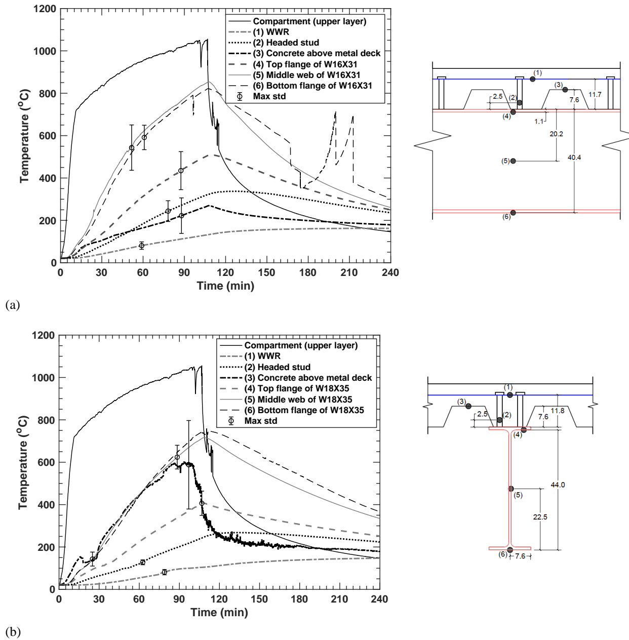
Fig. 4-19. Average temperatures of (a) 9.1 m long composite beams at midspan and (b) 6.1 m long composite girders at midspan. Error bars indicate the maximum variation in temperatures recorded using thermocouples mounted at the same height during fire loading. Thermocouple locations are in cm.
