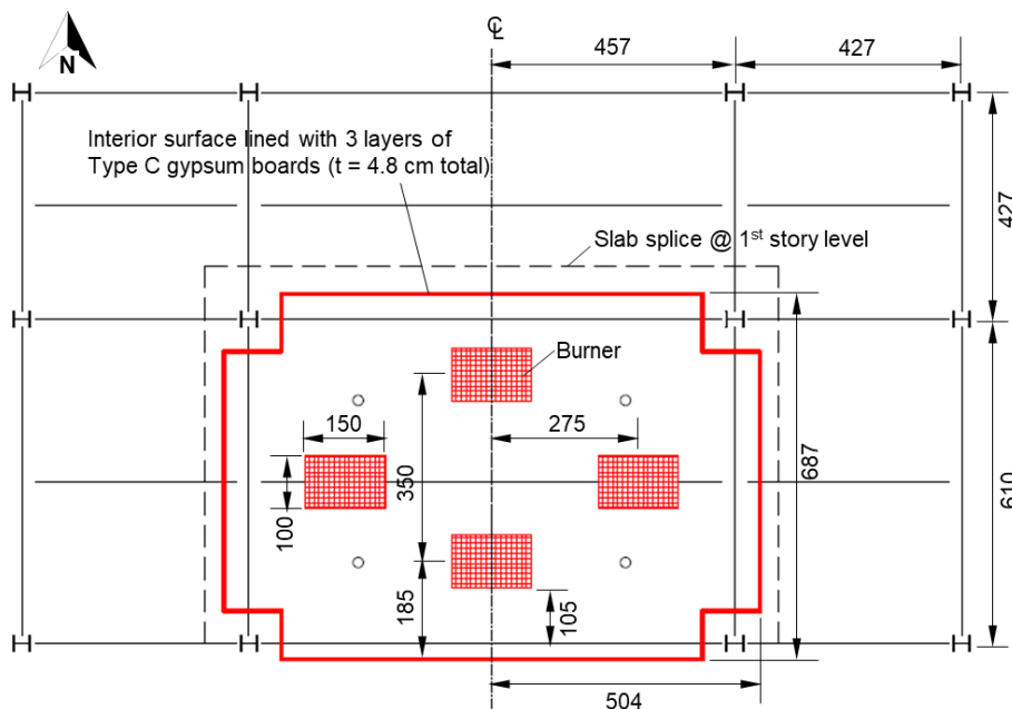
Fig. 2-32. Floor plan with the fire test compartment and distribution of burners. (Unit in cm).
