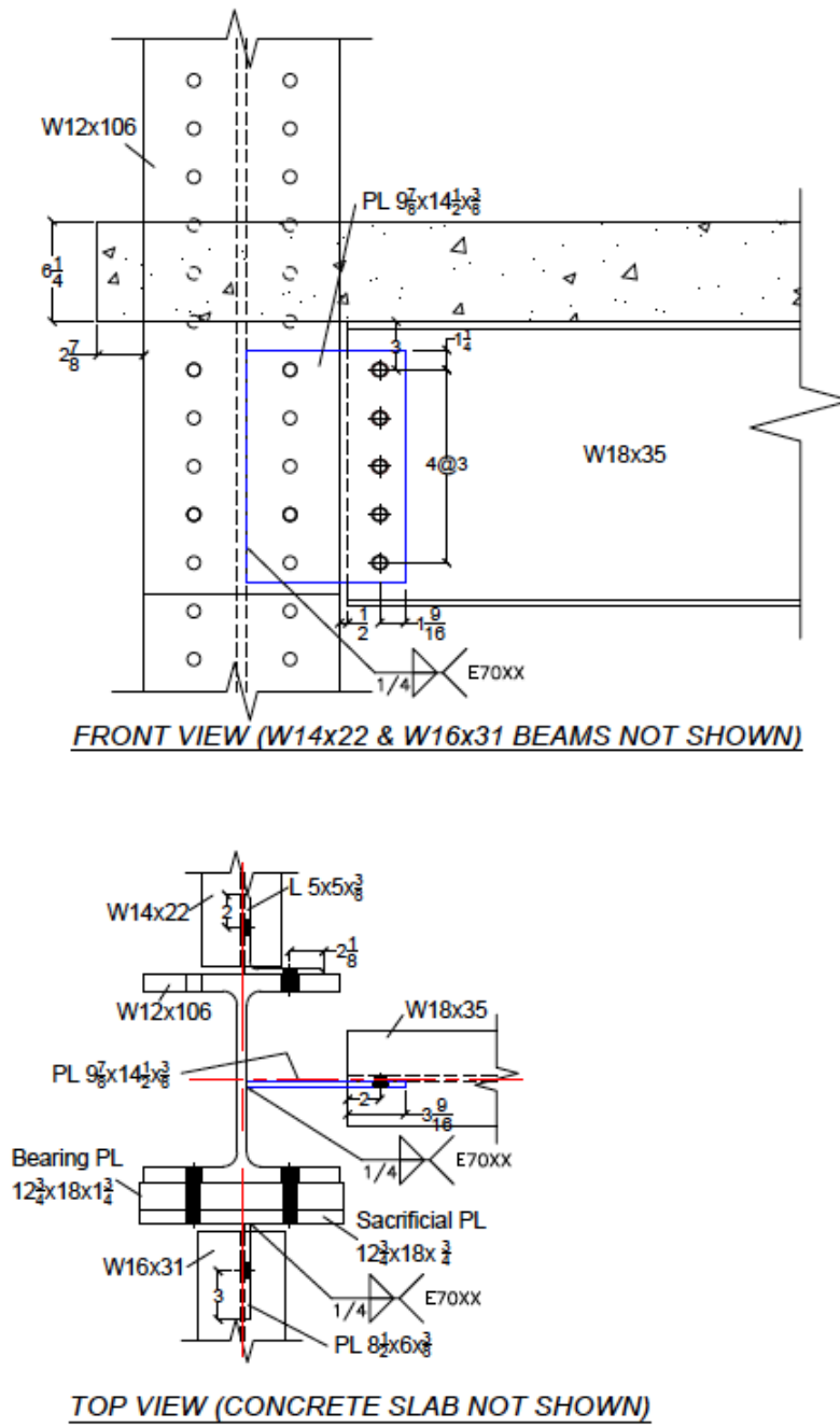
Fig. 2-6. Connection detail of column C2. Units are in inches.
