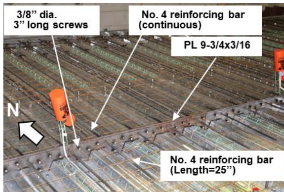
Fig. 2-19. Slab splice (a) west or east side (b) north side.
