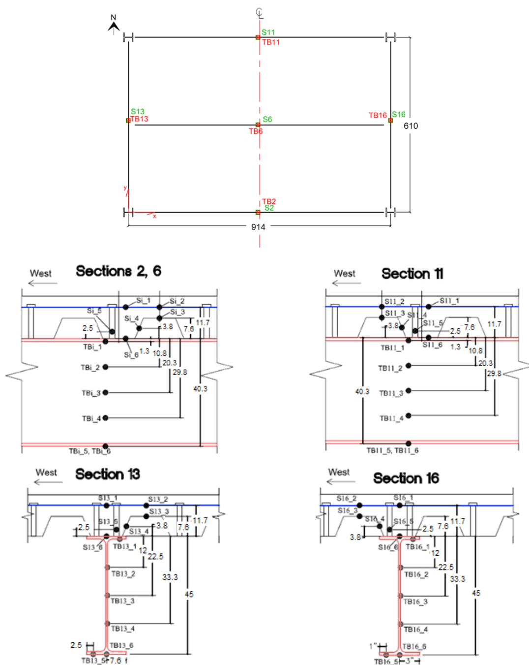
Fig. B-11. Locations of thermocouples mounted at the midspan composite sections, where i is the section number.
