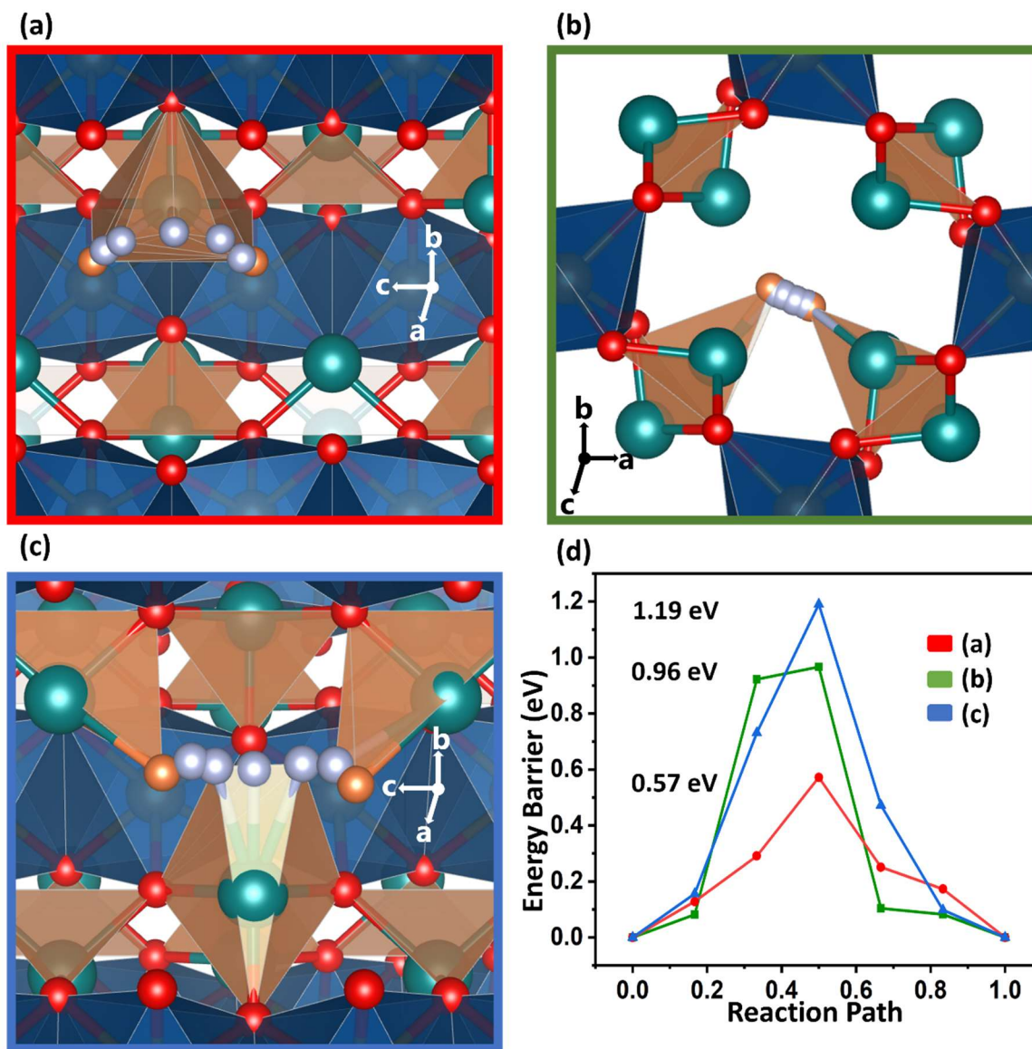
Figure S9. Nudged elastic band (NEB) calculations for possible fluoride-ion diffusion pathways in FeSb 2 O 4 . (a-c) show three distinct diffusion pathways adopted by the fluoride-ions inside the 1D tunnels defined by interconnected FeO 6 octahedra and SbO 3 tetrahedra in FeSb 2 O 4 . (d) NEB-calculated diffusion barriers for fluoride-ion diffusion pathways shown in (a-c).
