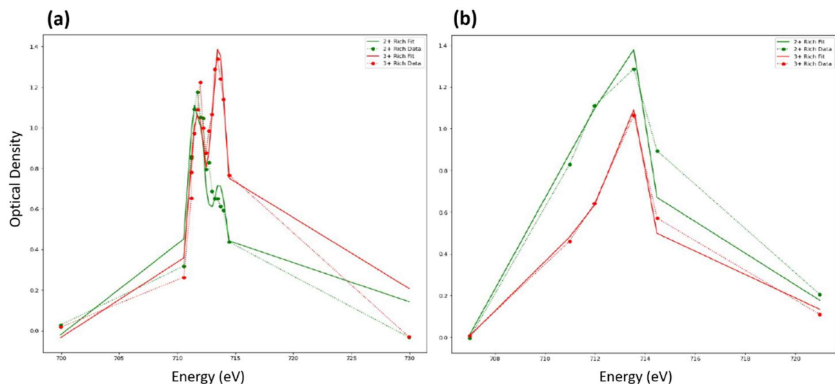
Figure S3. Linear fitting results for the ptychography data based on reference spectra shown in Figure S4. (a) Linear fitting results for data shown in Figure 3a. (b) Linear fitting results for data shown in Figure 3b.
