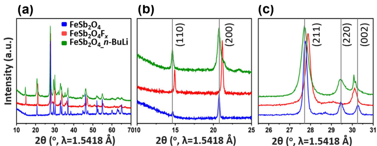
Figure S1. Structural characterization of FeSb 2 O 4 upon fluoridation (a) Comparison of powder X-ray diffraction data collected for FeSb 2 O 4 , FeSb 2 O 4 F x ( x \approx 1 ), and FeSb 2 O 4 recovered after treatment with n-butyllithium. Expanded views showing evolution of (b) the (110) and (200) reflections and (c) the (211), (220), and (002) reflections across the F-ion insertion and deinsertion reactions. 1 Adapted with permission from Zaheer, W., Andrews, J. L., Parija, A., Hyler, F. P., Jaye, C., Weiland, C., Yu, Y. S., Shapiro, D. A., Fischer, D. A., Guo, J., et al. (2020). Reversible Room-Temperature Fluoride-Ion Insertion in a Tunnel-Structured Transition Metal Oxide Host. ACS Energy Lett. 5, 2520–2526. 10.1021/acsenergylett.0c01328. Copyright 2021 American Chemical Society.
