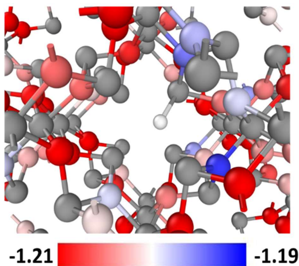
Figure S8. Bader Charge Analysis of \text{FeSb}_2\text{O}_4\text{F}_x . (a) The net charge on O atoms in \text{FeSb}_2\text{O}_4\text{F}_x (F = white, Fe and Sb = grey, and O = charge scale).
