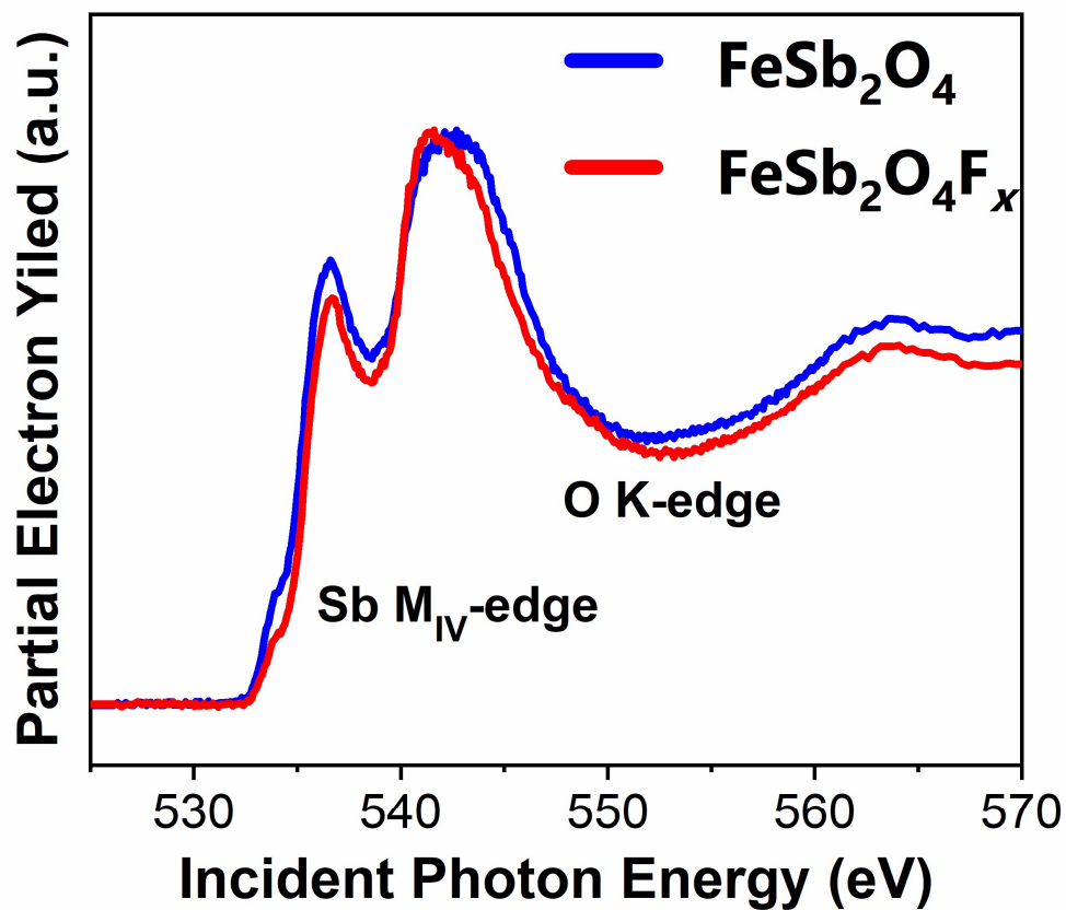
Figure S7. XANES spectra acquired at the Sb M_{IV} - and O K-edges of \text{FeSb}_2\text{O}_4 and \text{FeSb}_2\text{O}_4\text{F}_x ( x \approx 1 ).
