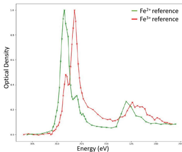
Figure S4. Reference spectra for Fe 2+ and Fe 3+ used for linear fitting ptychography data. 2 Adapted from Farmand, M., Celestre, R., Denes, P., Kilcoyne, A. L. D., Marchesini, S., Padmore, H., Tyliszczak, T., Warwick, T., Shi, X., Lee, J., et al. (2017). Near-Edge X-Ray Refraction Fine Structure Microscopy. Appl. Phys. Lett. 110 , 1-5. 10.1063/1.4975377. with permission of AIP Publishing.
