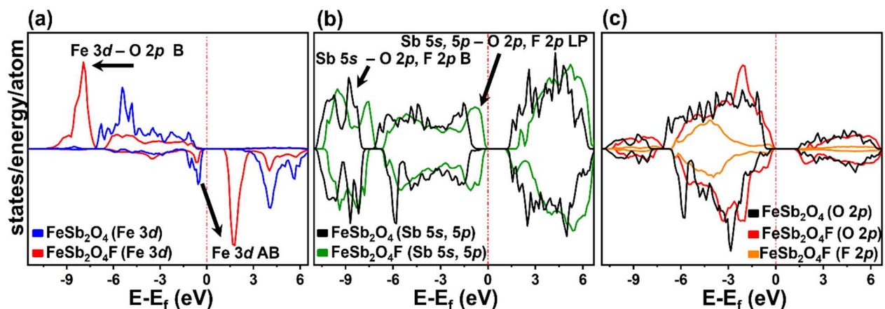
Figure S6. Comparison of atom-projected density of states for Fe, Sb, O, and F (a) Spin-polarized atom-projected partial density of states obtained from DFT calculations for Fe in \text{FeSb}_2\text{O}_4 and \text{FeSb}_2\text{O}_4\text{F} . (b) Sb atom-projected partial density of states for \text{FeSb}_2\text{O}_4 and \text{FeSb}_2\text{O}_4\text{F} . (c) O atom-projected partial density of states for \text{FeSb}_2\text{O}_4 and O, F atom-projected partial density of states for \text{FeSb}_2\text{O}_4\text{F} .
