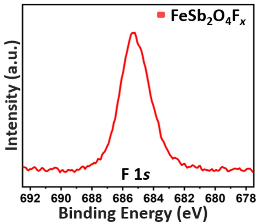
Figure S2: HAXPES spectrum for F 1s in FeSb 2 O 4 F x collected at an incident photon energy of 5.0 keV.
