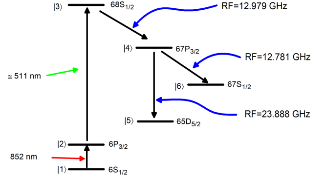
FIG. 10. Six-level scheme used to model the experimental data.
