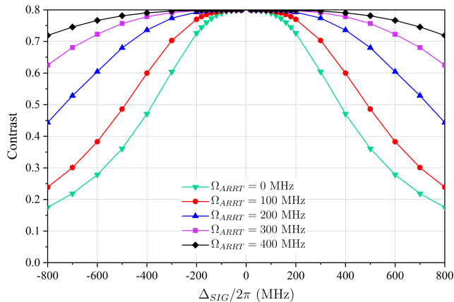
FIG. 13. Maximum EIT height change (from Fig. 12) reported as contrast (Eq. 15) for a set of SIG and ARRT Rabi frequencies ( \Omega_{SIG} and \Omega_{ARRT} , respectively) over a wide range of SIG detunings ( \Delta_{SIG} ). Increased contrast relates to an increase in sensitivity to the detuned SIG field.
