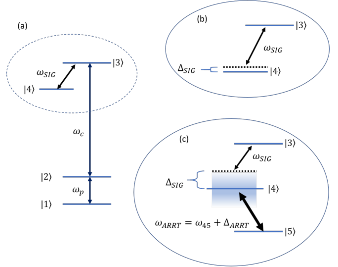
FIG. 1. (a) Typical 4-level EIT/AT scheme where \omega_p and \omega_c are the optical probe and pump fields and \omega_{SIG} is the RF signal that causes AT splitting for detection. (b) The RF field can be detuned over a small range from the |3\rangle - |4\rangle transition and still cause AT splitting. (c) This range can be extended by coupling to an adjacent resonance, |4\rangle - |5\rangle .
