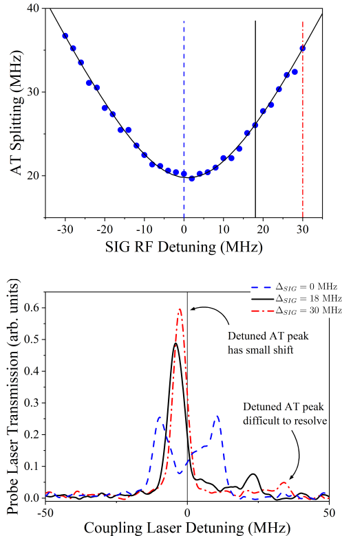
FIG. 2. RF detuning: (top) AT splitting as a function of RF detuning and (bottom) EIT signal for several RF detunings. As the detuning increases, one AT peak shifts further away and reduces in amplitude, while the other shifts back towards the zero field case. Uncertainty in the AT splitting measurements are on the order of 1 MHz.
