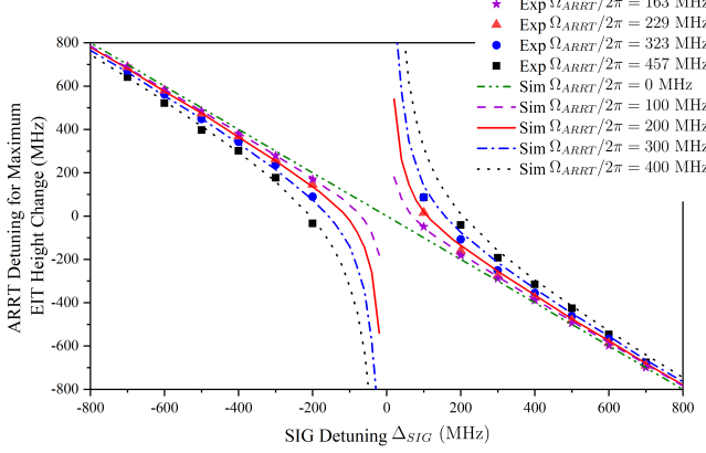
FIG. 12. Repeat of Fig. 9 with more \Omega_T measurements and compared to the model calculations. The experimental measurements show an asymmetry with the sign of \Delta_{SIG} , suggestive of a frequency shifting that the model does not capture, whereas the model does demonstrate the divergent trend as the SIG approaches the on-resonant condition (where the ARRT field is no longer beneficial).
