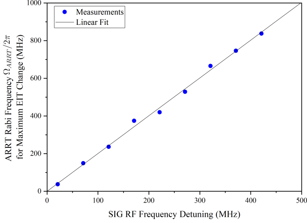
FIG. 8. The ARRT field Rabi frequency \Omega_{ARRT} for maximum sensitivity increases linearly with SIG field detunings \Delta_{SIG} .
