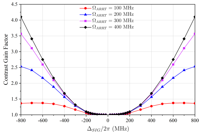
FIG. 14. Numerically modeled contrast gain factor (Eq. 16) for a set of ARRT field Rabi frequencies ( \Omega_T ) over a wide range of SIG field detunings ( \Delta_{SIG} ) showing increased sensitivity gain for strong ARRT fields and highly detuned SIG fields.
