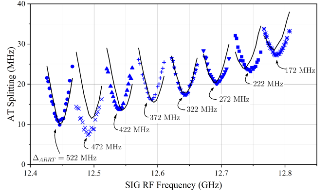
FIG. 4. SIG detuning \Delta_{SIG} for various values of \Delta_{ARRT} . Each parabola represents a different value of \Delta_{ARRT} , while the AT splitting was measured as \Delta_{SIG} was swept. Each one follows the same function as the zero-detuning case in Fig. 2 (top), where the AT splitting is a minimum on resonance. This shows that there is an apparent resonance condition that is shifted by applying the ARRT field. A description of the numerical model used to generate the simulated results (solid lines) is given in Section IV.
