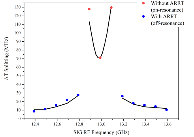
FIG. 11. Comparison of simulations (black lines) to experimental data (red and blue dots) in Fig. 5, from the SIG transition 68 S_{1/2} - 67 P_{3/2} using an ARRT field near 67 P_{3/2} - 65 D_{5/2} . The AT splittings are predicted well by theory.
