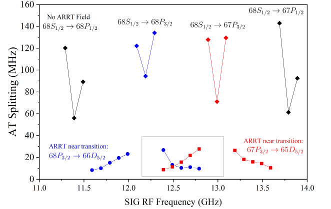
FIG. 5. Measurements of the AT splitting by a SIG field from both direct resonances (diamonds) and with an ARRT field (squares and circles). The blue circles are AT splittings enabled by applying an ARRT field near the 68 P_{3/2} - 66 D_{5/2} transition to shift the 68 P_{3/2} state, and the red squares were made using an ARRT field near the 67 P_{3/2} - 65 D_{5/2} transition to shift the 67 P_{3/2} state. This shows that the application of an appropriate adjacent resonance field can enable resonant detection over a continuous frequency range spanning several Rydberg states.
