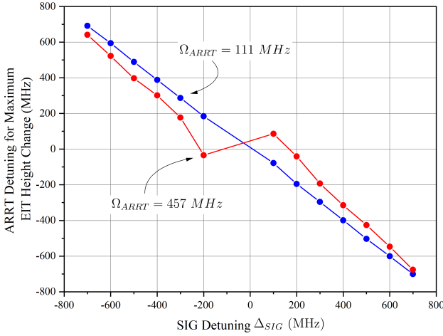
FIG. 9. ARRT field detuning \Delta_{ARRT} is varied to maximize response to various SIG field detunings \Delta_{SIG} , for two ARRT field strengths. For a weak ARRT field, optimal \Delta_{ARRT} varies linearly with the detuning of the SIG field. For a strong ARRT field, optimal \Delta_{ARRT} is reduced, and becomes non-linear. The asymmetry is likely due to an AC stark shift caused by the strong ARRT field.
