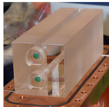
Figure 1: Fixed Length Optical Cavity (FLOC) will replace all mercury Manometers
