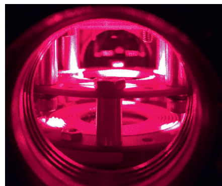
Figure 2: CAVS small portable version NIST prototype with a cloud of trapped Li atoms.
