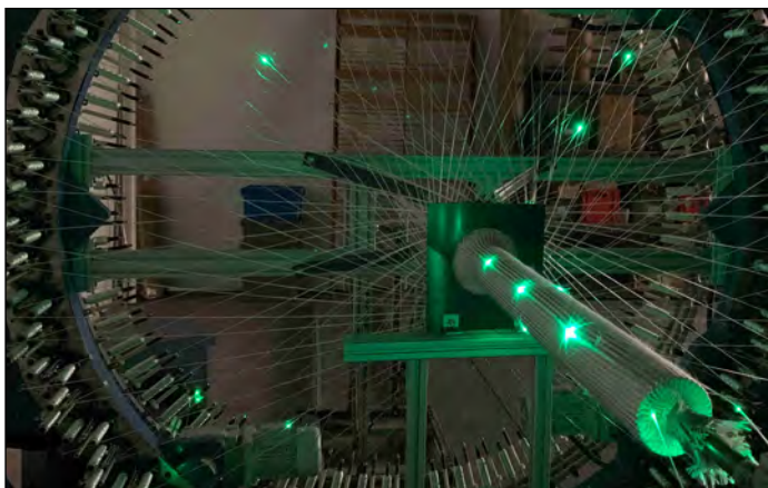
AFFOA member company Revolution Composites integrated LED fibers in their fiberglass reinforced epoxy composites through a braiding and resin transfer molding process. Credit: Revolution Composites.
