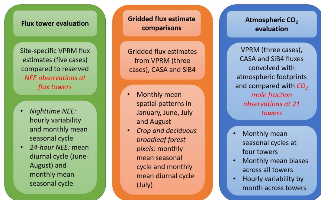
Figure 4. Diagram of planned analyses for VPRM flux evaluation. Each color box delineates a particular type of evaluation (in terms of data sets and scale of analysis), with the second row of sub-boxes describing the model runs and observations, and the third row describing each set of analyses.
