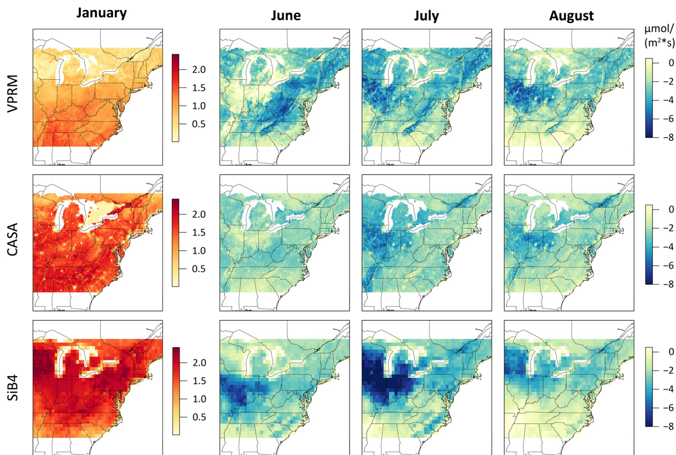
Figure 8. Monthly mean gridded NEE at 0.1^\circ for \text{VPRM}_{\text{new}} , CASA, and SiB4 in January, June, July, and August. Corresponding plots comparing \text{VPRM}_{\text{new}} , \text{VPRM}_{\text{seas}} , and \text{VPRM}_{\text{ann}} are shown in Figure S7 in Supporting Information S1.
