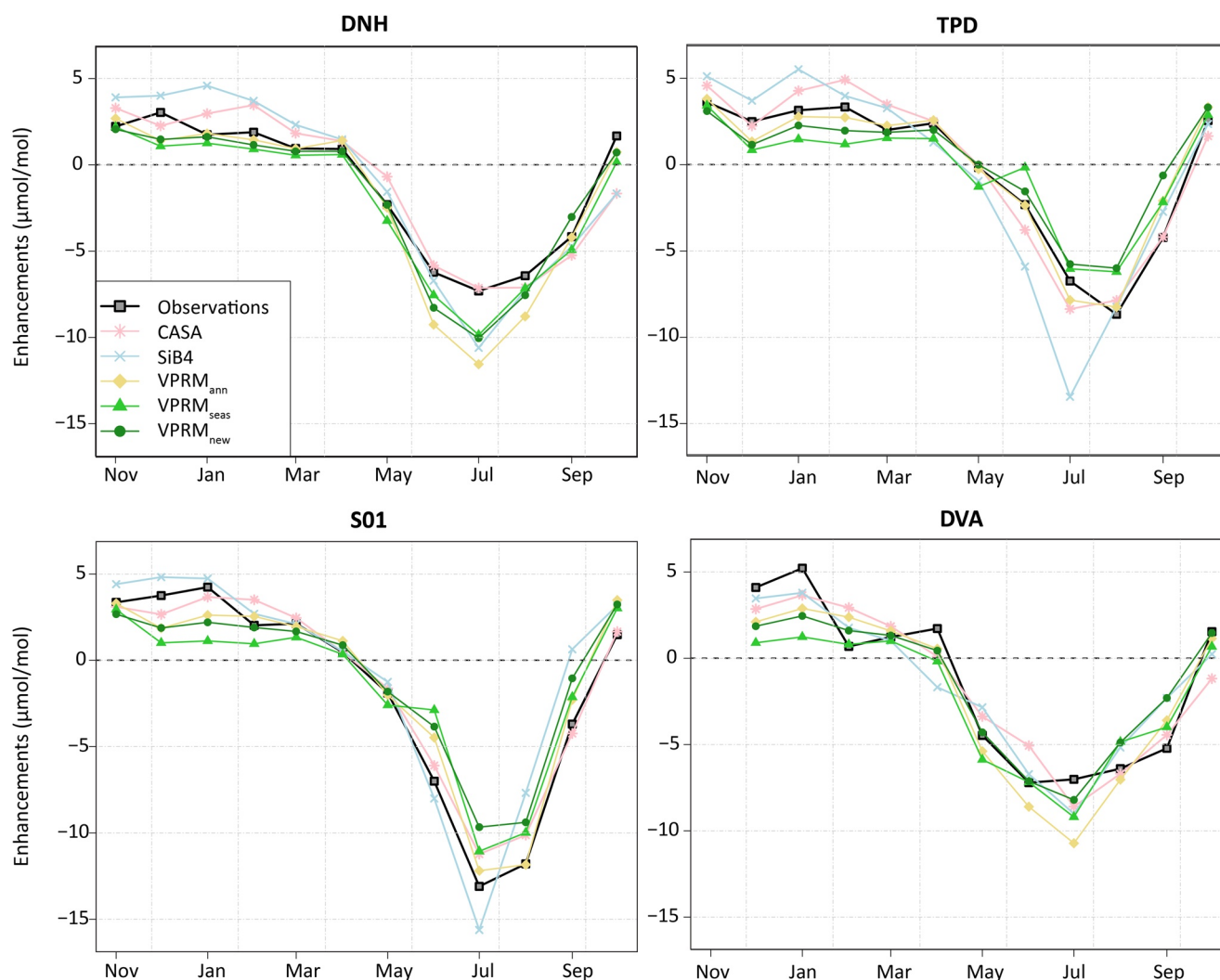
Figure 10. Monthly mean simulated and observed biological atmospheric CO 2 enhancements for VPRM new , VPRM seas , VPRM ann , CASA, and SiB4 at four towers: DNH in New Hampshire, TPD in Ontario, Canada, S01 in Indiana, and DVA in Virginia. Enhancements are determined using averaged convolutions with WRF-STILT and NAMS-STILT transport, “optimal” monthly background conditions, and Vulcan 3.0 + FFDAS fossil fuel emissions. The same figures using WRF-STILT and NAMS-STILT transport alone are shown in Figures S11 and S12 in Supporting Information S1.
