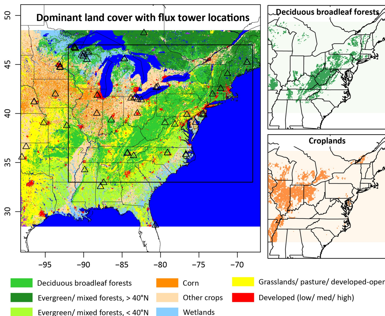
Figure 1. Map of dominant land cover at 0.02° resolution for eight plant functional types (PFTs), with a rectangle around the flux simulation domain (left panel). (The shrubland PFT is not shown here because it is not the dominant land cover for any pixel at this spatial resolution.) Also shown are the locations of the 69 flux towers included in the parameter optimization (Table S1 in Supporting Information S1). Deciduous broadleaf forest and cropland pixels used for spatial aggregation of gridded fluxes are shown in the panel on the right at 0.1°, where these pixels contain more than 50% coverage in the underlying land cover maps for VPRM and CASA, and 25% coverage for SiB4 at 0.5°.
