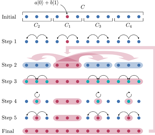
FIG. 1. A demonstration of our protocol for encoding a qubit into a GHZ-like state in a one-dimensional system C . Initially, the unknown coefficients a, b are encoded in one qubit (red circle) while the other qubits are each initialized in state |0\rangle . The first step of the protocol assumes the ability to encode information into GHZ-like states in subsystems C_1, \dots, C_4 using, for example, nearest-neighbor interactions. In step 2, we apply a generalized controlled-phase gate [Eq. (6)] between the subsystems to “merge” the GHZ-like states into an entangled state between all sites. The last three steps rotate this entangled state into the desired GHZ-like state by concentrating the entanglement in each subsystem onto one qubit, applying single-qubit rotations, and redistributing the entanglement to the rest of the system. Repeatedly feeding the resulting GHZ-like state back into step 2 of the protocol yields larger and larger GHZ-like states.
