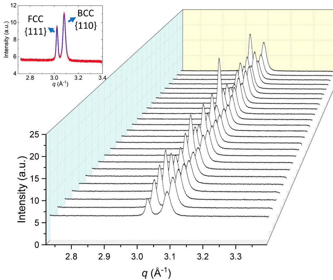
Figure 3. Spatially resolved, in-house XRD data of as-built 17-4 sample with a finely polished surface. For clarity, only the data within a q range of 2.7 \text{ \AA}^{-1} and 3.4 \text{ \AA}^{-1} are shown. The inset shows the indexing of these two peaks as FCC {111} and BCC {110}, respectively.
