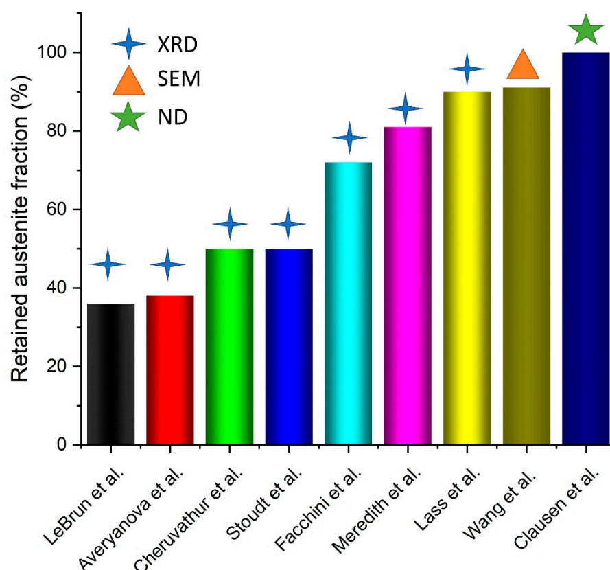
Figure 1. An incomplete set of phase fraction of retained austenite in as-built 17-4 steel, identified in literature. The measurement technique is specified by the symbols on the top of the individual columns. XRD stands for XRD results acquired using in-house X-ray diffractometer. SEM results are acquired from EBSD. ND stands for neutron diffraction.
