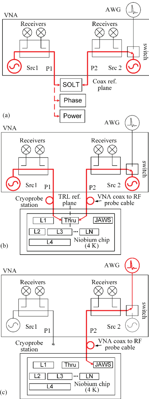
Fig. 2a) First-tier VNA calibration using SOLT, power and phase standards. b) Second-tier VNA calibration using broadband on-wafer multiline TRL kit. c) JAWS measurements, with AWG driving signal passed through the VNA.
