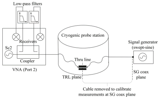
Fig. 3 Simple control experiment used to verify the calibration.
