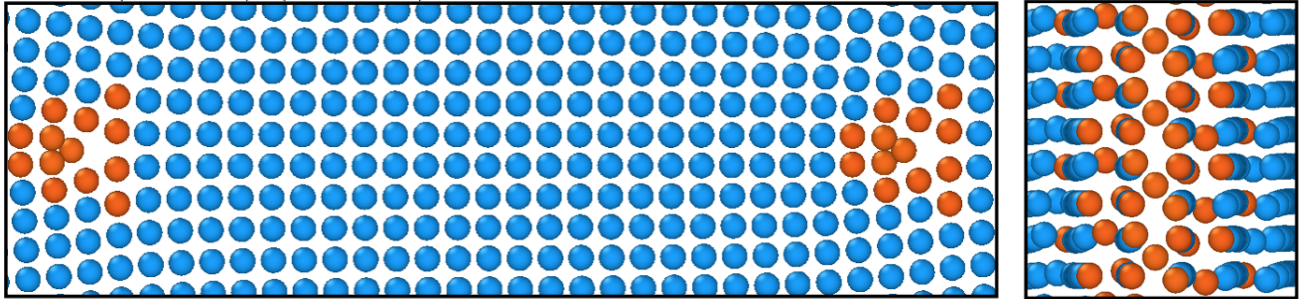
Figure 13: Structures of symmetrical tilt GBs in Si. The structures are projected parallel to the [001] tilt axis (left) and normal to the tilt axis (right)
