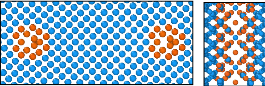
Figure 6: Structures of symmetrical tilt GBs in Si. The structures are projected parallel to the [001] tilt axis (left) and normal to the tilt axis (right)
