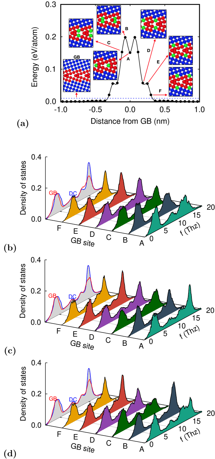
Figure 4: (a) Selected atomic sites (shown in green and labeled A through F) in the (210) GB at 1600 K. The sites are ranked according to the distance from the GB center and their energy is plotted as a function of this distance. The lines are drawn to highlight the trends. Panels (b), (c) and (d) show the vibrational density of states of the selected GB sites in the x, y, and z directions, respectively. The projection on the DOS frequency plane shows the overall DOS of the GB core in the respective direction in comparison with that of diamond cubic (DC) Si.
