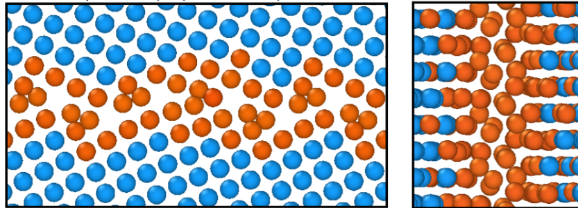
Figure 9: Structures of symmetrical tilt GBs in Si. The structures are projected parallel to the [001] tilt axis (left) and normal to the tilt axis (right)
