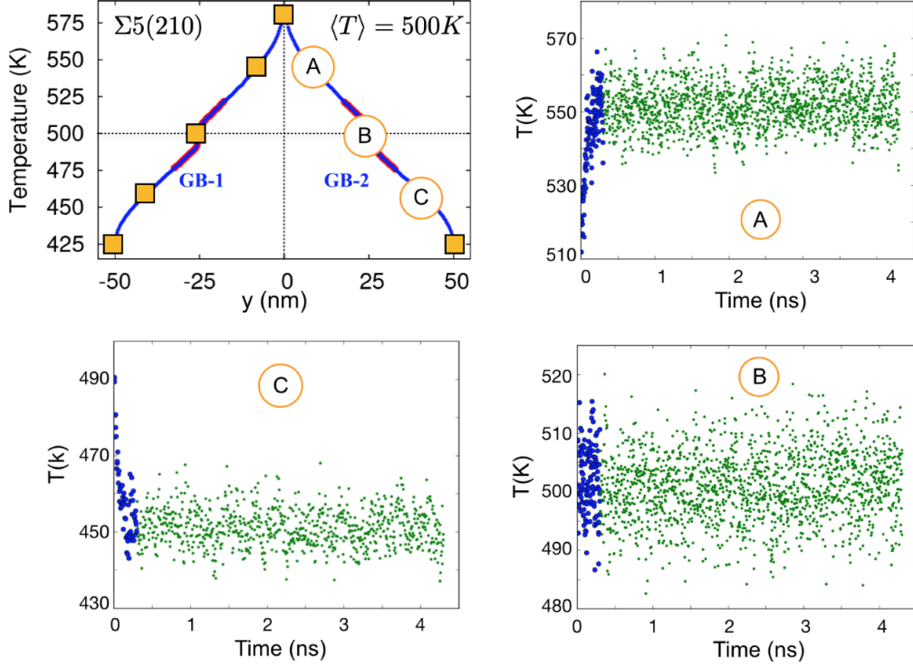
Figure 1: Example of local temperature convergence plots used to verify that the system had reached a steady-state regime.
