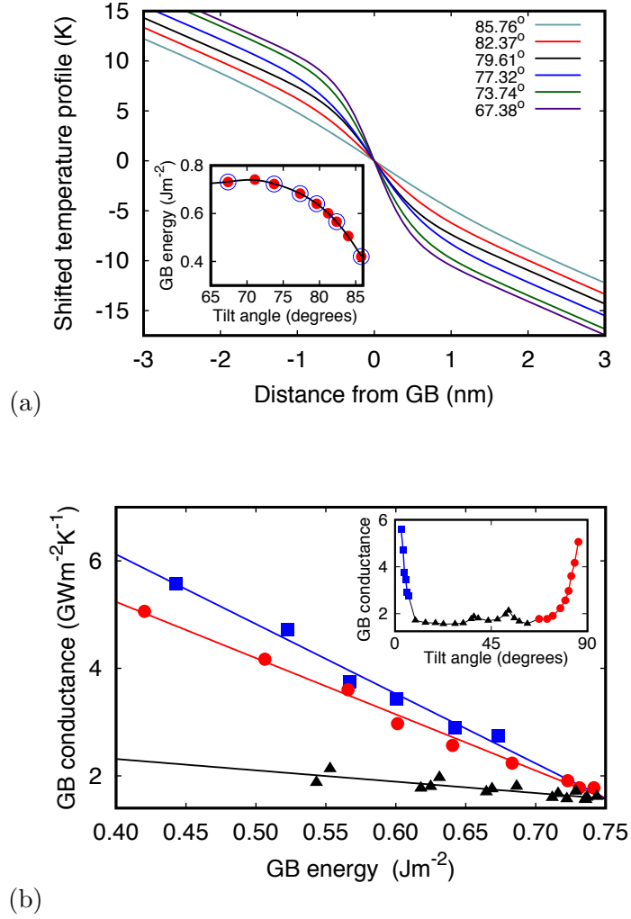
Figure 9: (a) Temperature profiles for low-angle (relative to 90^\circ ) GBs at 750 K. The profiles were fitted by Eq.(4) and shifted to zero by subtracting the average temperature of the simulation block. (b) Kapitza conductance of all GBs studied in this work as a function of GB energy at 750 K. Note that the results naturally break into three groups as discussed in the text. The lines represent linear fits intended to highlight the trends. The inlays show the plots of the GB conductance \sigma_K versus the tilt angle.
