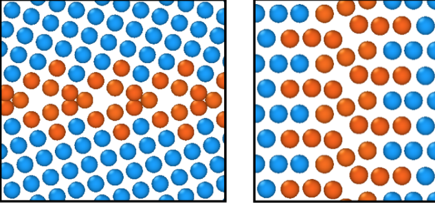
Figure 10: Structures of symmetrical tilt GBs in Si. The structures are projected parallel to the [001] tilt axis (left) and normal to the tilt axis (right)
