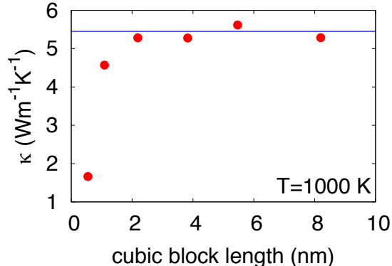
Figure 3: The dependence of thermal conductivity on block size for the Green-Kubo method
