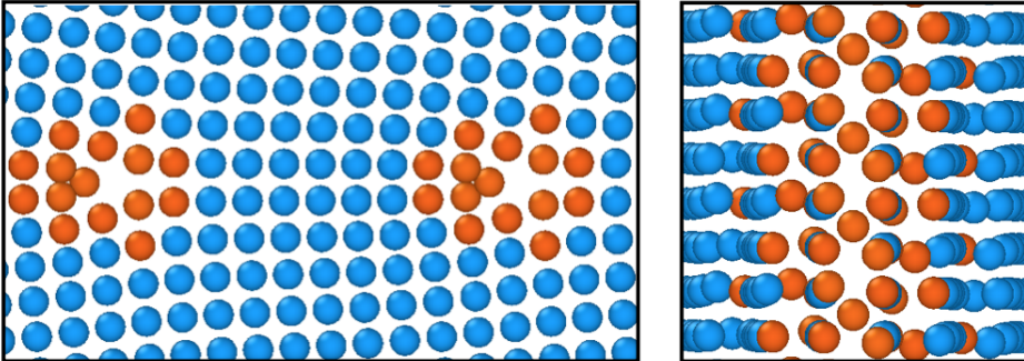
Figure 12: Structures of symmetrical tilt GBs in Si. The structures are projected parallel to the [001] tilt axis (left) and normal to the tilt axis (right)
