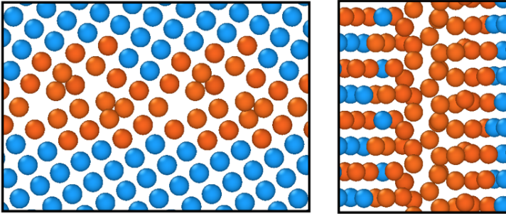
Figure 8: Structures of symmetrical tilt GBs in Si. The structures are projected parallel to the [001] tilt axis (left) and normal to the tilt axis (right). Note: The structure for the (510) has been extensively studied in the literature and there are at least twelve recognized structures [1, 6]. In [1] the structure for the (510) boundary used in this work was denoted (structure-b) and was seen to be the second lowest energy structure out of eight possible (510) structures. It is possible that our GB minimization search was unable to find the minimum energy structure or that the discrepancy is a result of the different interatomic potentials being used.
