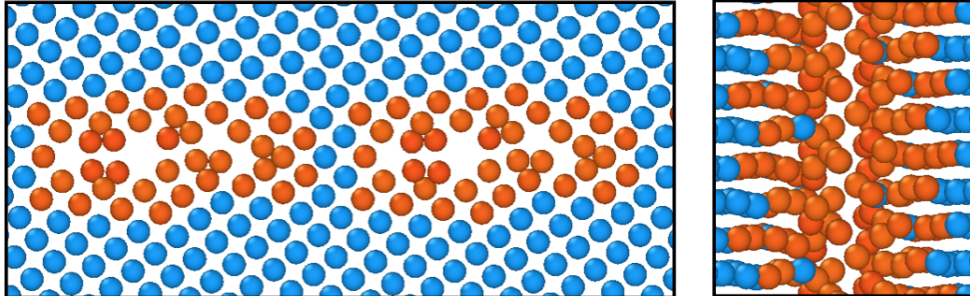
Figure 7: Structures of symmetrical tilt GBs in Si. The structures are projected parallel to the [001] tilt axis (left) and normal to the tilt axis (right)
