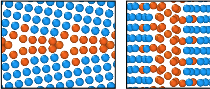
Figure 11: Structures of symmetrical tilt GBs in Si. The structures are projected parallel to the [001] tilt axis (left) and normal to the tilt axis (right)
