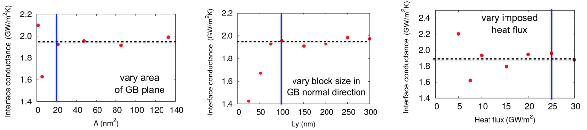
Figure 2: Plots showing the dependence of GB Kapitza conductance on block size and imposed heat flux
