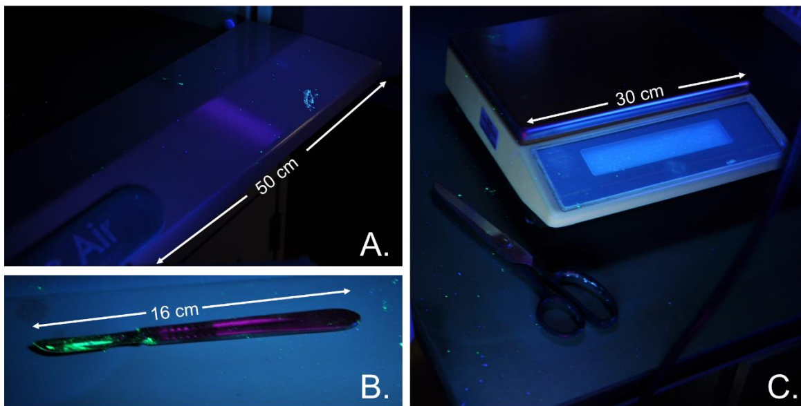
Figure 4. Photographs from the analysis and weighing of the simulant brick. (A.) Touch transfer of particulate to the exterior of the fume hood during analysis. (B.) Scalpel used to open the simulant brick. (C.) Particulate present around and on balance after taking a net weight. The flour / fluorescent powder mixture is the yellow fluorescing material.
