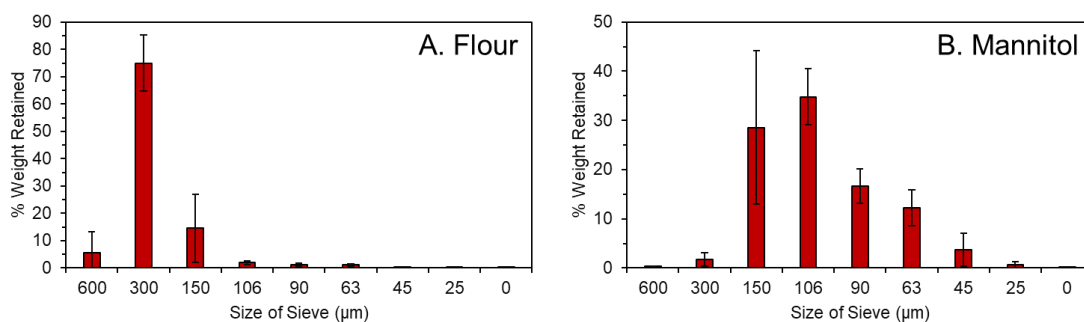
Figure 1. Particle size distributions for the flour (A.) and mannitol (B.) used in these experiments. Error bars represent the standard deviation of three replicate measurements.
