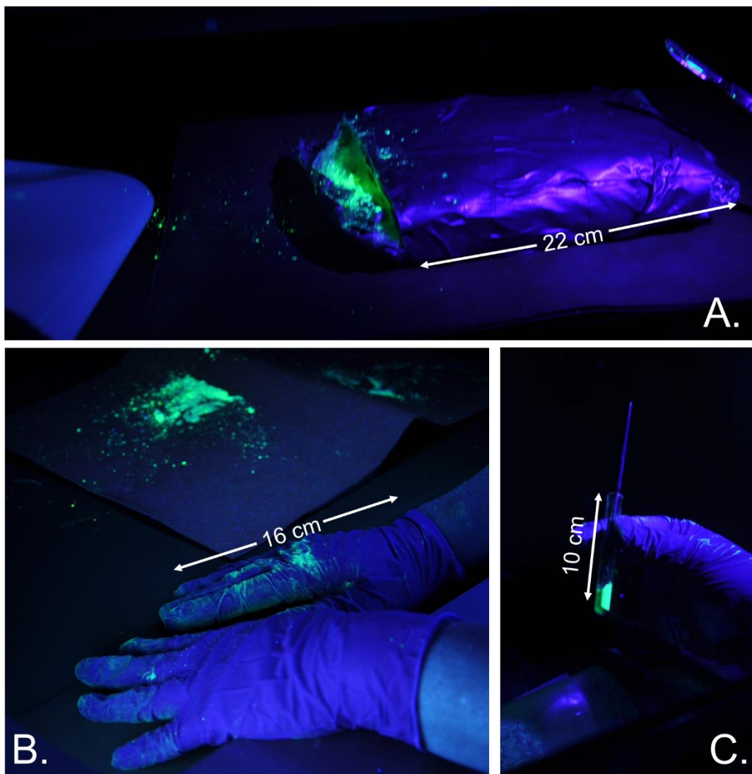
Figure 3. Photographs from the opening and analysis of the simulant brick. (A.) The brick after it has been cut open using a scalpel. (B.) Particulate transfer onto gloves after opening the brick. (C.) Transfer of a representative sample into a glass test tube. The flour / fluorescent powder mixture is the yellow fluorescing material.
