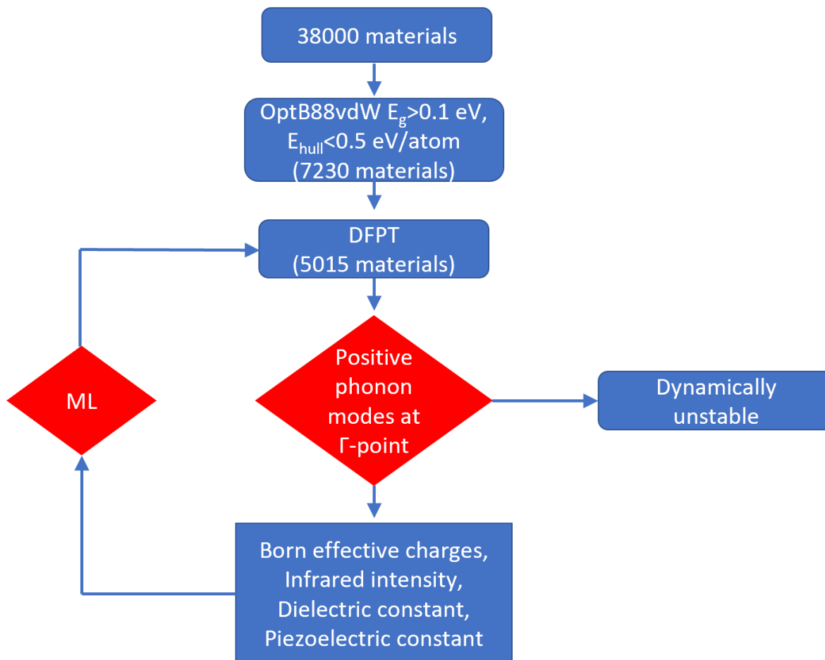
Fig. 1 Flow-chart portraying different steps for the DFT and ML methods.
