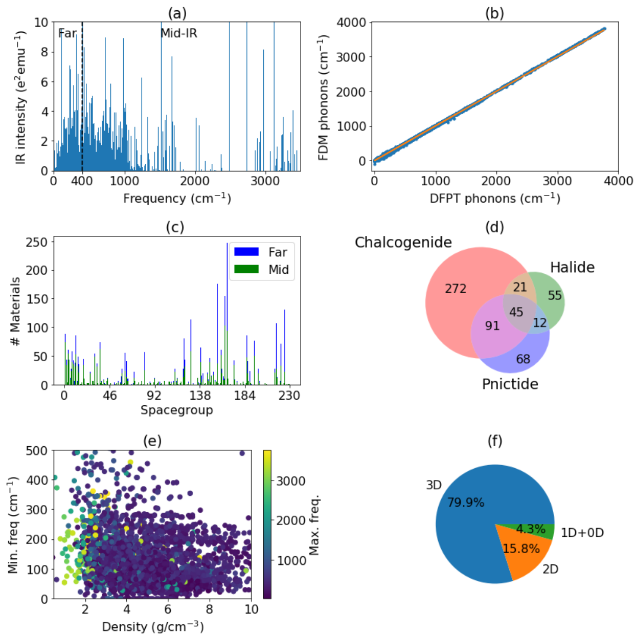
Fig. 2 Analysis of the IR-data. a) IR peaks for all the materials in the database, b) Comparison of finite-difference (FDM) and DFPT phonon frequencies for conventional cells, c) space-group distributions of materials with at least one far (blue) and mid (green) IR peaks, d) Venn-diagram of the chemistry of materials containing chalcogenides, halides, or pnictides, e) Minimum frequency vs density of the system, f) dimensionality analysis of the far-IR materials.
