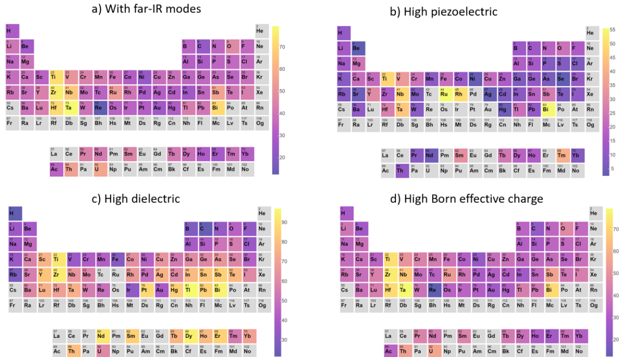
Fig. 7 Trends across the Periodic table of a) high IR peak (having at least one peak >400\text{ cm}^{-1} ), b) piezoelectric ( >1\text{ C/m}^2 ), c) dielectric ( >20 ) materials, and 2) max. Born-effective charge in a system ( >5 ) The elements in a material are weighed 1 or 0 if the material has high or low-values. Then the percentage probability of finding the element in a high-value material is calculated.
