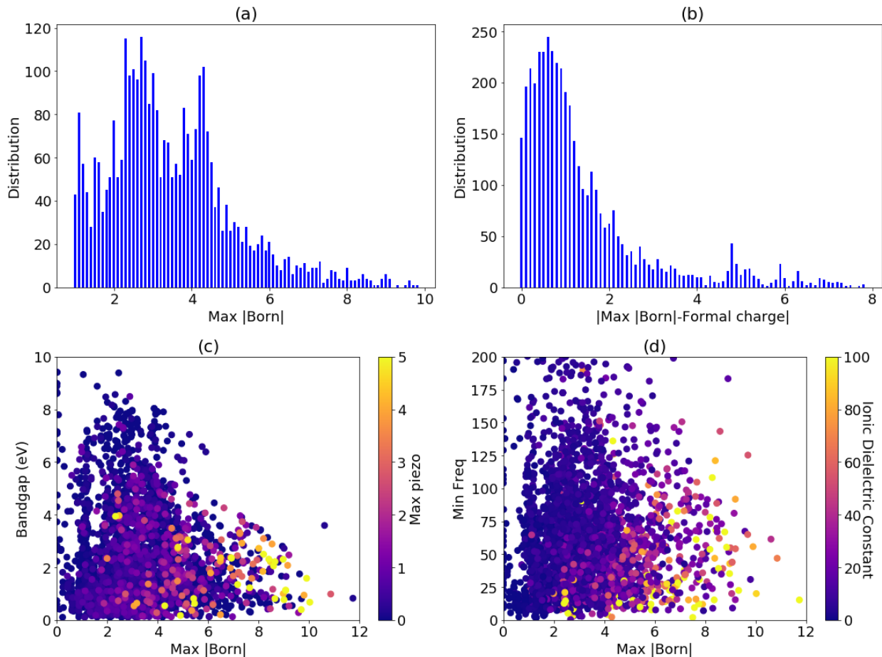
Fig. 6 Born effective charge distribution and its relation to PZ, DL and bandgaps. a) Histogram of Born-effective charge data, b) histogram of maximum BEC and formal charge c) BEC wrt bandgap with color-coded max PZ, d) BEC with respect to the min-IR-frequency with color-coded ionic part of dielectric constant.
