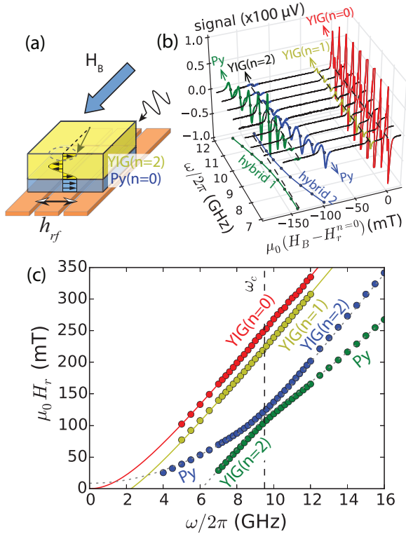
FIG. 1. (a) Illustration of the magnetization excitations in the YIG/Py bilayers with a coplanar waveguide. (b) Lineshapes of the YIG(100 nm)/Py(9 nm) sample for the first three resonance modes of YIG and the uniform mode of Py. The field axis is shifted so that the resonance field of the YIG( n=0 ) mode is zero. (c) Unshifted evolution of the four modes in (b). Curves show the fits as uncoupled modes. The vertical dashed line denotes where the YIG( n=2 ) and Py( n=0 ) modes cross on the frequency axis at \omega_c/2\pi = 9.4 GHz.
