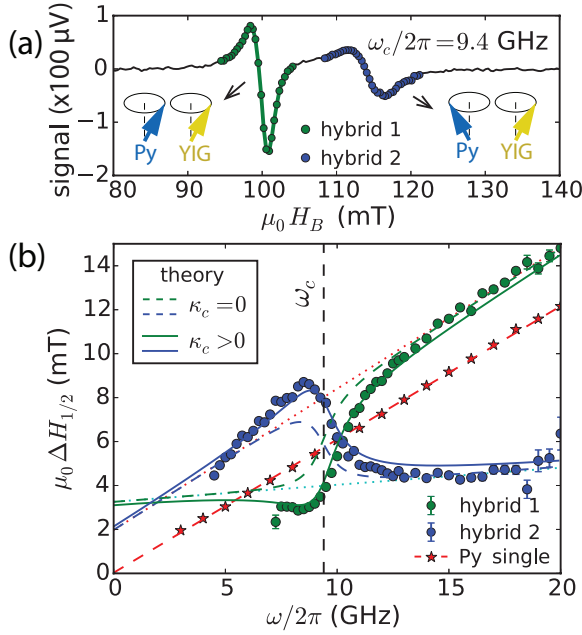
FIG. 2. (a) The lineshape of the YIG(100 nm)/Py(7.5 nm) sample at \omega_c/2\pi = 9.4 GHz, showing different linewidths between the two hybrid modes of YIG( n = 2 ) and Py( n = 0 ) resonances. (b) Linewidths of the two hybrid modes as a function of frequency. Dotted lines show the linear fit of the linewidths for the two uncoupled modes. Dashed curves show the theoretical values with \kappa_c = 0 . Solid curves show the fits with finite \kappa_c .
