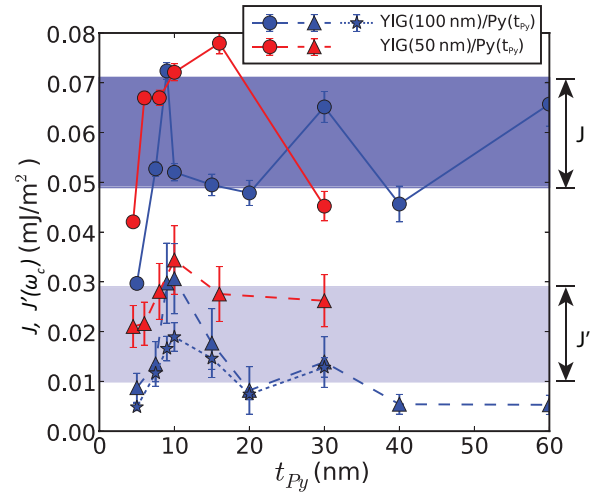
FIG. 4. Thickness dependence of J (circles) and J' (triangles), which are calculated from g_c and \kappa_c(\omega_c) , respectively. Blue points denote the results for YIG(100 nm)/Py( t_{Py} ) and red points for YIG(50 nm)/Py( t_{Py} ). The blue stars denote J'_{sp} , in which \Delta H_{sp}^{Py}(\omega_c) is calculated from the Py linewidth enhancement from Py( t_{Py} ) to YIG(100 nm)/Py( t_{Py} ). Error bars indicate single standard deviations found from the fits to the lineshape.
