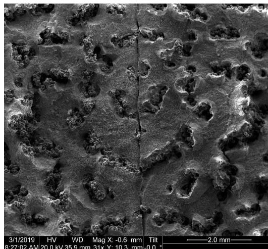
FIG. 9 Specimen SN-S-A: scanning electron microscope image of mating fracture surfaces.
