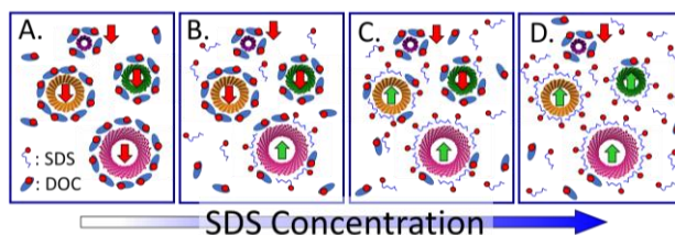
Figure 7. Simplified schematic of the hypothesized mechanism driving the selection of ATPE partition for each individual (n,m) species in the SDS-DOC competition ATPE system for a constant DOC concentration. A. At low SDS concentration all SWCNT (n,m)s are covered primarily or entirely by DOC molecules, which would result in
