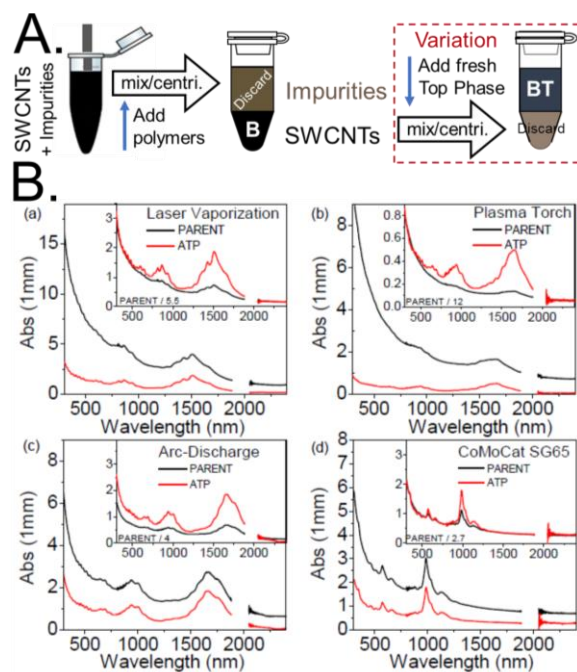
Figure 3. A. Schematic of SWCNT dispersion purification by ATPE as described by Subbaiyan et al. , 17 and with the variation of adding a second step to transfer the purified dispersion to a top phase for collection. For DOC dispersed SWCNT populations, the DOC concentration is reduced to a quantity that enables partition of many impurity types into the top phase, which can be discarded, while retaining the individualized SWCNTs in the bottom phase. In the variation including a second step, addition of SDS and reduction of the DOC concentration with addition of more top phase polymer, is specified to just at the condition needed to partition all SWCNT species to the top phase. Additional impurities will remain in the bottom phase if done correctly. B. Figures from Subbaiyan et al. 17 demonstrating the purification of SWCNT populations of several different average diameters that partition to the bottom phase relative to the original dispersion as shown by the reduction in absorbance that does not display the specific SWCNT optical transitions. Reprinted with permission from Springer Nature: Subbaiyan et al. Nano Res. 2015, 8 (5), 1755–1769. Copyright 2014.
