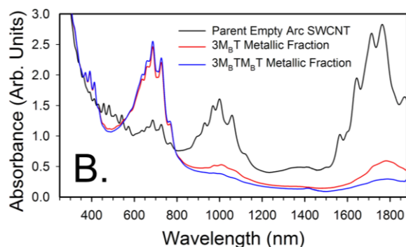
Figure 5. A. Schematic of additional workflow of ATPE separations for producing high purity metallic SWCNT populations starting at the 3M_B ( i.e. M_B M_B M_B ) phase of Figure 4. After separation of semiconducting SWCNTs to the top phase and their removal via pipetting, DOC is added to a concentration of 0.05 % in the bottom phase and mixed. After a waiting period of 30 min to 1 h, fresh top phase mimic containing DOC and SDS at a concentration just sufficient to partition all (n,m) species to the top phase is added, mixed and ATPE performed. The last step may need to be repeated on the resultant bottom fraction to collect all of the desirable SWCNTs. B. Scaled absorbance spectra of metallic-enriched empty arc SWCNTs separated in the manner of workflow in A. compared to the parent dispersion. The workflow of A. results in a purer metallic population than achieved without use of DOC; a repetition of the separation further increases metallic purity. Also shown is the effect of re-semiconducting metallic sorting the DOC-transferred top fraction, followed by a repetition of the workflow. This results in an even greater metallic purity with little recovery loss of the metallic population. Spectra are scaled to an absorbance of A = 5 arb. units at the \approx 240 nm peak for all samples.
