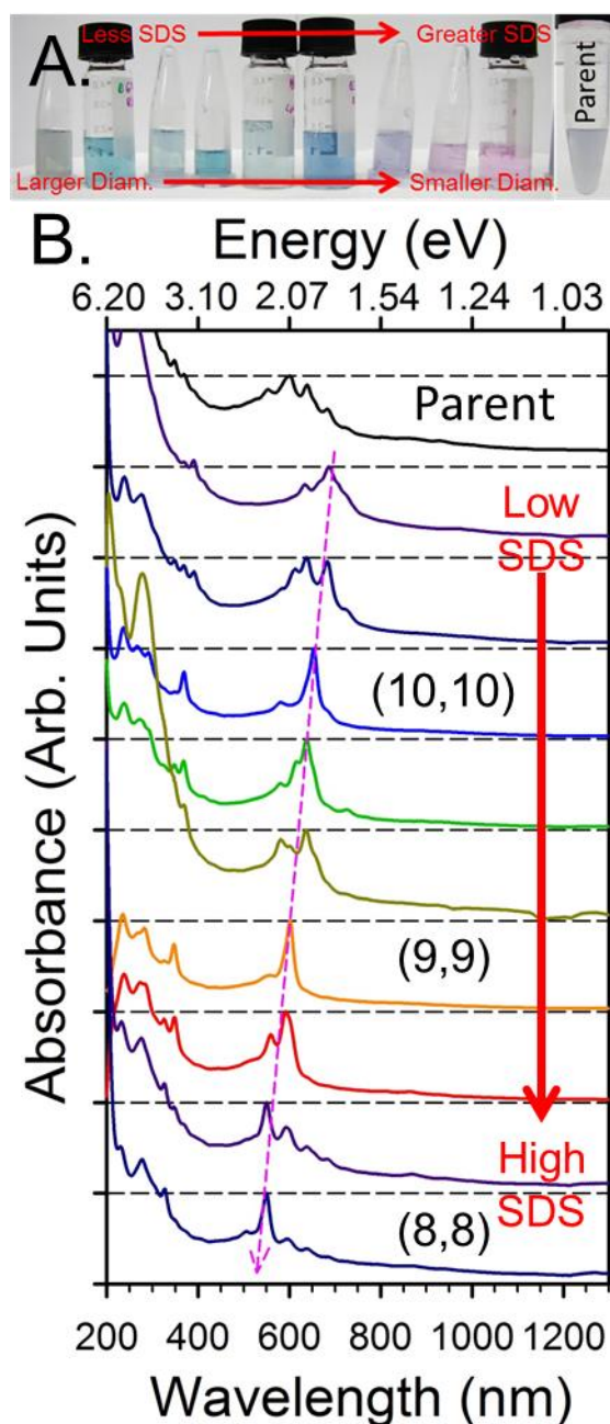
Figure 8. An example of fractions resulting from the gradient process ATPE separation of empty metallic PT SWCNTs adapted from Fagan et al. 19 A. Photographs of the SDS gradient ATPE separated diameter fractions in order from lowest SDS for extraction (left) to greatest SDS for extraction (right). B. Absorbance spectra of the fractions SWCNT fractions in order of their appearance in the photograph in panel A (left most = penultimate top), the topmost spectrum is of the metallic parent dispersion shown in A. The changes in the SWCNT species distribution from systematic ATPE separation are demonstrated by the changes in absorbance peak
