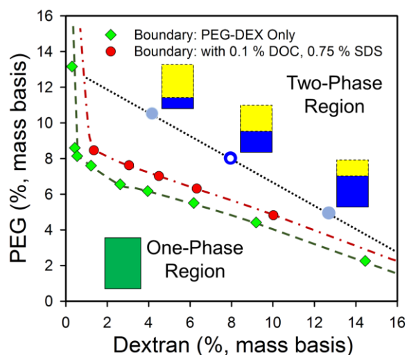
Figure 1. Phase diagram of a 6 kDa PEG and Dextran 70 ATPE system in water determined by the cloud point method 22 without (green diamond symbols) or in the presence of surfactants (red filled circles) at room temperature ( \approx 21^\circ\text{C} ). Compositions of PEG and DEX within the two-phase region, such as at the open blue circle, will at equilibrium form two phases at compositions located along the coexistence curve (dashed green eyeguide/dot-dash red eyeguide), and connected by a tie-line (black dotted eyeguide). In the PEG-Dextran ATPE system the upper phase is PEG-rich phase, and the lower phase is dextran-rich. All initial compositions along a tie-line produce identical composition of the two phases, but at different volume ratios due to mass conservation ( e.g. schematic volumes at the blue filled circles). The red circles report the coexistence curve, also called the binodal, of the polymers in the presence of 0.1 % (mass basis) DOC and 0.75 % (mass basis) SDS, which shifts the coexistence curve to slightly greater polymer mass fractions. Most conditions encountered in the use of surfactant-ATPE for SWCNTs will display similar coexistence curves.
