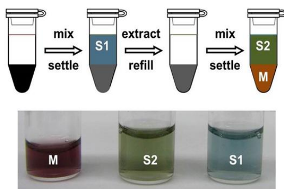
Figure 6. Top. Schematic of band gap fractionation of a SWCNT sample by sequential ATPE separations at successively reduced oxidant concentrations. Bottom. Photographs of separated fractions isolated from a small diameter SWCNT population. Adapted with permission from Gui et al. Nano Lett. 2015, 15 , 1642–1646. Copyright 2015 American Chemical Society.
