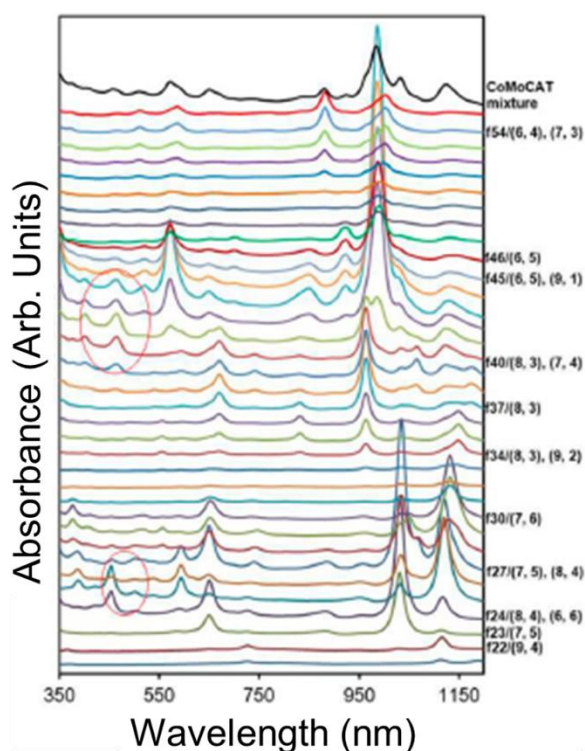
Figure 9. Absorbance spectra of sequential chromatographically-separated SWCNT populations using a CCC instrument. The emergence and disappearance of absorbance features is due to the differential partitioning of
