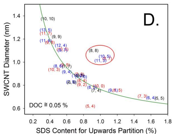
Figure 2. A. Schematic of a multistage ATPE separation. B. Schematic of the separation coefficient functionality for a semiconducting-metallic SWCNT separation at constant SC and oxidant (NaClO) concentration as a function of SDS addition. C. Schematic of the separation coefficient functionality of different (n,m) SWCNTs for SDS/DOC competition separations as a function of SDS concentration for constant DOC. At the SDS concentration shown by the red (dashed) vertical line, approximately all of the (8,6), (9,4), (6,6) and most of the (7,5) would partition to the top phase, with the other shown species partitioning to the bottom phase. D. Points showing the approximate SDS concentration required to partition the labelled species into the top phase of the PEG 6 kDa:DEX 70 ATPE system at \approx 20^\circ\text{C} and a DOC concentration of 0.05 %. The data quality was insufficient to discriminate enantiomers. Adapted from Fagan et al. 19 ACS Nano , 2015 , 9, 5377–5390.
