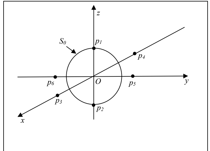
Figure 9. Construction of an example case with only two contact points for an optimal sphere. Moving the center from the origin results in a greater objective function for the data points shown.
