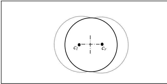
Figure 4. The constrained (inscribed) least-squares circle (shown solid) does not suffer from the instability seen for the maximum inscribed case.
