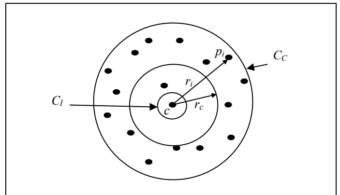
Figure 5. An example set of points and concentric circles for Lemmas 1a, b. The value of the objective function can be improved if the inscribed circle C_l (or the circumscribed circle C_c ) does not contact a data point.
