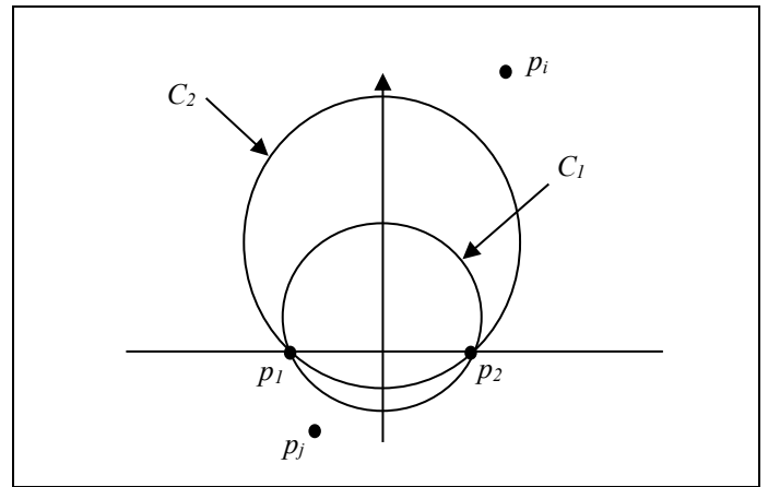
Figure 10. A one-parameter family of inscribing circles having a common chord. The search space for an optimal solution could be reduced by searching along the perpendicular bisector of a common chord.
