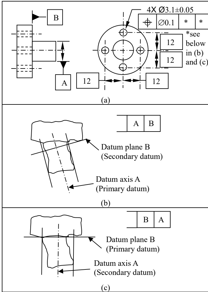
Figure 2. A simple example of (a) specification during design of a part, and (b, c) establishment of systems of primary and secondary datums involving cylindrical features on manufactured instances of the part.
