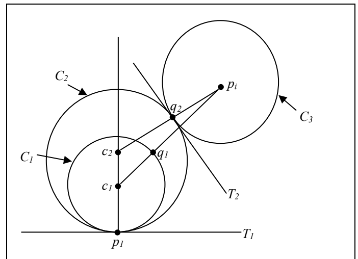
Figure 6. Construction for the proof of Theorem 1a. Growing the inscribing circle from C_1 to C_2 causes the distance from a data point p_i to C_2 to be less than the distance from p_i to C_1 .
