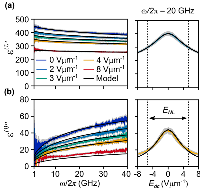
FIG. 7. Linear permittivity, \hat{\epsilon}^{(1)} = \epsilon_1' - i\epsilon_1'' as a function of frequency, and as a function of bias electric field at 20 GHz. An interval of width E_{NL} centered around E_{dc} = 0 Vm ^{-1} is indicated. The error bars (gray) are the 95% confidence interval from the standard error of the mean. a) The real part, \epsilon_1' . b) The imaginary part, \epsilon_1'' .
