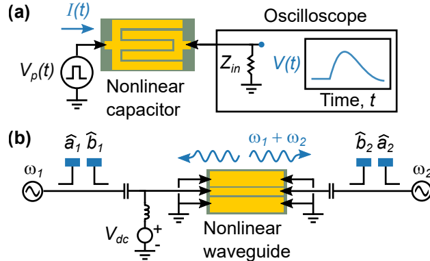
FIG. 1. Schematic picture of nonlinear measurements of thin films. a) In time-domain measurements, tuning dynamics are characterized by applying a voltage pulse V_p(t) to a capacitor and measuring the current I(t) = V(t)/Z_{in} that flows as the capacitor charges. This current is related to the change of the polarization with respect to time. b) We characterize tuning dynamics by exciting a waveguide patterned on a nonlinear material with two microwave frequencies \omega_1 and \omega_2 , and measuring the waves generated by nonlinear mixing. The complex amplitudes \hat{a} and \hat{b} correspond to the forward (towards the sample) and backward (from the sample) traveling waves, respectively. This method can be extended to much higher frequencies than time-domain measurements.
