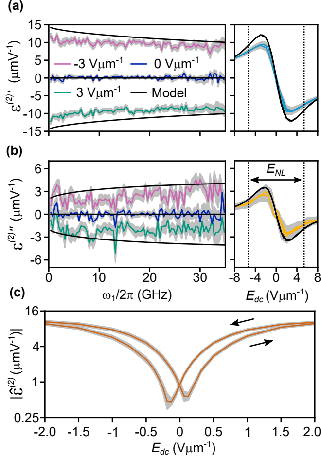
FIG. 8. The 2nd order nonlinear permittivity, \hat{\varepsilon}^{(2)} = \varepsilon^{(2)'} - i\varepsilon^{(2)''} , inferred from the \omega_1 + \omega_2 mixing product. In the frequency-dependent measurements, we varied the angular frequency of one of the stimulus signals, \omega_1 , while the other stimulus frequency, \omega_2 , was held constant at 2\pi \times 5 GHz. In our bias-swept measurements we set \omega_1 = 2\pi \times 7.84 GHz and \omega_2 = 2\pi \times 7.76 GHz. To facilitate comparison to Figure 7, we indicate an interval of width E_{NL} centered around the E_{dc} = 0 V \mu\text{m}^{-1} . The error bars (gray) are the 95% confidence interval from the standard error of the mean. a) The real part, \varepsilon_2' . b) The imaginary part, \varepsilon_2'' . c) The absolute value of \hat{\varepsilon}^{(2)} near 0 V.
