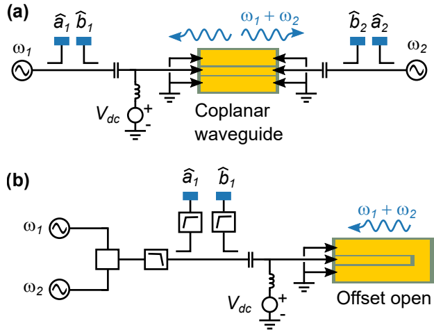
FIG. 4. Measurement configurations. a) For broadband measurements, we used coplanar waveguides, and excited the waveguide from both edges. b) For narrow-band measurements, we used a one-port configuration, with waveguides terminated by a gap to ground. This allowed us to use filters to minimize spurious signals generated within the LSNA.
