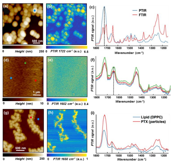
Fig. 2 (a) AFM topography map, and (b) PTIR map ( 1722\text{ cm}^{-1} , carboxylic acid stretching) of paclitaxel microcrystals. (c) Comparison between macroscale FTIR (red) and nanoscale PTIR spectra [blue, from marked position in panel (a)] of paclitaxel microcrystals, showing good agreement. (d) AFM topography map, (e) PTIR map ( 1652\text{ cm}^{-1} , paclitaxel amide I), and (f) PTIR spectra [from the color-coded positions in panel (d)] of a paclitaxel loaded PBD-b-PEO film highlighting the film homogeneity. (g) AFM topography map, (h) PTIR map ( 1650\text{ cm}^{-1} , paclitaxel amide I) and (i) PTIR spectra [from the color-coded positions in panel (g)] of a paclitaxel loaded DPPC film showing the partial segregation of paclitaxel nanocrystals from the DPPC film.
