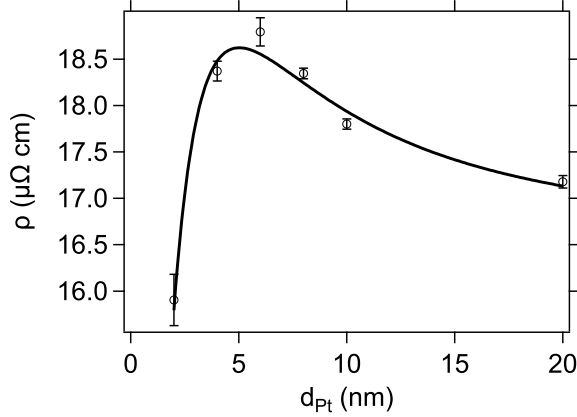
Figure 9. Thickness-dependent resistivity, measured for substrate/Ta(1.5)/Py(3.5)/Pt( d_{\text{Pt}} )/Ta(3) as a function of Pt thickness.
