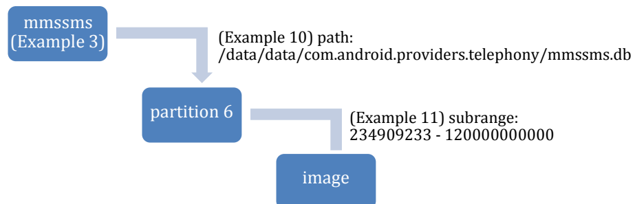
Figure 2. Schematic example of multiple relationships in CASE, depicting the sample JSON in Examples 10 and 11
