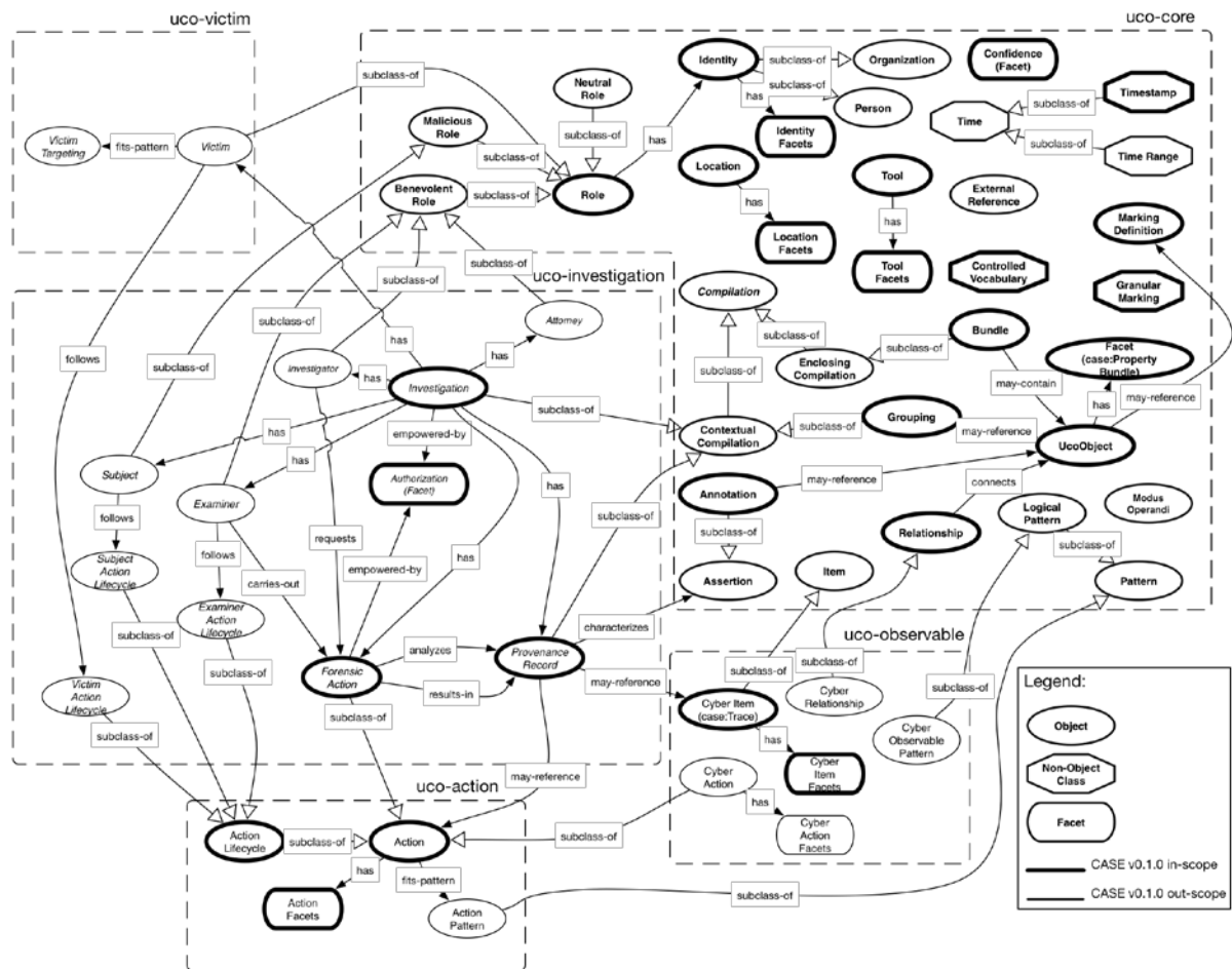
Figure 1. UCO v0.1.0/CASE v0.1.0 Overview. All items shown are elements of UCO v0.1.0. Items with bold outline are elements of CASE v0.1.0.
