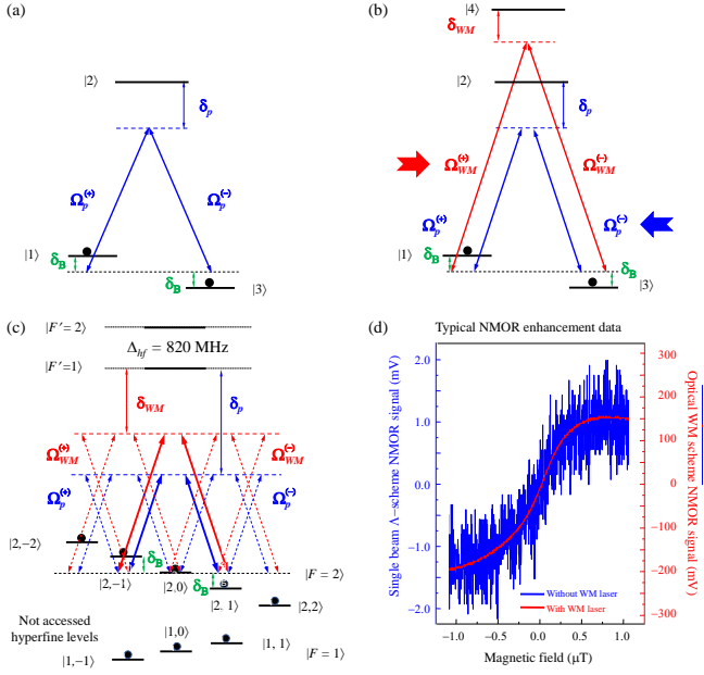
FIG. 1. Simplified models, actual atomic system, and experimental observations. (a) Simplified \Lambda -scheme used in conventional single beam atomic magnetometers. The lower two states are the m_F = \pm 1 hyperfine states of a generic F = 1 manifold (the m_F = 0 state is not shown). \Omega_p^{(\pm)} represents \sigma^{(\pm)} components of a linearly-polarized probe field. (b) Simplified wave mixing scheme where the inelastic scattering from the wave-mixing (WM) field to the probe field is the underlying physical process. \Omega_{WM}^{(\pm)} represents \sigma^{(\pm)} components of the linearly-polarized wave-mixing (WM) field. (c) Actual experimental system (magnetic sub-levels in the excited states are omitted) where the thick arrows depict the part that corresponds to (b). (d) Typical experimental data showing a 150-fold NMOR optical SNR enhancement (see Supplementary Information).
