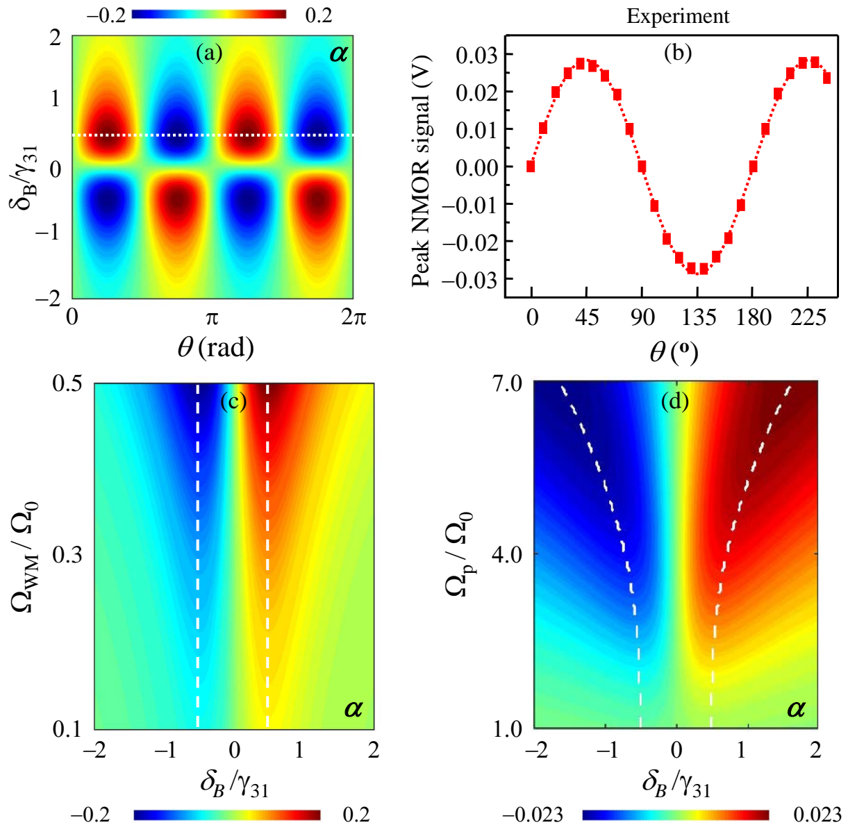
FIG. 4. Polarization angular dependence of NMOR and the magnetic resonance linewidth preserving effect. (a) Calculated probe field NMOR angle \alpha as a function of the normalized Zeeman frequency shift \delta_B/\gamma_{31} and the angle \theta between the polarizations of the probe and WM fields at Z/L = 1 . The white dotted-line indicates the sinusoidal oscillation at \delta_B/\gamma_{31} = 0.5 . (b) The experimental NMOR peak signal (solid squares) plotted as a function of the angle \theta between the polarization directions of the WM and the probe field. The axial magnetic field is 10 nT. The red dotted line is a sine curve fit to the data. (c) and (d): Calculated power broadening of the magnetic resonance for the optical WM method (c) and the conventional single-beam \Lambda method (d) as a function of the normalized WM and probe Rabi frequencies and the Zeeman shift (here, Rabi frequencies are normalized with respect to \Omega_0 = 2\pi \times 200 kHz). White dashed lines indicate the peaks of the NMOR signal. No magnetic resonance broadening can be seen in the WM method, (c) whereas the power broadening of the NMOR signal is significant in the conventional single-beam \Lambda method (d) even though the NMOR signal amplitude is still substantially less than that in (c), see color scales). Parameters are the same as in Fig. 2.
