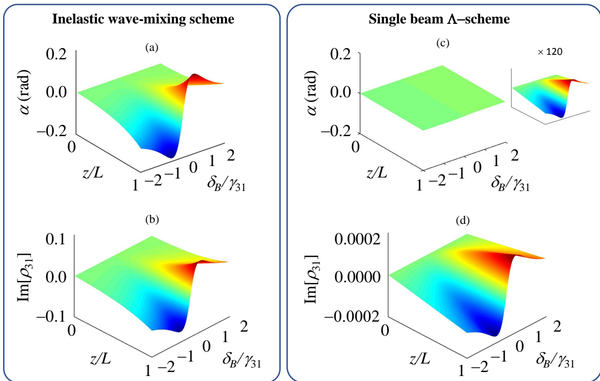
FIG. 3. Probe polarization rotation and ground state Zeeman coherence: Probe polarization rotation \alpha and the imaginary part of the ground state Zeeman coherence \text{Im}[\rho_{31}] as functions of the normalized Zeeman shift \delta_B/\gamma_{31} and propagation distance z/L . The inset in the upper-right plot shows the actual line shapes of the magnetic resonance of the conventional single-beam \Lambda method after 120-fold enlargement of the vertical axis. Notice that the resonance line shapes are identical to that of the optical WM method (upper-left panel), indicating the magnetic-field-sensitivity-preserving feature of the optical WM method. The imaginary part of the ground state Zeeman coherence \rho_{31} exhibits nonlinear(left)/linear(right) growth characteristics in the WM/single-beam scheme, indicating large energy transfer in a deep-inelastic scattering process.
