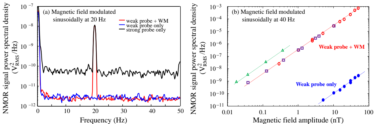
FIG. 2. NMOR optical signal power spectral density and peak NMOR signal power spectral density vs. magnetic field amplitude at 311 K. (a) A 10 nT magnetic field is modulated sinusoidally at 20 Hz. Blue: single beam \Lambda technique with a probe field intensity I_p = 16.8 \mu\text{W}/\text{cm}^2 . Red: optical WM technique with I_p = 16.8 \mu\text{W}/\text{cm}^2 and a WM field intensity I_{WM} = 15 \mu\text{W}/\text{cm}^2 . Black: single beam \Lambda technique with a probe field intensity I_p = 2.6 \text{ mW}/\text{cm}^2 . (b) NMOR optical power spectral density as a function of magnetic field amplitude. Blue dots: single beam \Lambda technique, I_p = 650 \mu\text{W}/\text{cm}^2 . Red open-circle and purple squares: optical WM technique with I_p = 650 \mu\text{W}/\text{cm}^2 and I_{WM} = 60 \mu\text{W}/\text{cm}^2 . Green triangle: WM technique, but with I_p = 1.3 \text{ mW}/\text{cm}^2 . Notice the more than 300,000-fold optical signal power spectral density enhancement achieved with the optical WM technique in both plots.
