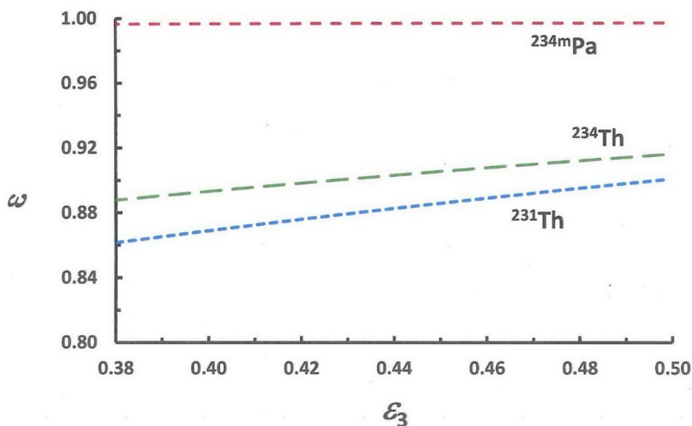
Fig. 6. Computed LS detection efficiencies \epsilon for the uranium-isotope daughters, ^{234\text{m}}\text{Pa} , ^{234}\text{Th} , and ^{231}\text{Th} , as a function of the efficiency for ^3\text{H} as obtained with the MICELLE2 code.
