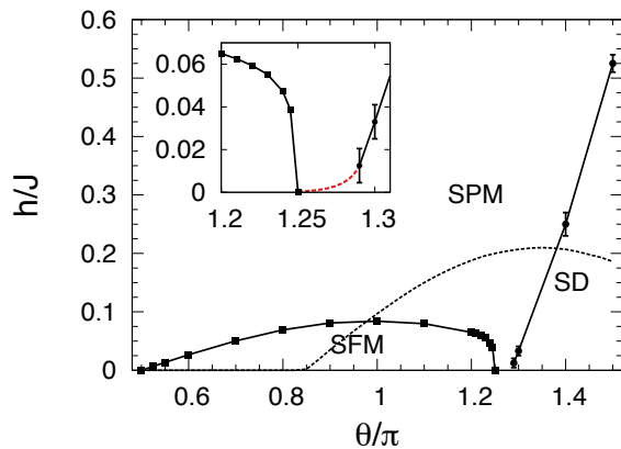
FIG. 13. Phase diagram as a function of h and \theta for a fixed pitch \eta = 0.1\pi extracted from the DMRG calculations. The dashed line marks the classical SFM phase boundary, which completely misses the dimerized phase and underestimates the stability of the SFM for positive \tilde{K} . Error bars are determined based on the spread of the crossing in the corresponding correlation length (the error bars for SFM-to-SPM are smaller than the symbol). (Inset) Zoomed in on the region near \theta = 1.25\pi , here we have added a schematic dashed red line, where we expect the critical field is exponentially small.
