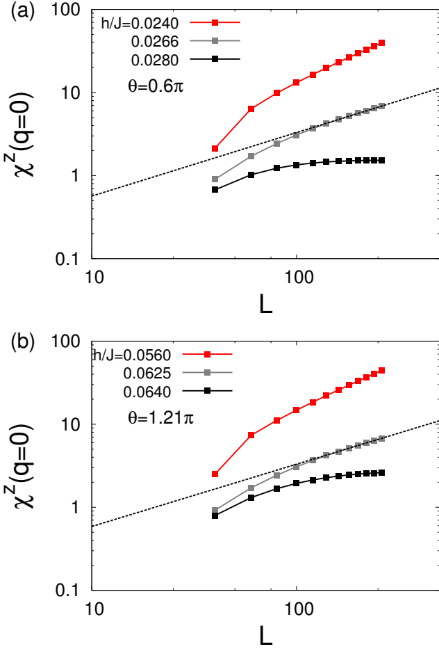
FIG. 5. Spin susceptibility as a function of system size L and magnetic field h for \theta = 0.6\pi (a) and \theta = 1.21\pi (b). In the SFM phase \chi^z(0) \sim L (red) and in the SPM \chi^z(0) \sim \text{const.} (black). At the critical point the spin susceptibility diverges with L like \chi^z(0) \sim L^{\gamma/\nu} (grey) and using the value of \nu found in Fig. 4, we find \gamma = 0.52(4) and 0.50(4) for \theta = 0.6\pi and 1.21\pi respectively.
