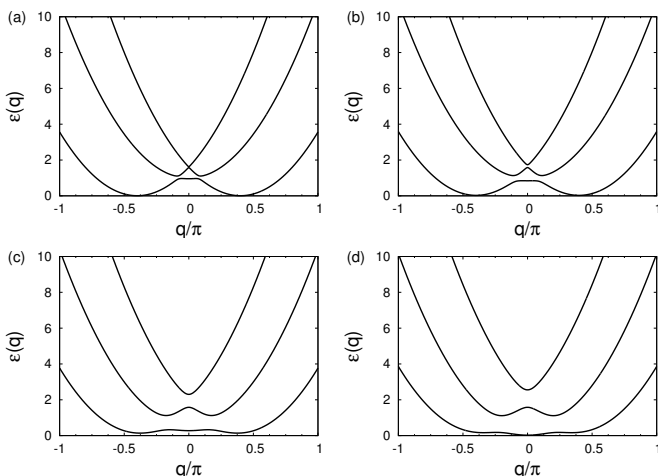
FIG. 8. Dispersion from Landau theory truncating the effective action in Eq. (26) to quadratic order. As a prototypical example, we take r_0/K = -0.5 , u_0/K = 0.2 , and \eta = 0.4\pi , which has a critical field h_c/K = 3.53 . Evolution of the spin wave dispersion as a function of increasing magnetic field h/K = 0.5 (a), h/K = 1.0 (b), h/K = 2.5 (c) and h/K = 3.0 (d).
