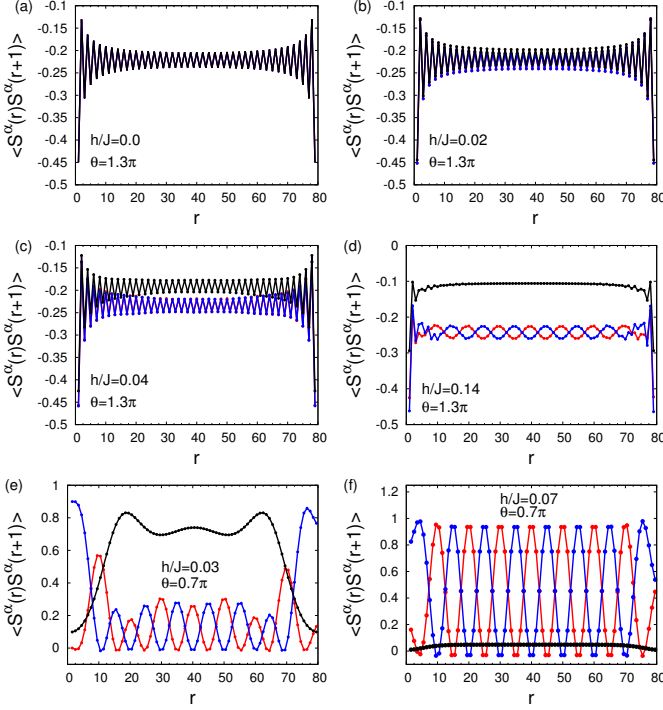
FIG. 9. Average nearest neighbor spin product along the chain for \theta = 1.3\pi and L = 80 in the SD phase (a), (b), (c), in the SPM phase for \theta > 1.25\pi (d). In contrast, for \theta < 1.25\pi (e) is in the SFM phase and (f) is in the SPM phase. We find the effect of the magnetic field in the SD phase is to break the spin symmetry between the x (red), y (blue), and z (black) components of the spin. For large fields in the SPM phase the translational symmetry is restored and the value of \theta dictates the sign of the spin product.
