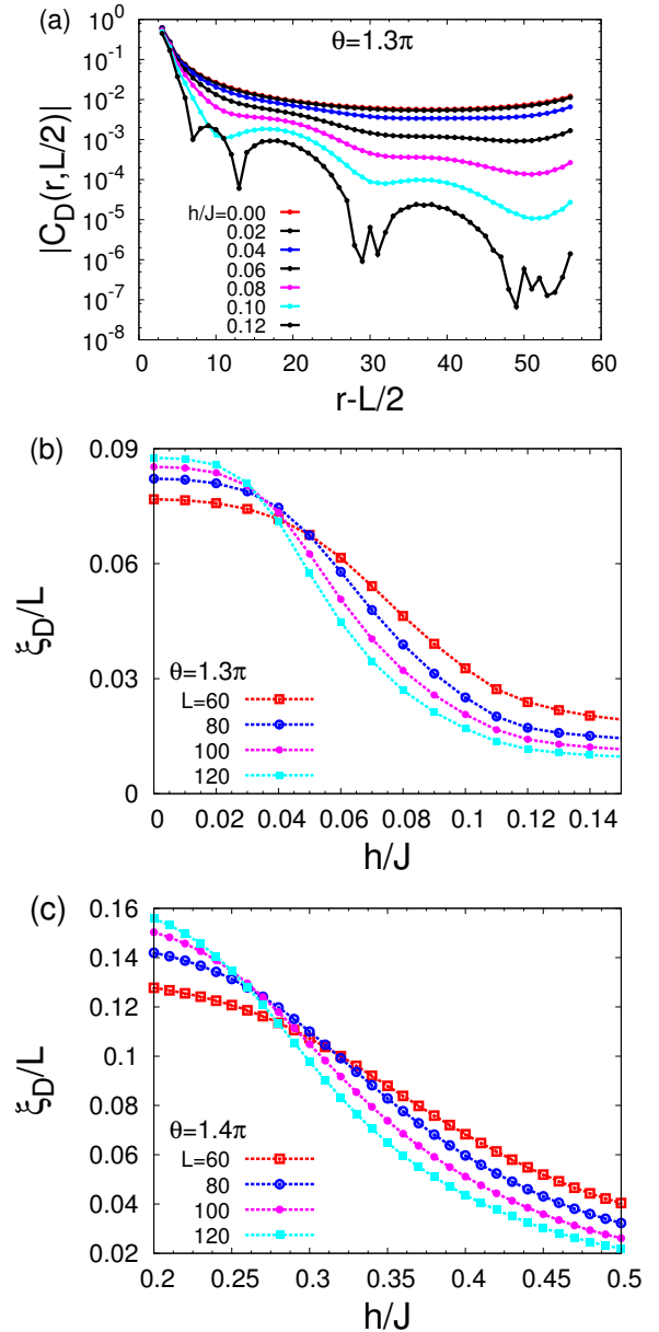
FIG. 12. Dimer correlations for \theta = 1.3\pi and M = 225 . (a) Dimer correlation function measured from the center of the chain ( r' = L/2 ) for various values of the spiral magnetic field and a system size L = 120 . For small fields in the SD phase C_D(r, L/2) saturates to a constant at large r , where as in the SPM phase it goes to zero. The dimer correlation length [from C_D(r, L/2) in Eq. (17)] as a function of the magnetic field for various system sizes for \theta = 1.3\pi (b) and \theta = 1.4\pi (c). The crossing of \xi_D/L estimates the location of the quantum phase transition into the SPM phase, here we find h_c(\theta = 1.3\pi)/J = 0.033(8) and h_c(\theta = 1.4\pi)/J = 0.25(2) . The drift in the crossing with L implies large corrections to finite size scaling.
