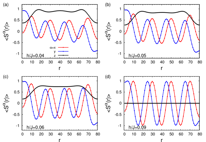
FIG. 2. Average spin along the chain in the SFM (a), (b), and (c), as well as the SPM (d) phase computed using DMRG with chain length L = 80 , bond dimension M = 50 , and \theta = 1.1\pi . For a pitch \eta = \pi/10 the spiral is commensurate with L and there are large finite size effects for small h near the chain boundaries, we have also confirmed this behavior in the classical model [see Figs. 6 (a) and (b)]. Away from the chain boundaries we find \langle S^x(r) \rangle \propto \cos(\eta r) and \langle S^y(r) \rangle \propto \sin(\eta r) consistent with the Landau theory (see Sec. II C). For moderate fields the boundary effects are weak and \langle S^z(r) \rangle is roughly constant in the center of the chain. Crossing the critical field h_c(\theta = 1.1\pi)/J = 0.0798(3) we find M_z = 0 .
