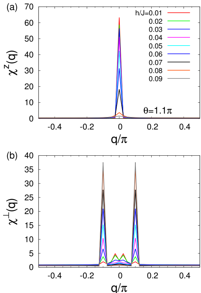
FIG. 3. Spin susceptibility computed from DMRG as a function of momentum q in the longitudinal (a) and transverse (b) directions with L = 80 , M = 50 , \theta = 1.1\pi , and the legend is shared across both figures. In the SFM phase \chi^z(q) is strongly peaked at q = 0 with a peak height monotonically decreasing with increasing h going to zero at h_c . The non-zero SOC produces peaks in \chi^\perp(q) at q = \pm\eta (= \pm 0.1\pi) and the peak continuously increases as a function of h .
