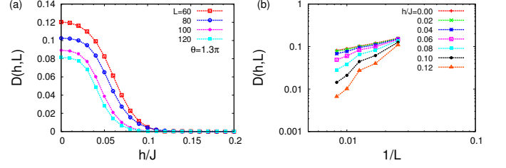
FIG. 11. Dimer order parameter defined in Eq. (27) for \theta = 1.3\pi as a function of h and L . D versus h for various L (a) and D versus L for various h (b). In the SD phase we find the dimer order parameter is saturating to a constant for large L and weak h . At large h , D goes to zero at large L , and we take an estimate for transition from the smallest value of h where D still seems to vanish at large L .
