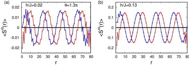
FIG. 10. Average spin along the chain for \theta = 1.3\pi in the SD phase (a) and in the SPM phase (b) for L = 80 and M = 200 and x (red), y (blue), and z (black) spin components. The dimerization is visible in the average spin in the SD phase, whereas for large fields the translational symmetry is restored in the SPM phase.
