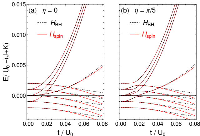
FIG. 1. Comparison of the low-energy eigenvalues of H_{\text{BH}} at unit filling with the spectrum of H_{\text{spin}} for two lattice sites, shown as a function of t/U_0 for (a) uniform field, and (b) SOC with pitch angle \eta = \pi/5 . In both cases we take h = 0.001U_0 and U_2 = -0.1U_0 . The spectra are indistinguishable for sufficiently small t/U_0 , and the SOC causes avoided level crossings in the spectrum in the regime t^2/U_0 \sim h . At larger t , as the spectra begin to differ quantitatively, the level ordering nonetheless remains identical.
