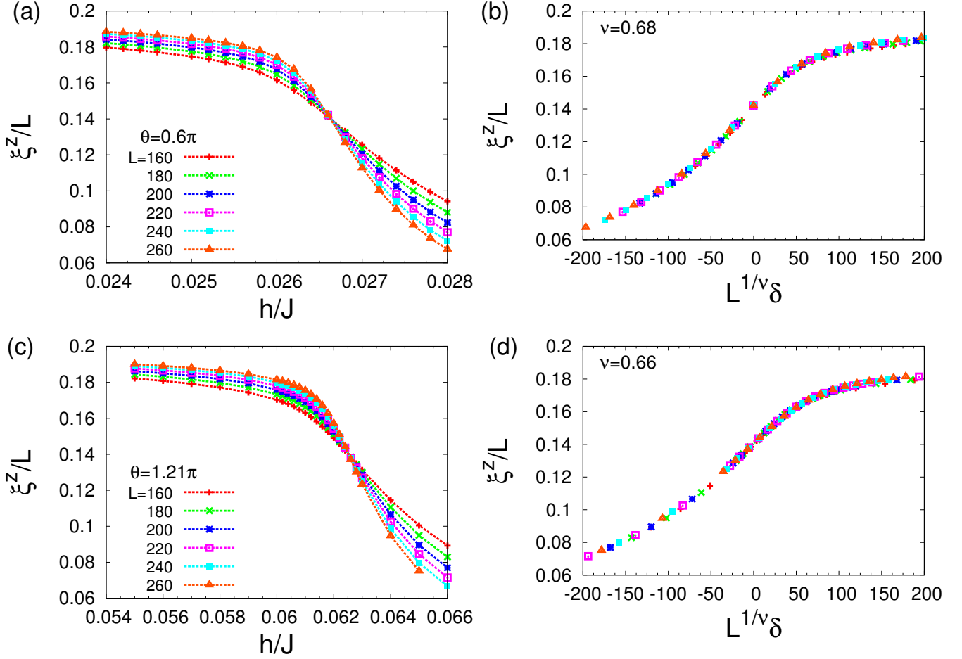
FIG. 4. Longitudinal correlation length \xi^z defined in Eq. (17) for various system sizes as a function of h for \theta = 0.6\pi (a) and (b) as well as \theta = 1.21\pi (c) and (d). We find a clear crossing in the data for \xi^z/L versus h for several L and take this location as an unbiased estimate of h_c , we find h_c(\theta = 0.6\pi) = 0.0266(2) and h_c(\theta = 1.21\pi) = 0.0625(3) . In the vicinity of the transition we perform finite size scaling from Eq. (18) and collapse the data in terms of L^{1/\nu}\delta and estimate the quality of collapse using a \chi^2 analysis [63]. We find \nu = 0.68(8) for \theta = 0.6\pi and \nu = 0.66(6) for \theta = 1.21\pi .
