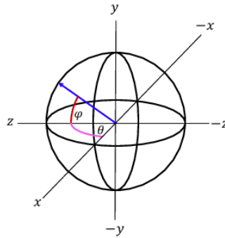
Fig. 2. Spherical coordinates of a unit vector.
