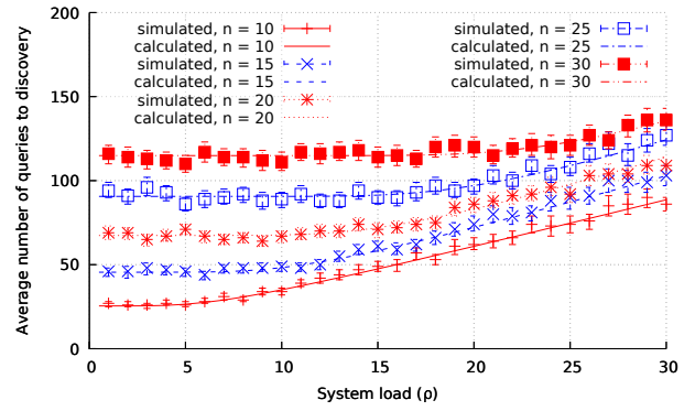
Fig. 1. Analytical results vs. simulation results for the random scheme
